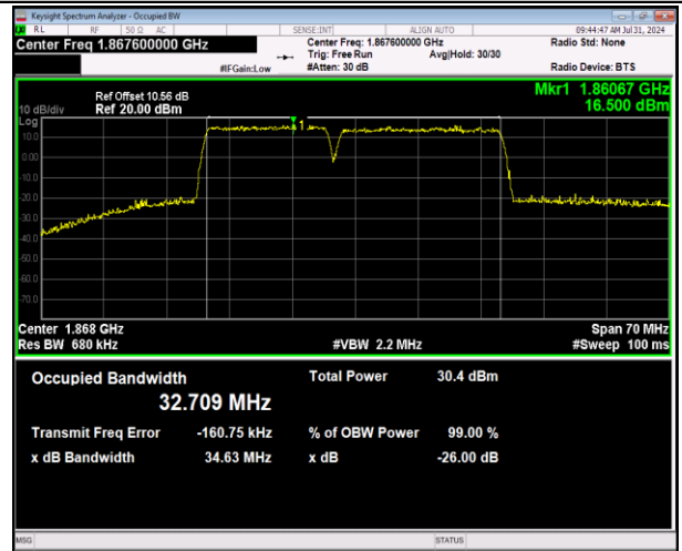
2-2-15MHz-20MHz-64QAM-64QAM-18678-18849-75RB #0-100RB#0-PASS
