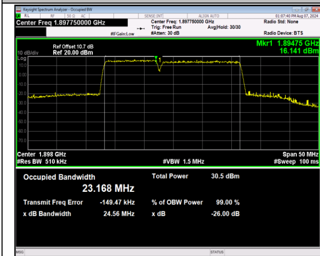
2-2-10MHz-15MHz-16QAM-16QAM-19005-19125-50RB#0-75RB#0-PASS
