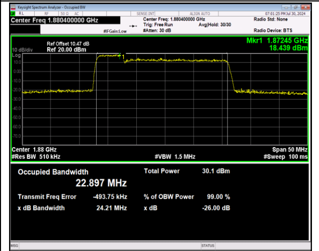
2-2-5MHz-20MHz-64QAM-64QAM-18808-18925-25RB#0-100RB#0-PASS
