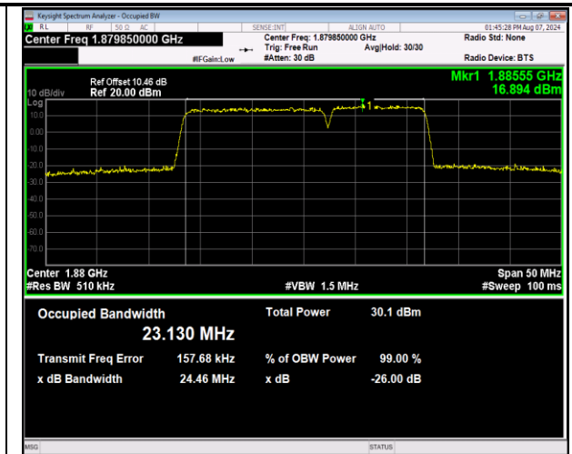
2-2-15MHz-10MHz-16QAM-16QAM-18851-18971-75RB #0-50RB#0-PASS
