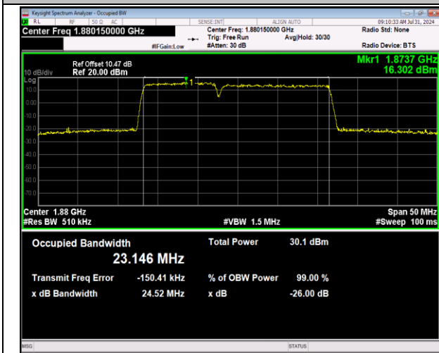
2-2-10MHz-15MHz-64QAM-64QAM-18829-18949-50RB#0-75RB#0-PASS
