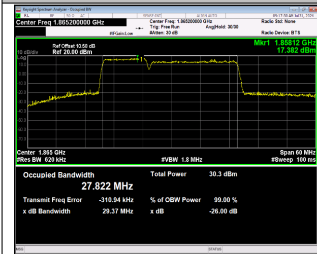
2-2-10MHz-20MHz-64QAM-64QAM-18655-18799-50RB# 0-100RB#0-PASS
