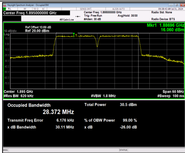
2-2-15MHz-15MHz-64QAM-64QAM-18975-19125-75RB# 0-75RB#0-PASS
