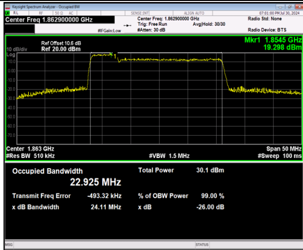
2-2-5MHz-20MHz-64QAM-64QAM-18633-18750-25RB#0-100RB#0-PASS
