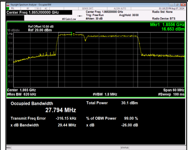
2-2-10MHz-20MHz-16QAM-16QAM-18655-18799-50RB #0-100RB#0-PASS
