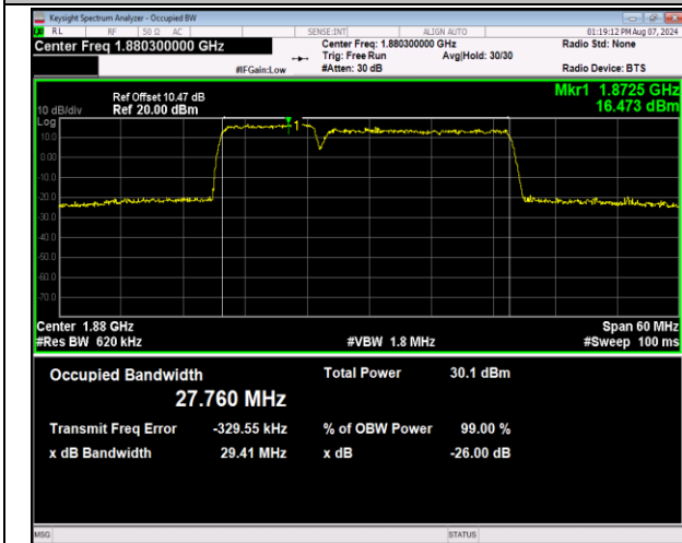
2-2-10MHz-20MHz-16QAM-16QAM-18806-18950-50RB# 0-100RB#0-PASS
