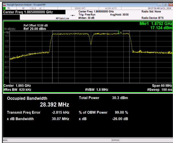
2-2-15MHz-15MHz-64QAM-64QAM-18675-18825-75RB# 0-75RB#0-PASS
