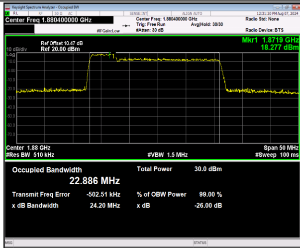
2-2-5MHz-20MHz-16QAM-16QAM-18808-18925-25RB#0-100RB#0-PASS
