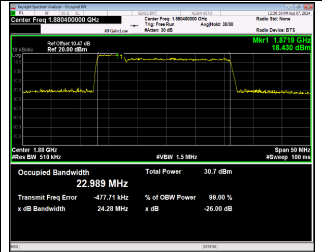
2-2-5MHz-20MHz-QPSK-QPSK-18808-18925-25RB#0-100RB#0-PASS
