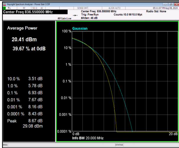
5-5-10MHz-10MHz-16QAM-16QAM-20476-20575-50RB#0
