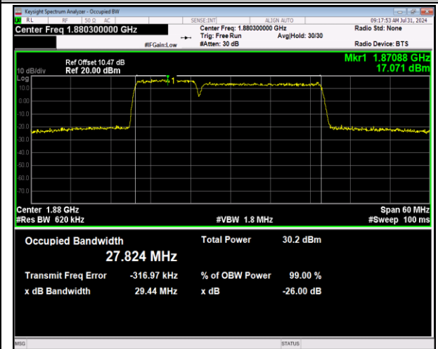
2-2-10MHz-20MHz-64QAM-64QAM-18806-18950-50RB #0-100RB#0-PASS
