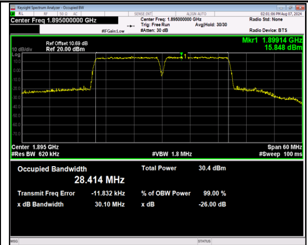
2-2-15MHz-15MHz-16QAM-16QAM-18975-19125-75RB #0-75RB#0-PASS
