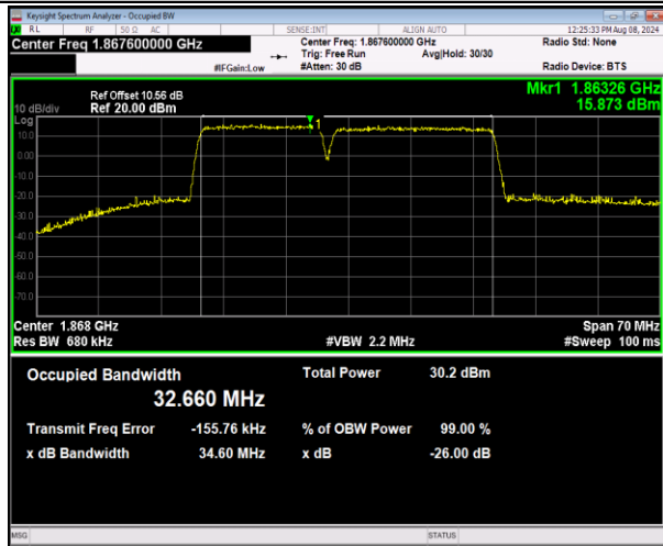
2-2-15MHz-20MHz-16QAM-16QAM-18678-18849-75RB# 0-100RB#0-PASS
