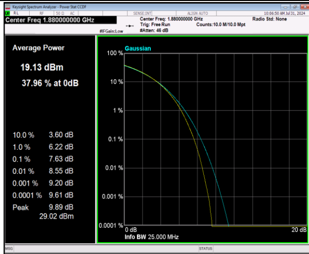
2-2-20MHz-20MHz-64QAM-64QAM-18801-18999-100RB#0 #0-100RB#0-PASS
