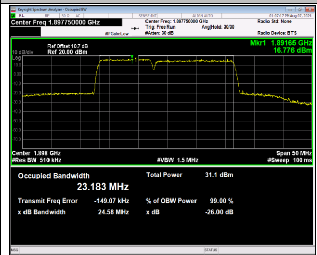
2-2-10MHz-15MHz-QPSK-QPSK-19005-19125-50RB#0-75RB#0-PASS
