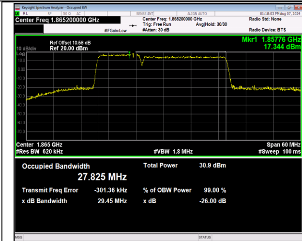
2-2-10MHz-20MHz-QPSK-QPSK-18655-18799-50RB#0-1 00RB#0-PASS
