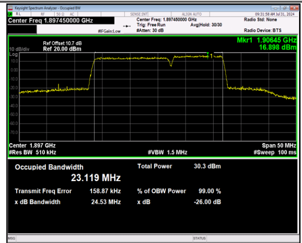
2-2-15MHz-10MHz-64QAM-64QAM-19027-19147-75RB #0-50RB#0-PASS
