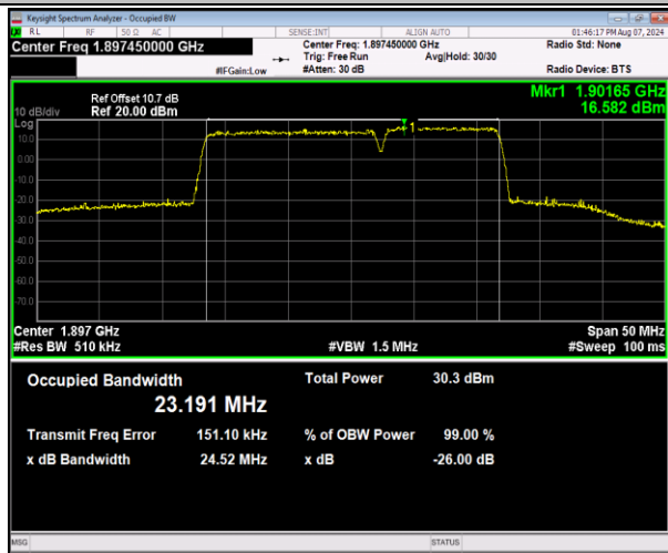
2-2-15MHz-10MHz-16QAM-16QAM-19027-19147-75RB# 0-50RB#0-PASS
