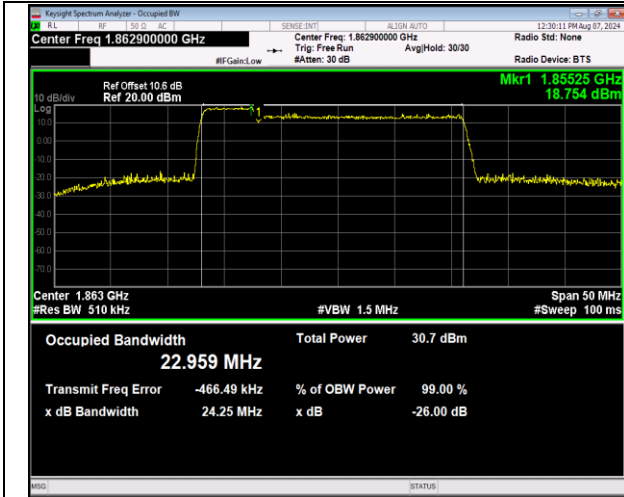
2-2-5MHz-20MHz-QPSK-QPSK-18633-18750-25RB#0-10 ORB#0-PASS
