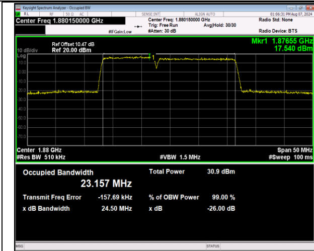
2-2-10MHz-15MHz-QPSK-QPSK-18829-18949-50RB#0-7 5RB#0-PASS
