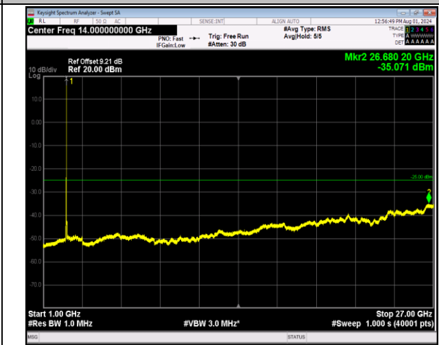
7-7-20MHz-20MHz-64QAM-64QAM-21152-21350-1RB#99-0RB#0-1000~27000MHz-PASS
