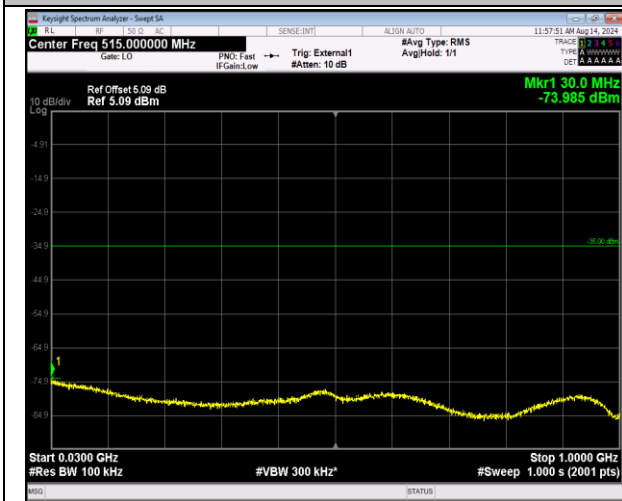
41-41-5MHz-20MHz-16QAM-16QAM-40273-40390-25RB# #0-100RB#0-30~1000MHz-PASS
