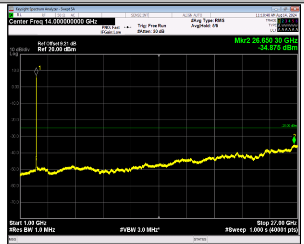
7-7-20MHz-20MHz-16QAM-16QAM-21001-21199-100RB#0 -100RB#0-1000~27000MHz-PASS
