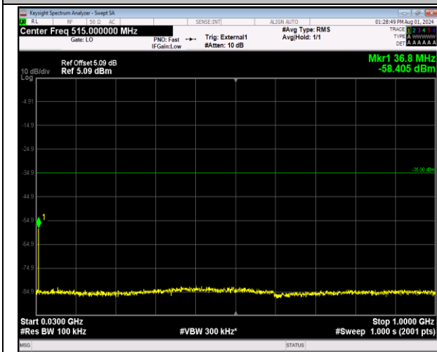
41-41-5MHz-20MHz-64QAM-64QAM-40648-40765-1RB# 24-0RB#0-30~1000MHz-PASS
