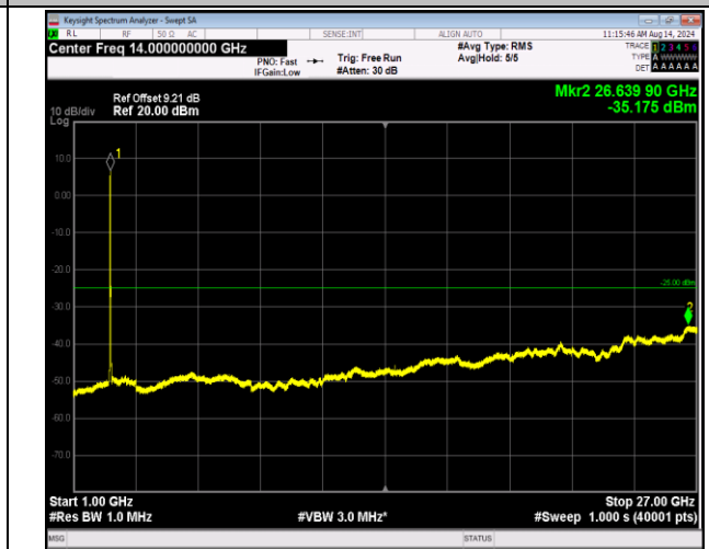
7-7-20MHz-20MHz-16QAM-16QAM-21152-21350-100RB#0 -100RB#0-1000~27000MHz-PASS
