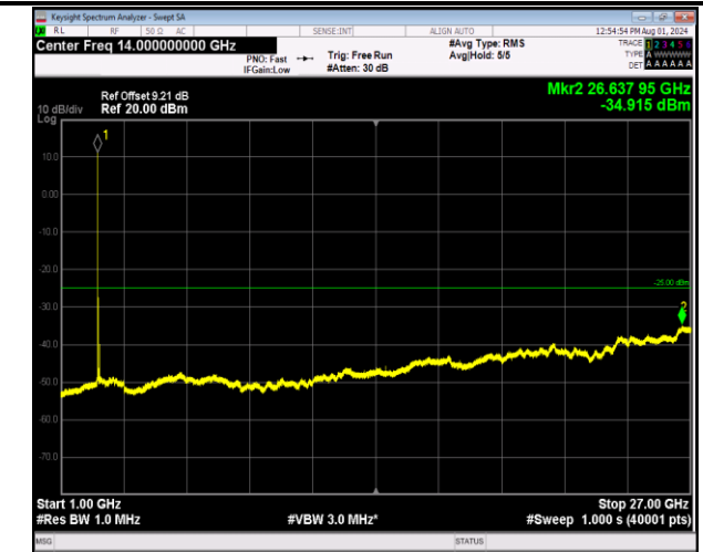
7-7-20MHz-20MHz-64QAM-64QAM-21001-21199-1RB#0-1 RB#99-1000~27000MHz-PASS
