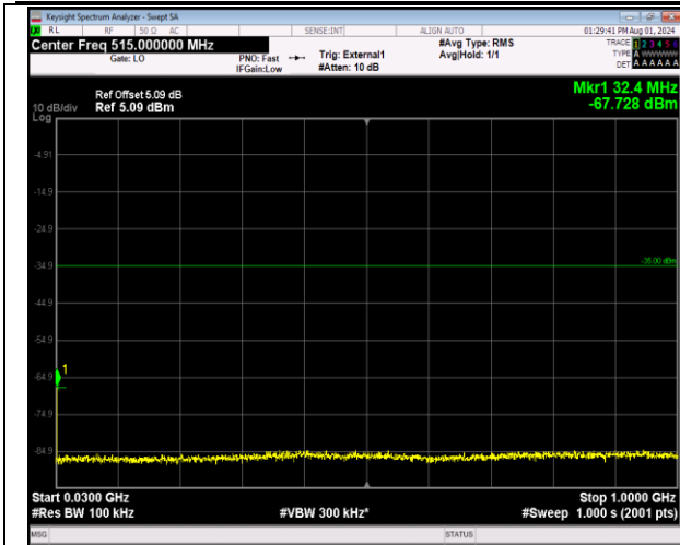
41-41-5MHz-20MHz-64QAM-64QAM-40648-40765-1RB# 0-1RB#99-30~1000MHz-PASS
