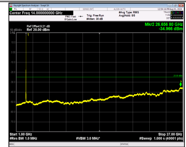
7-7-20MHz-20MHz-64QAM-64QAM-21001-21199-1RB#99-0RB#0-1000~27000MHz-PASS
