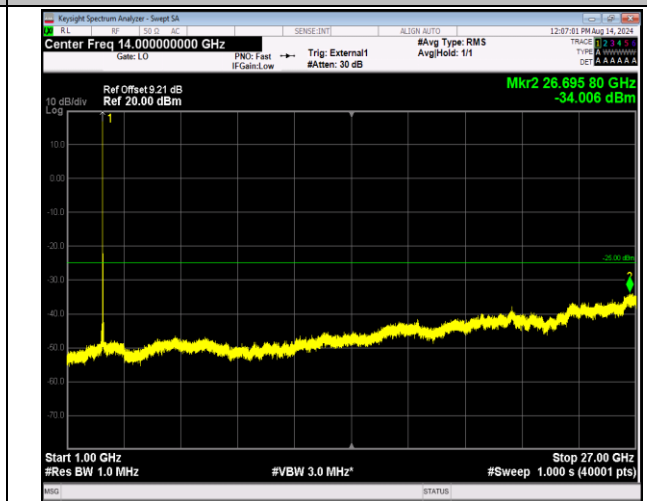
41-41-5MHz-20MHz-16QAM-16QAM-41023-41140-1RB#0- 0RB#0-1000~27000MHz-PASS
