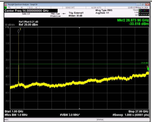
41-41-5MHz-20MHz-16QAM-16QAM-40648-40765-25RB#0 -100RB#0-1000~27000MHz-PASS
