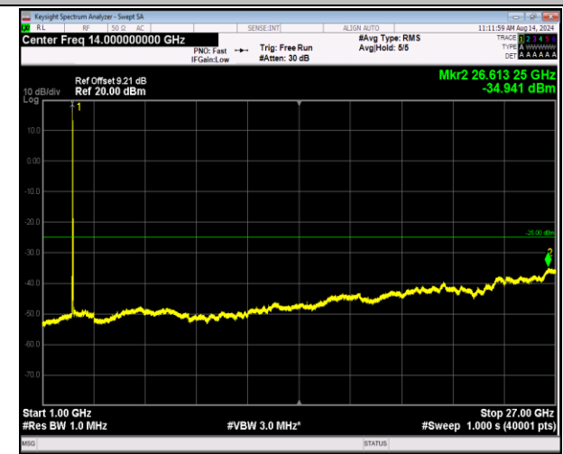
7-7-20MHz-20MHz-16QAM-16QAM-21152-21350-1RB#0-0 RB#0-1000~27000MHz-PASS
