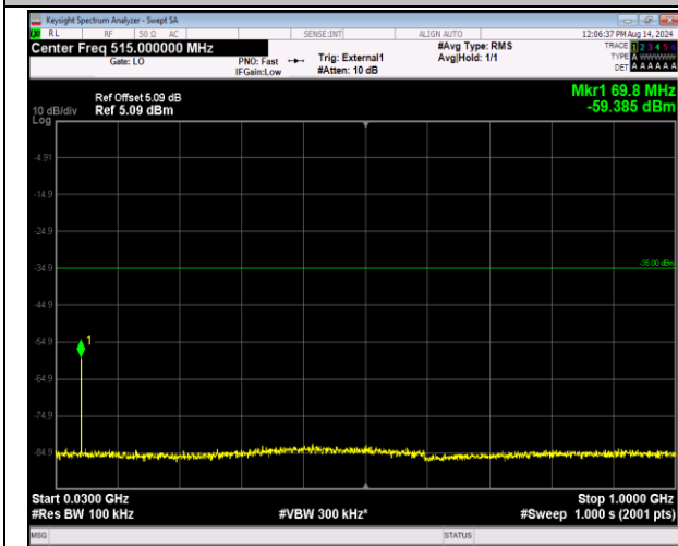
41-41-5MHz-20MHz-16QAM-16QAM-41023-41140-1RB# 0-0RB#0-30~1000MHz-PASS
