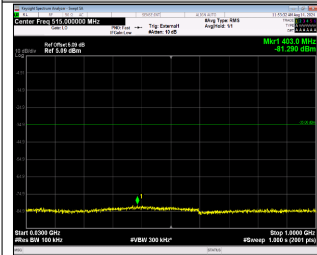
41-41-5MHz-20MHz-QPSK-QPSK-40273-40390-1RB#24-0RB#0-30~1000MHz-PASS
