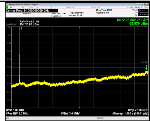
41-41-5MHz-20MHz-64QAM-64QAM-40273-40390-1RB#24 -0RB#0-1000~27000MHz-PASS
