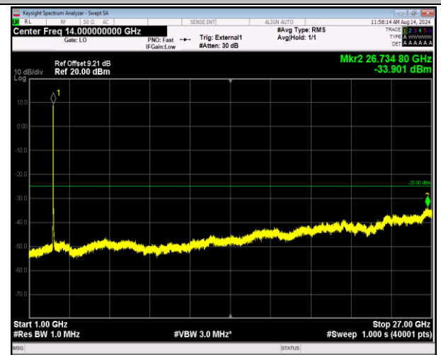
41-41-5MHz-20MHz-16QAM-16QAM-40273-40390-25RB#0 -100RB#0-1000~27000MHz-PASS
