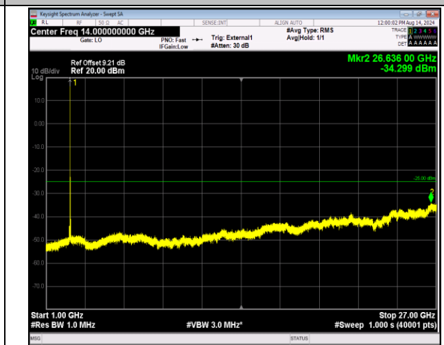
41-41-5MHz-20MHz-16QAM-16QAM-40648-40765-1RB#0- 0RB#0-1000~27000MHz-PASS
