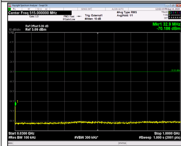
41-41-5MHz-20MHz-QPSK-QPSK-40648-40765-1RB#0-1RB#99-30~1000MHz-PASS
