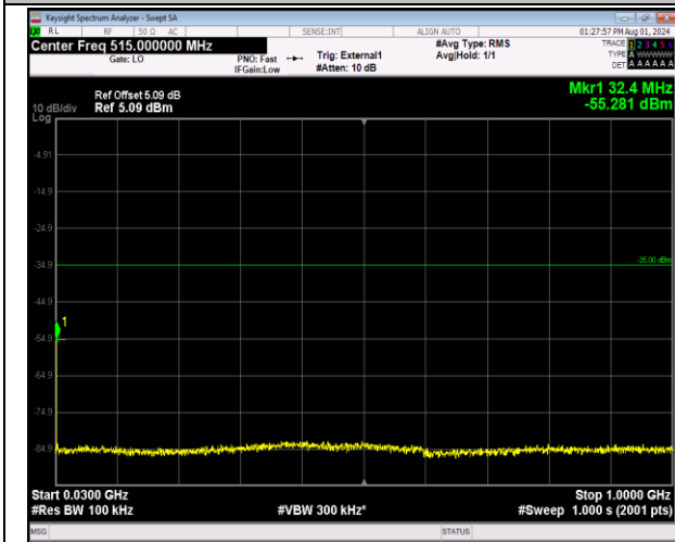
41-41-5MHz-20MHz-64QAM-64QAM-40648-40765-1RB# 0-ORB#0-30~1000MHz-PASS
