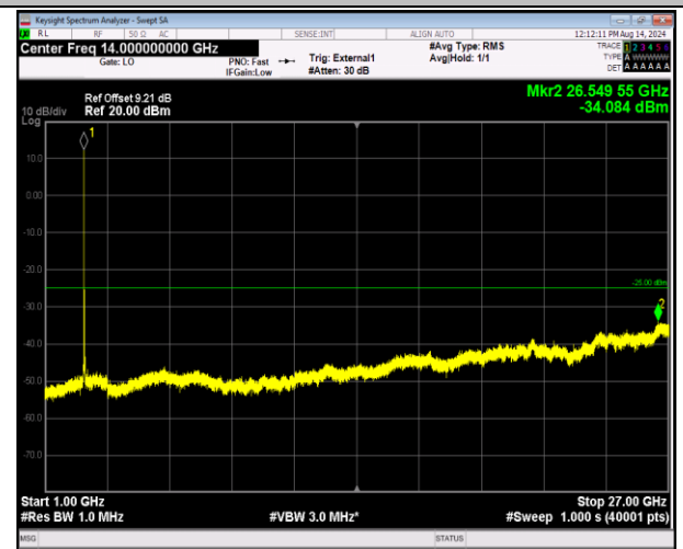
41-41-5MHz-20MHz-16QAM-16QAM-41023-41140-25RB#0 -100RB#0-1000~27000MHz-PASS
