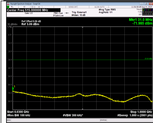
41-41-5MHz-20MHz-QPSK-QPSK-40273-40390-25RB#0 -100RB#0-30~1000MHz-PASS
