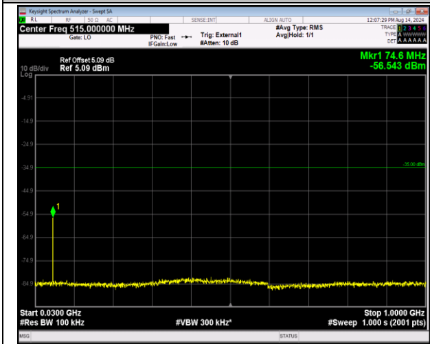
41-41-5MHz-20MHz-QPSK-QPSK-41023-41140-1RB#24-0RB#0-30~1000MHz-PASS
