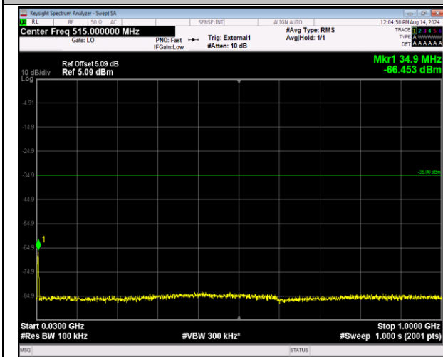
41-41-5MHz-20MHz-16QAM-16QAM-40648-40765-25RB# #0-100RB#0-30~1000MHz-PASS
