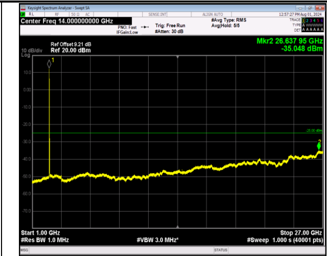
7-7-20MHz-20MHz-64QAM-64QAM-21152-21350-1RB#0-1 RB#99-1000~27000MHz-PASS
