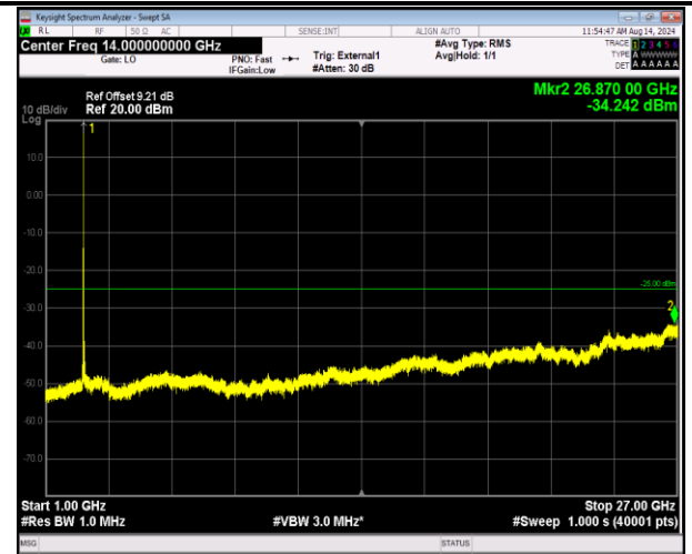
41-41-5MHz-20MHz-16QAM-16QAM-40273-40390-1RB#24 -ORB#0-1000~27000MHz-PASS
