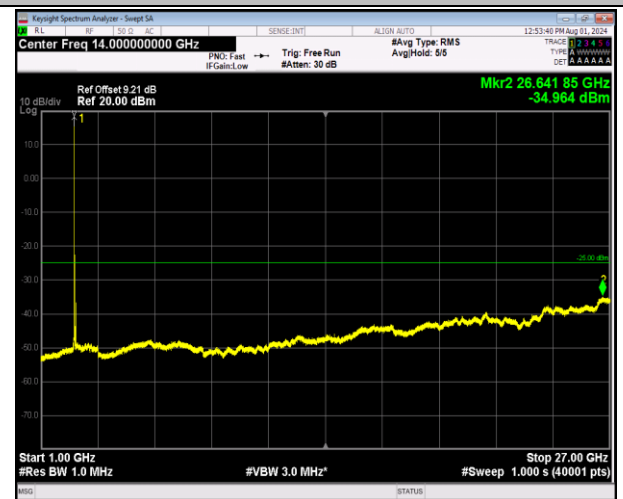
7-7-20MHz-20MHz-64QAM-64QAM-21001-21199-1RB#0- RB#0-1000~27000MHz-PASS
