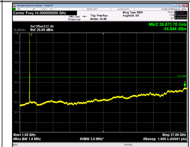
7-7-20MHz-20MHz-64QAM-64QAM-21152-21350-1RB#0- ORB#0-1000~27000MHz-PASS
