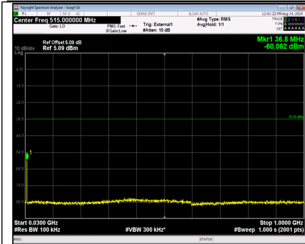
41-41-5MHz-20MHz-16QAM-16QAM-40648-40765-1RB# 24-ORB#0-30~1000MHz-PASS
