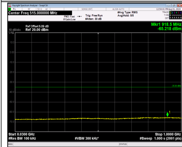
7-7-20MHz-20MHz-64QAM-64QAM-21001-21199-1RB#9 9-0RB#0-30~1000MHz-PASS
