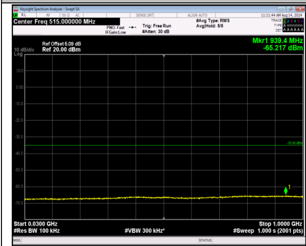
7-7-20MHz-20MHz-16QAM-16QAM-21152-21350-1RB#0 -0RB#0-30~1000MHz-PASS
