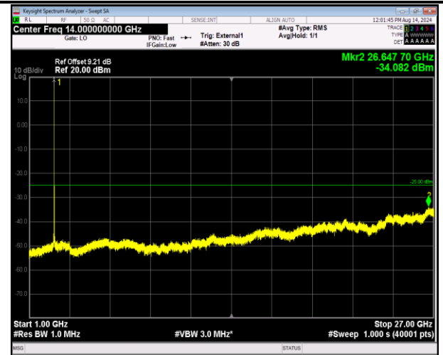
41-41-5MHz-20MHz-16QAM-16QAM-40648-40765-1RB#24 -ORB#0-1000~27000MHz-PASS
