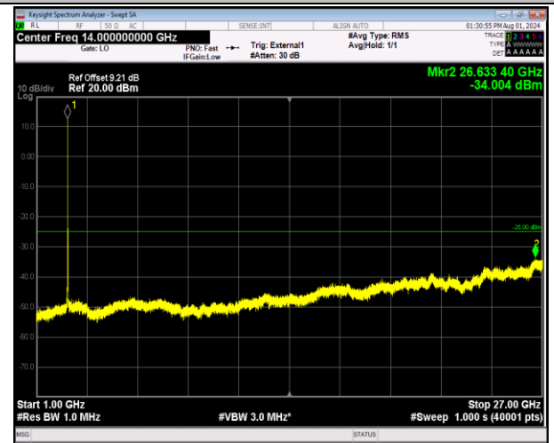
41-41-5MHz-20MHz-64QAM-64QAM-40648-40765-25RB#0 -100RB#0-1000~27000MHz-PASS
