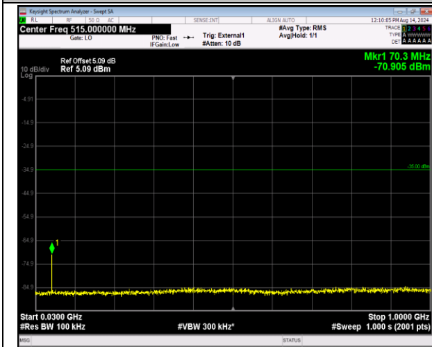
41-41-5MHz-20MHz-16QAM-16QAM-41023-41140-1RB# 0-1RB#99-30~1000MHz-PASS
