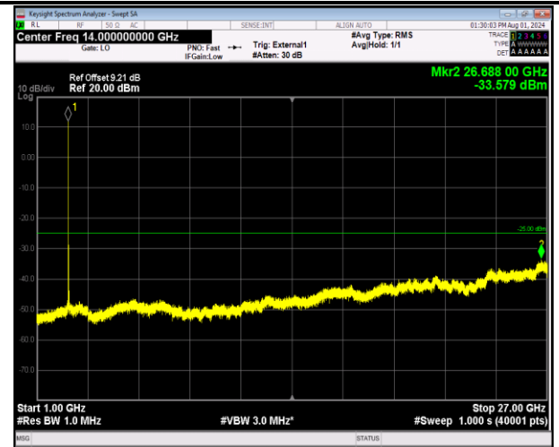
41-41-5MHz-20MHz-64QAM-64QAM-40648-40765-1RB#0- 1RB#99-1000~27000MHz-PASS
