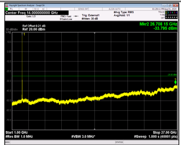
41-41-5MHz-20MHz-64QAM-64QAM-40648-40765-1RB#24 -0RB#0-1000~27000MHz-PASS
