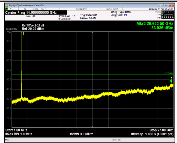
41-41-5MHz-20MHz-16QAM-16QAM-40273-40390-1RB#0- 0RB#0-1000~27000MHz-PASS
