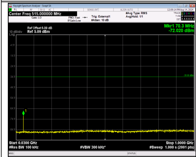
41-41-5MHz-20MHz-QPSK-QPSK-41023-41140-1RB#0-1RB#99-30~1000MHz-PASS
