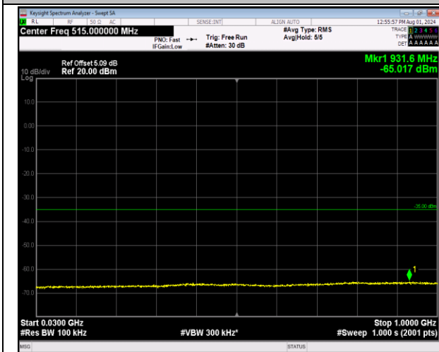
7-7-20MHz-20MHz-64QAM-64QAM-21152-21350-1RB#0 -ORB#0-30~1000MHz-PASS
