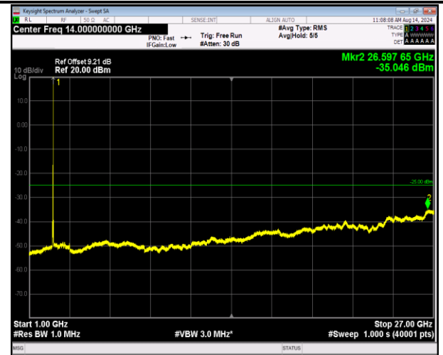
7-7-20MHz-20MHz-16QAM-16QAM-21001-21199-1RB#99- ORB#0-1000~27000MHz-PASS
