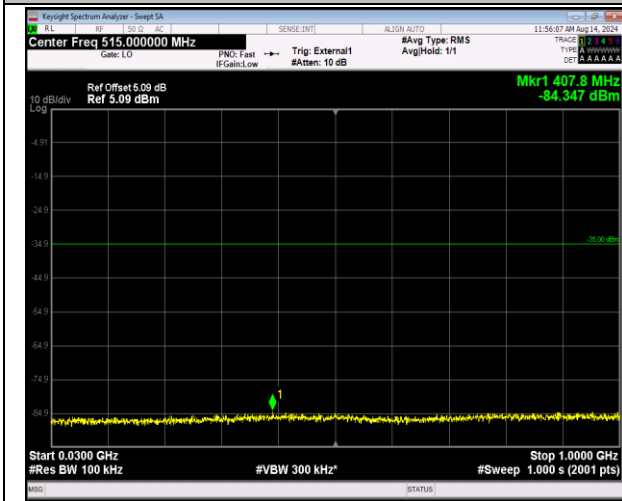
41-41-5MHz-20MHz-16QAM-16QAM-40273-40390-1RB# 0-1RB#99-30~1000MHz-PASS
