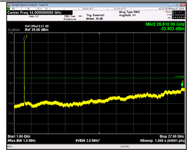
41-41-5MHz-20MHz-64QAM-64QAM-40273-40390-25RB#0 -100RB#0-1000~27000MHz-PASS
