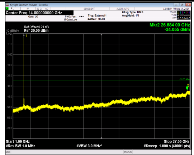
41-41-5MHz-20MHz-16QAM-16QAM-41023-41140-1RB#24 -ORB#0-1000~27000MHz-PASS
