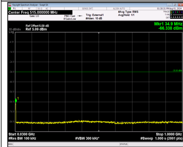
41-41-5MHz-20MHz-64QAM-64QAM-40648-40765-25RB #0-100RB#0-30~1000MHz-PASS
