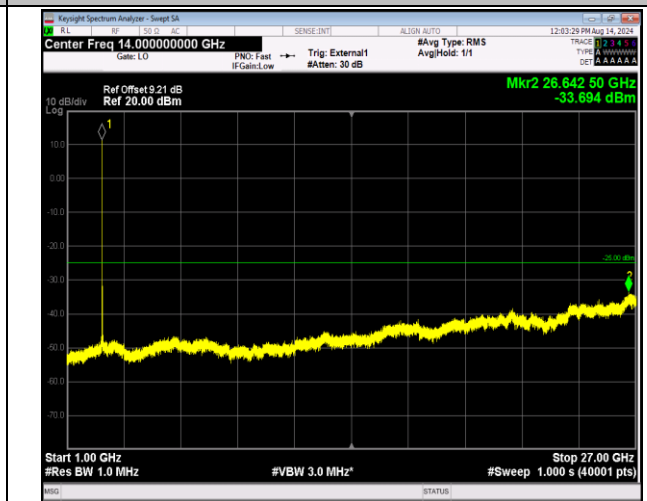
41-41-5MHz-20MHz-16QAM-16QAM-40648-40765-1RB#0- 1RB#99-1000~27000MHz-PASS
