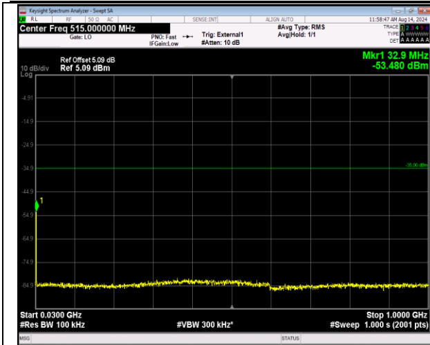
41-41-5MHz-20MHz-QPSK-QPSK-40648-40765-1RB#0-0RB#0-30~1000MHz-PASS
