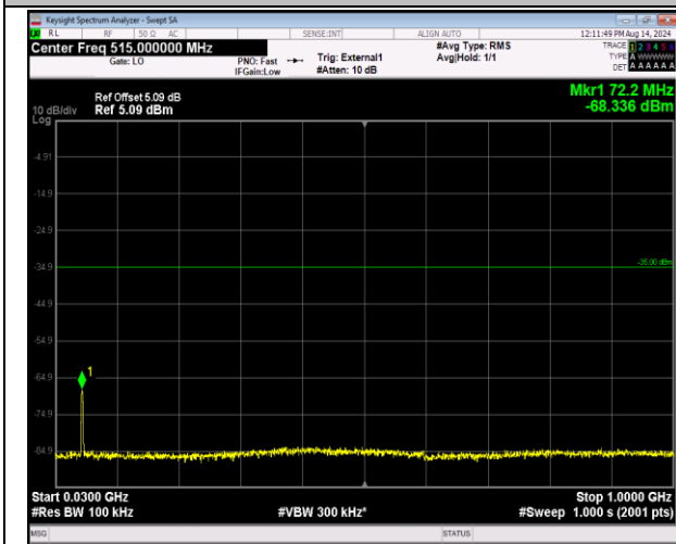
41-41-5MHz-20MHz-16QAM-16QAM-41023-41140-25RB# #0-100RB#0-30~1000MHz-PASS
