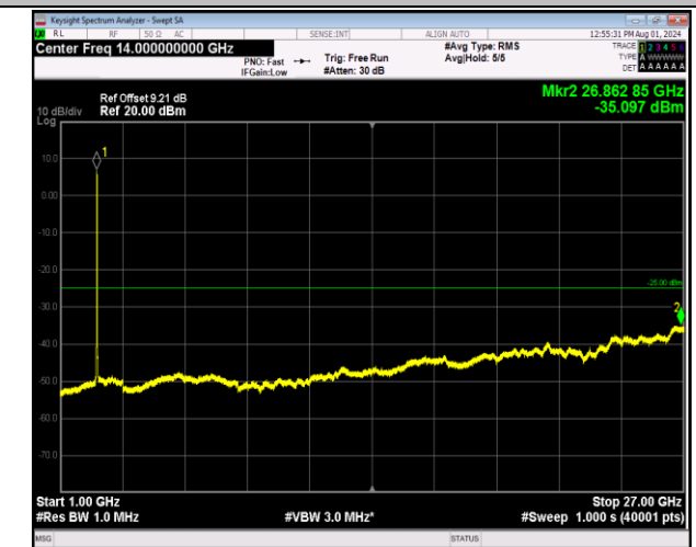
7-7-20MHz-20MHz-64QAM-64QAM-21001-21199-100RB#0-100RB#0-1000~27000MHz-PASS
