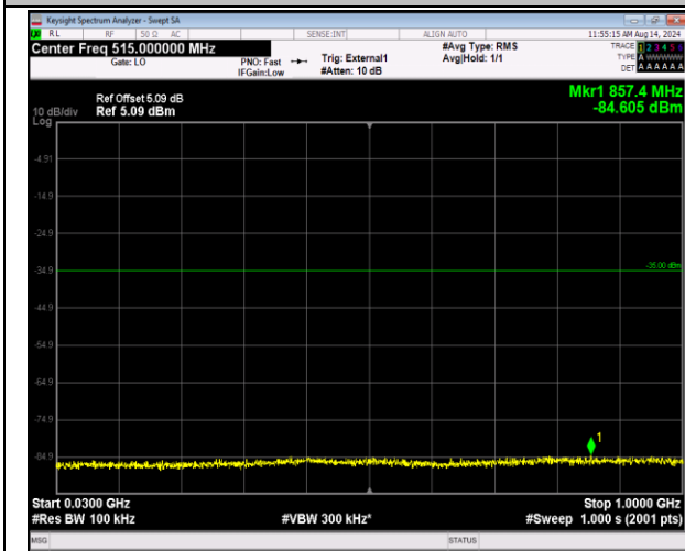
41-41-5MHz-20MHz-QPSK-QPSK-40273-40390-1RB#0-1RB#99-30~1000MHz-PASS
