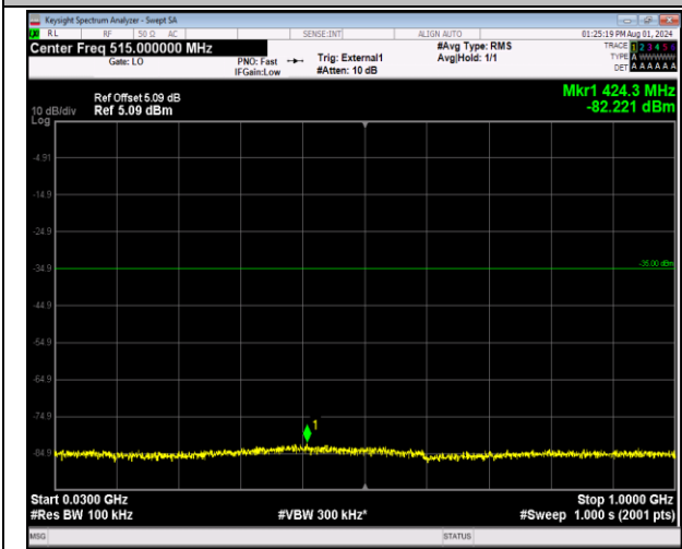
41-41-5MHz-20MHz-64QAM-64QAM-40273-40390-1RB# 24-0RB#0-30~1000MHz-PASS
