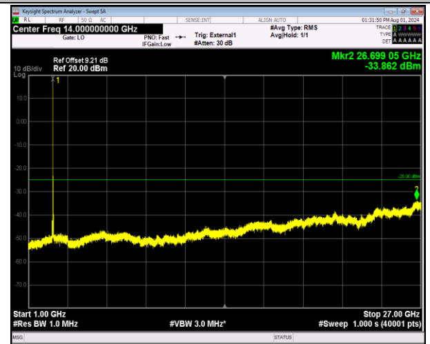
41-41-5MHz-20MHz-64QAM-64QAM-41023-41140-1RB#0- ORB#0-1000~27000MHz-PASS
