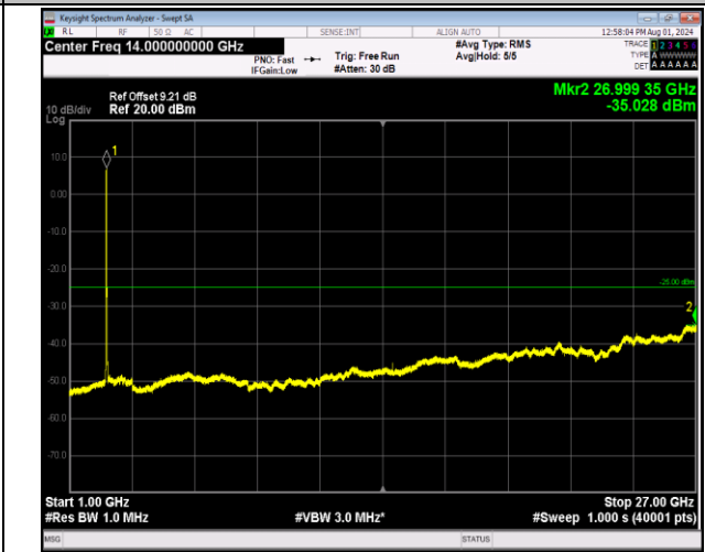
7-7-20MHz-20MHz-64QAM-64QAM-21152-21350-100RB#0-100RB#0-1000~27000MHz-PASS
