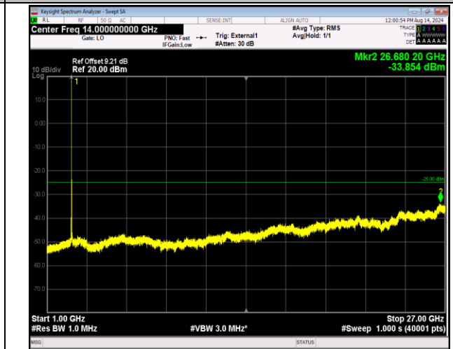
41-41-5MHz-20MHz-QPSK-QPSK-40648-40765-1RB#24-0RB#0-1000~27000MHz-PASS
