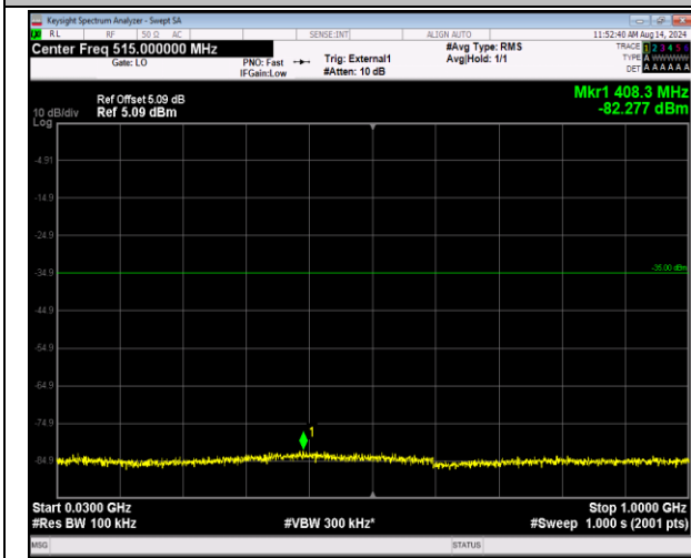
41-41-5MHz-20MHz-16QAM-16QAM-40273-40390-1RB# 0-0RB#0-30~1000MHz-PASS
