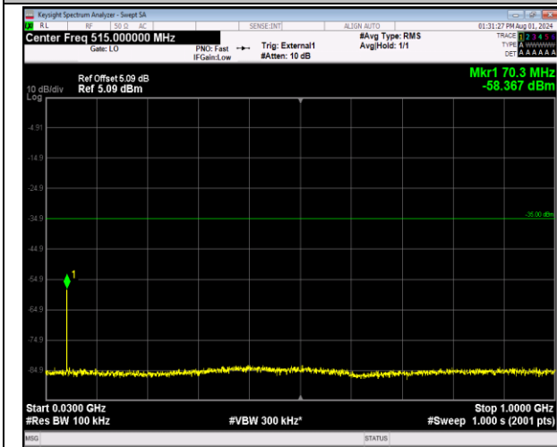
41-41-5MHz-20MHz-64QAM-64QAM-41023-41140-1RB# 0-ORB#0-30~1000MHz-PASS
