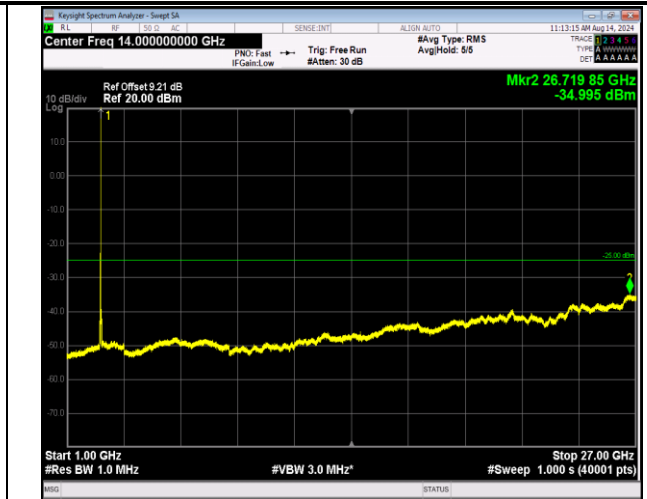
7-7-20MHz-20MHz-16QAM-16QAM-21152-21350-1RB#99- ORB#0-1000~27000MHz-PASS
