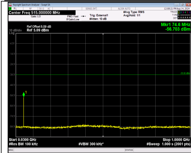
41-41-5MHz-20MHz-16QAM-16QAM-41023-41140-1RB# 24-ORB#0-30~1000MHz-PASS
