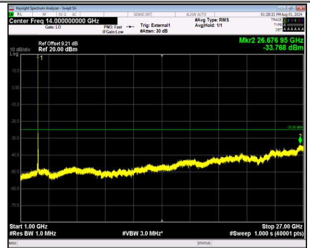
41-41-5MHz-20MHz-64QAM-64QAM-40648-40765-1RB#0- ORB#0-1000~27000MHz-PASS
