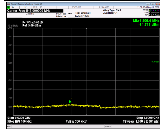
41-41-5MHz-20MHz-QPSK-QPSK-40273-40390-1RB#0-0RB#0-30~1000MHz-PASS
