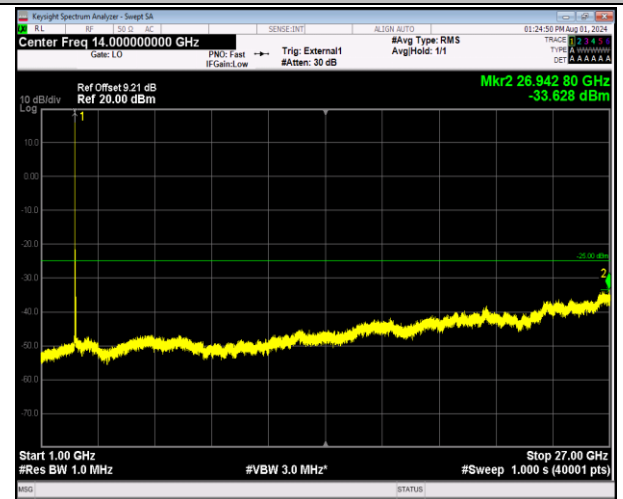
41-41-5MHz-20MHz-64QAM-64QAM-40273-40390-1RB#0- ORB#0-1000~27000MHz-PASS
