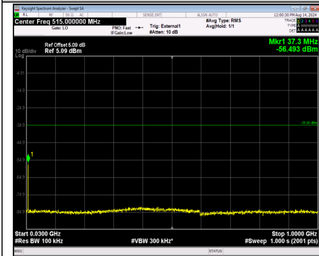
41-41-5MHz-20MHz-QPSK-QPSK-40648-40765-1RB#24-0RB#0-30~1000MHz-PASS
