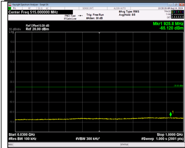
7-7-20MHz-10MHz-16QAM-16QAM-21051-21195-1RB#9 9-0RB#0-30~1000MHz-PASS
