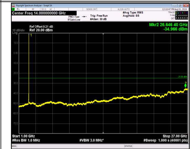
7-7-20MHz-10MHz-64QAM-64QAM-21251-21395-1RB#99-0 0RB#0-1000~27000MHz-PASS
