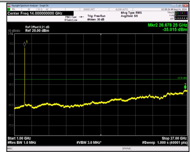
7-7-20MHz-10MHz-16QAM-16QAM-21251-21395-100RB#0 -50RB#0-1000~27000MHz-PASS
