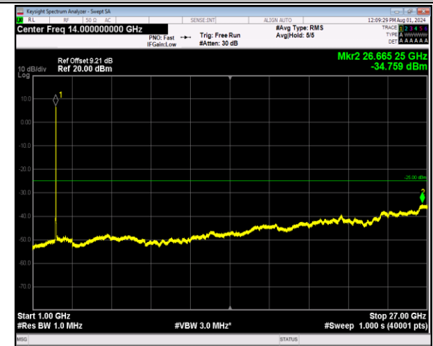
7-7-20MHz-10MHz-64QAM-64QAM-21051-21195-100RB#0 -50RB#0-1000~27000MHz-PASS
