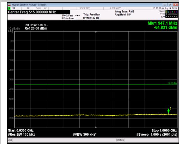
7-7-20MHz-10MHz-16QAM-16QAM-20850-20994-1RB#0 -ORB#0-30~1000MHz-PASS
