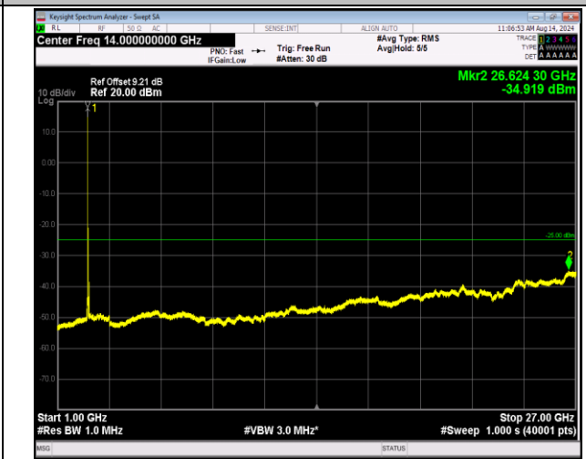
7-7-20MHz-20MHz-16QAM-16QAM-21001-21199-1RB#0-0 RB#0-1000~27000MHz-PASS
