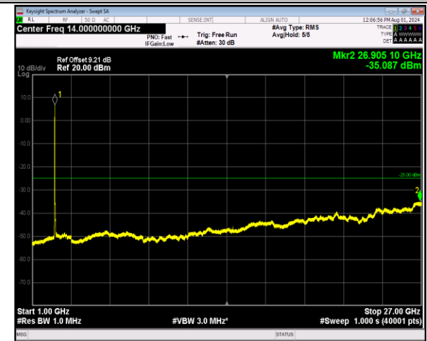
7-7-20MHz-10MHz-64QAM-64QAM-20850-20994-100RB#0 -50RB#0-1000~27000MHz-PASS
