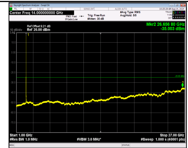
7-7-20MHz-10MHz-16QAM-16QAM-20850-20994-1RB#99- ORB#0-1000~27000MHz-PASS
