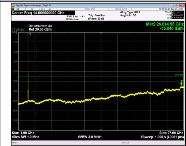
7-7-20MHz-10MHz-16QAM-16QAM-21051-21195-1RB#0-0 RB#0-1000~27000MHz-PASS
