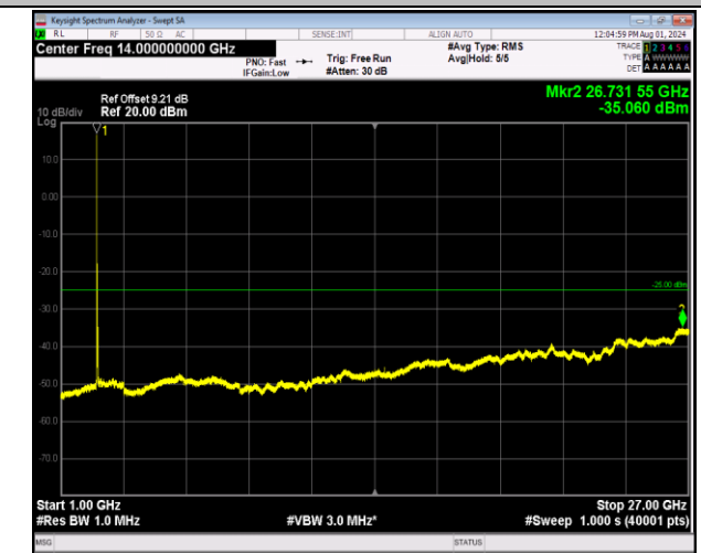
7-7-20MHz-10MHz-64QAM-64QAM-20850-20994-1RB#0-0 RB#0-1000~27000MHz-PASS
