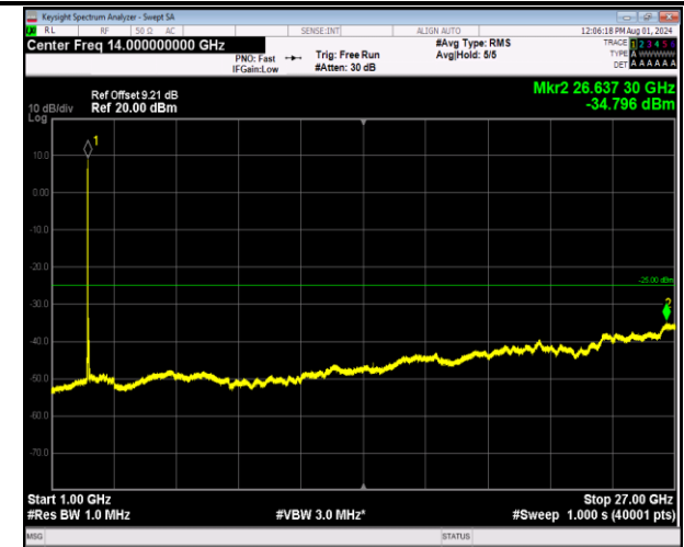
7-7-20MHz-10MHz-64QAM-64QAM-20850-20994-1RB#0-1 RB#49-1000~27000MHz-PASS
