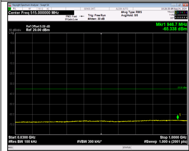
7-7-20MHz-10MHz-16QAM-16QAM-20850-20994-1RB#0 -1RB#49-30~1000MHz-PASS
