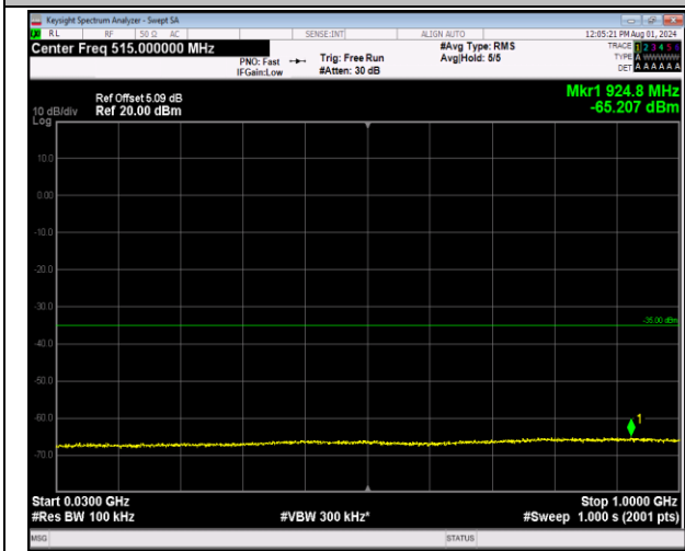
7-7-20MHz-10MHz-64QAM-64QAM-20850-20994-1RB#9 9-0RB#0-30~1000MHz-PASS
