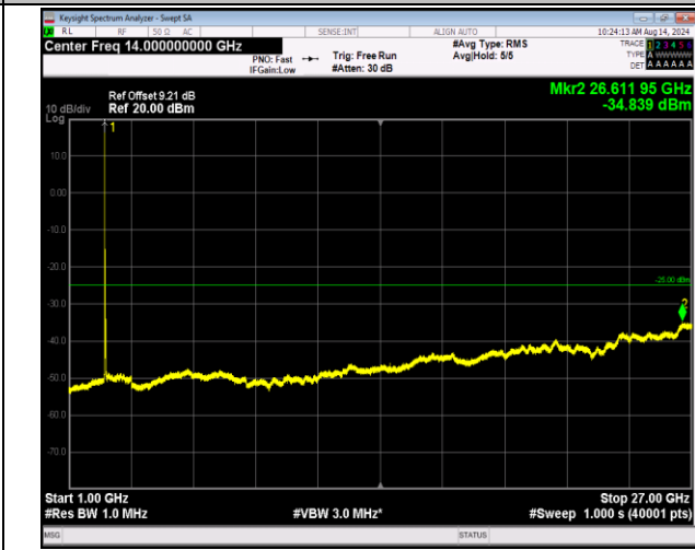
7-7-20MHz-10MHz-16QAM-16QAM-20850-20994-1RB#0-0 RB#0-1000~27000MHz-PASS
