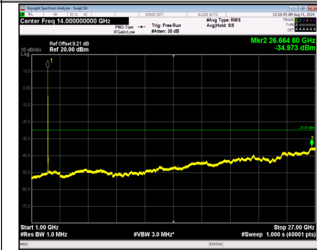
7-7-20MHz-10MHz-16QAM-16QAM-20850-20994-1RB#0-1 RB#49-1000~27000MHz-PASS
