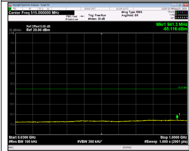
7-7-20MHz-10MHz-64QAM-64QAM-21051-21195-1RB#0 -0RB#0-30~1000MHz-PASS
