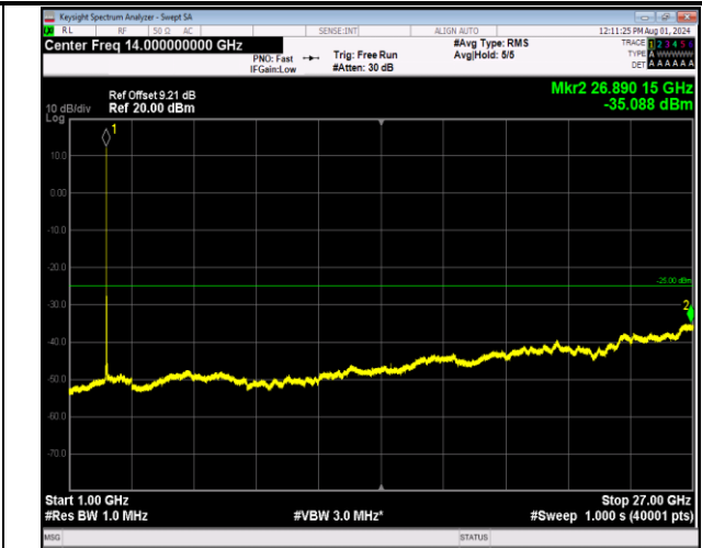
7-7-20MHz-10MHz-64QAM-64QAM-21251-21395-1RB#0-1 RB#49-1000~27000MHz-PASS
