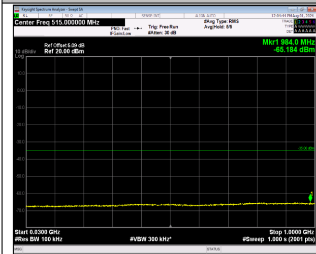
7-7-20MHz-10MHz-64QAM-64QAM-20850-20994-1RB#0 -ORB#0-30~1000MHz-PASS
