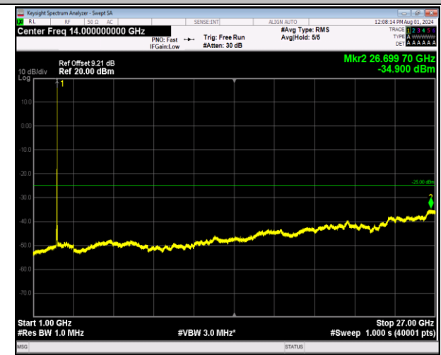
7-7-20MHz-10MHz-64QAM-64QAM-21051-21195-1RB#99- 0RB#0-1000~27000MHz-PASS
