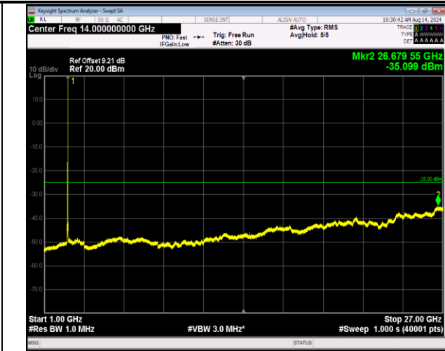
7-7-20MHz-10MHz-16QAM-16QAM-21051-21195-1RB#99- ORB#0-1000~27000MHz-PASS
