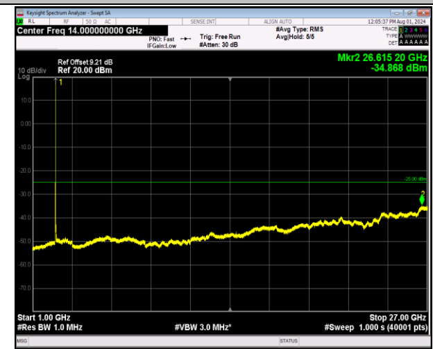
7-7-20MHz-10MHz-64QAM-64QAM-20850-20994-1RB#99- 0RB#0-1000~27000MHz-PASS
