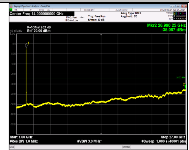
7-7-20MHz-10MHz-16QAM-16QAM-20850-20994-100RB#0 -50RB#0-1000~27000MHz-PASS
