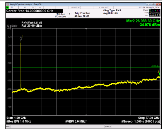
7-7-20MHz-20MHz-64QAM-64QAM-20850-21048-100RB#0-100RB#0-1000~27000MHz-PASS
