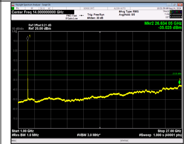
7-7-20MHz-10MHz-16QAM-16QAM-21051-21195-1RB#0-1 RB#49-1000~27000MHz-PASS
