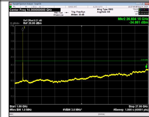
7-7-20MHz-10MHz-16QAM-16QAM-21251-21395-1RB#0-1 RB#49-1000~27000MHz-PASS
