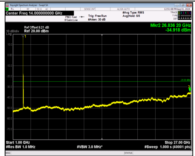
7-7-20MHz-20MHz-64QAM-64QAM-20850-21048-1RB#0-0 RB#0-1000~27000MHz-PASS
