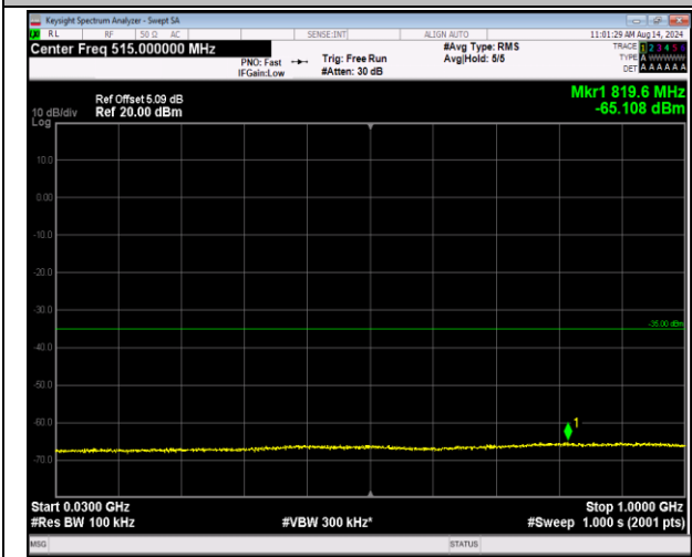
7-7-20MHz-20MHz-16QAM-16QAM-20850-21048-1RB#0 -0RB#0-30~1000MHz-PASS
