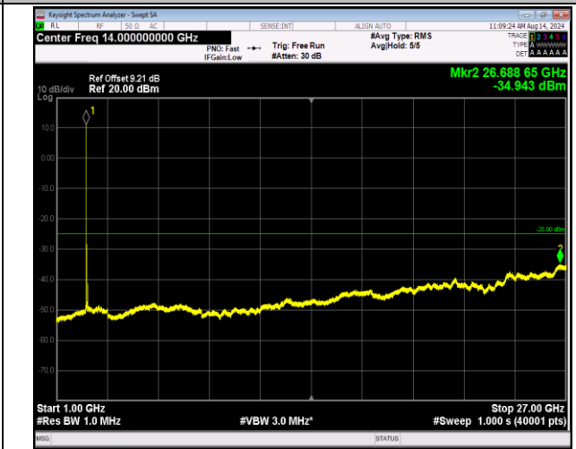
7-7-20MHz-20MHz-16QAM-16QAM-21001-21199-1RB#0-1 RB#99-1000~27000MHz-PASS
