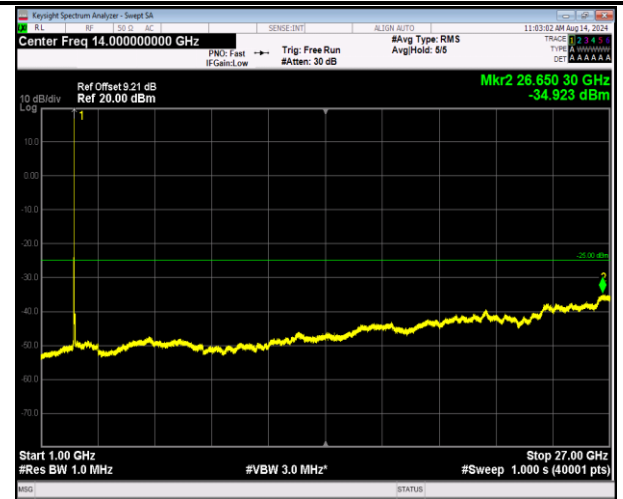
7-7-20MHz-20MHz-16QAM-16QAM-20850-21048-1RB#99- ORB#0-1000~27000MHz-PASS
