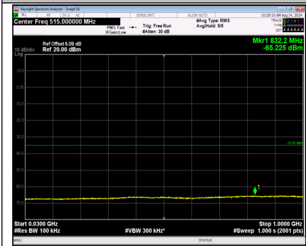
7-7-20MHz-10MHz-16QAM-16QAM-21051-21195-1RB#0 -0RB#0-30~1000MHz-PASS
