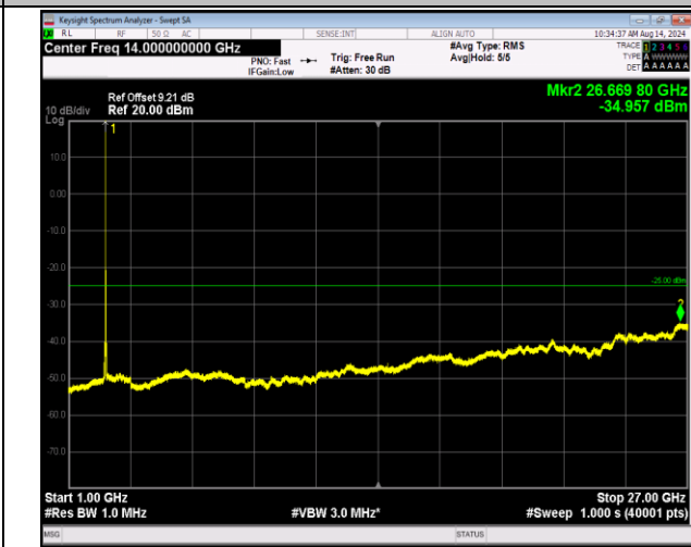
7-7-20MHz-10MHz-16QAM-16QAM-21251-21395-1RB#0-0 RB#0-1000~27000MHz-PASS
