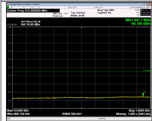
7-7-20MHz-20MHz-QPSK-QPSK-21001-21199-1RB#99-0 ORB#0-30~1000MHz-PASS
