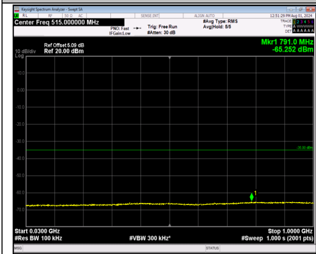
7-7-20MHz-20MHz-64QAM-64QAM-20850-21048-1RB#9 9-0RB#0-30~1000MHz-PASS
