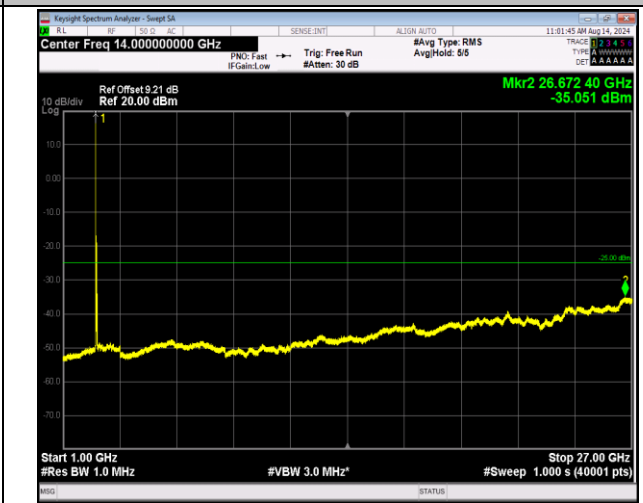
7-7-20MHz-20MHz-16QAM-16QAM-20850-21048-1RB#0-0 RB#0-1000~27000MHz-PASS
