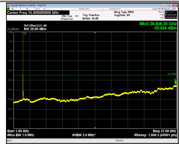
7-7-20MHz-20MHz-64QAM-64QAM-20850-21048-1RB#99-0RB#0-1000~27000MHz-PASS
