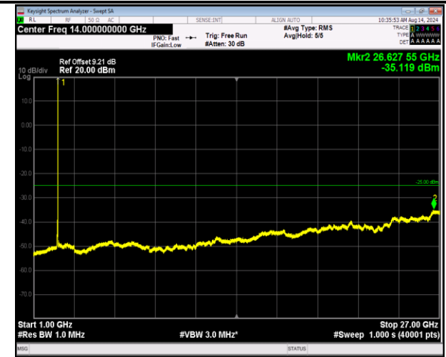
7-7-20MHz-10MHz-16QAM-16QAM-21251-21395-1RB#99- 0RB#0-1000~27000MHz-PASS
