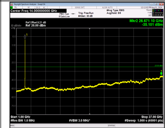
7-7-20MHz-10MHz-64QAM-64QAM-21251-21395-100RB#0 -50RB#0-1000~27000MHz-PASS
