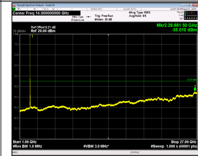
7-7-20MHz-10MHz-64QAM-64QAM-21051-21195-1RB#0-0 RB#0-1000~27000MHz-PASS
