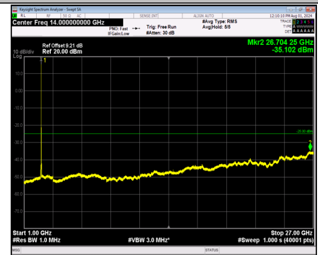
7-7-20MHz-10MHz-64QAM-64QAM-21251-21395-1RB#0-0 RB#0-1000~27000MHz-PASS
