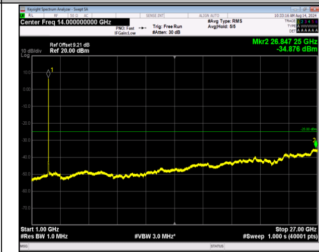
7-7-20MHz-10MHz-16QAM-16QAM-21051-21195-100RB#0 -50RB#0-1000~27000MHz-PASS
