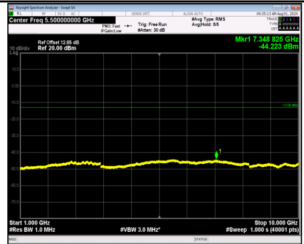
5-5-5MHz-3MHz-64QAM-64QAM-20595-20634-1RB#0-1RB #15-1000~10000MHz-PASS
