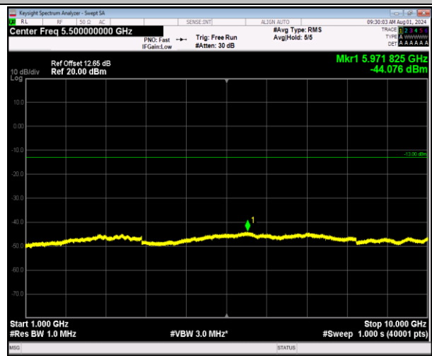
5-5-5MHz-3MHz-64QAM-64QAM-20425-20464-1RB#24-OR B#0-1000~10000MHz-PASS
