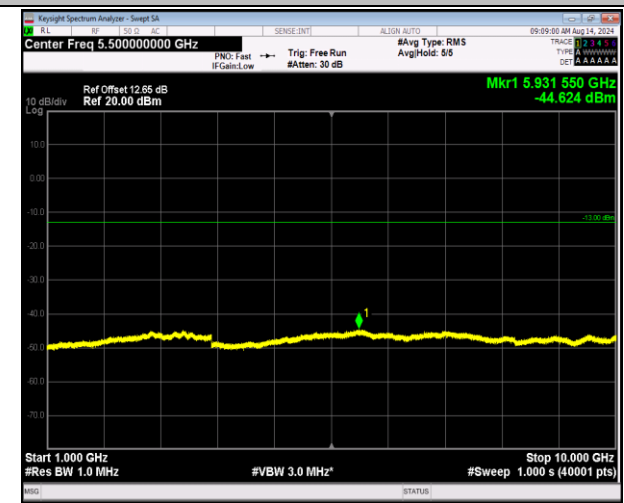
5-5-10MHz-10MHz-16QAM-16QAM-20476-20575-1RB#0-0RB#0-1000~10000MHz-PASS
