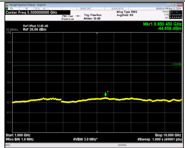
5-5-5MHz-3MHz-16QAM-16QAM-20595-20634-1RB#0-1RB #15-1000~10000MHz-PASS
