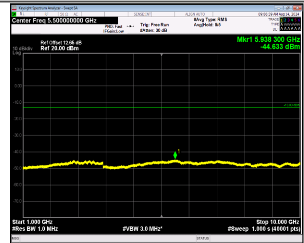
5-5-10MHz-10MHz-16QAM-16QAM-20450-20549-1RB#0-1-1000~10000MHz-PASS
