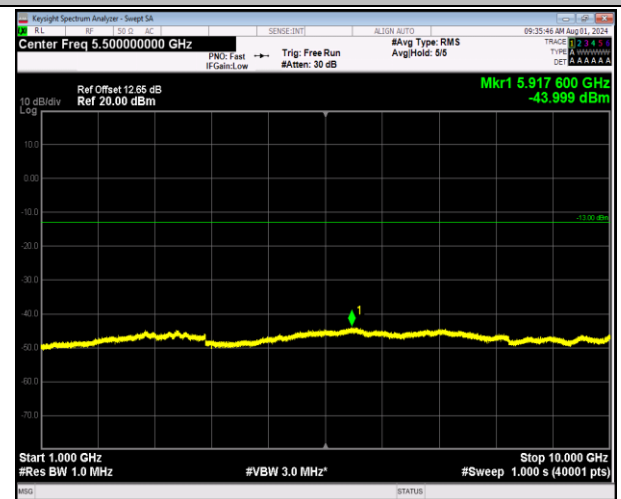
5-5-5MHz-3MHz-64QAM-64QAM-20595-20634-25RB#0-15 RB#0-1000~10000MHz-PASS
