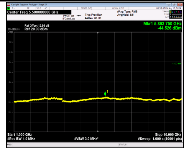
5-5-5MHz-3MHz-QPSK-QPSK-20510-20549-1RB#0-0RB#0 -1000~10000MHz-PASS
