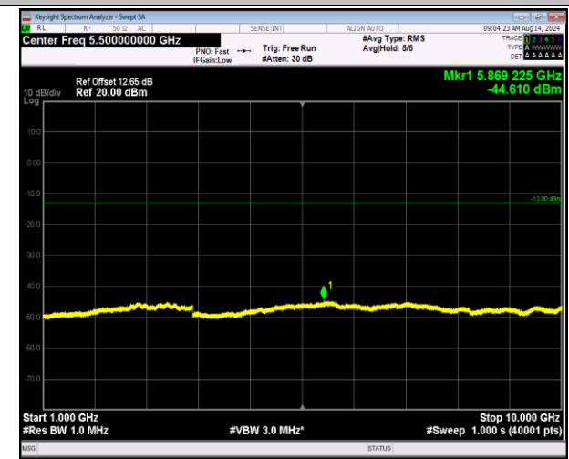
5-5-10MHz-10MHz-16QAM-16QAM-20450-20549-1RB#0-0-1000~10000MHz-PASS
