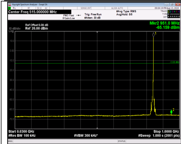
5-5-5MHz-3MHz-16QAM-16QAM-20595-20634-1RB#24-0RB#0-30~1000MHz-PASS
