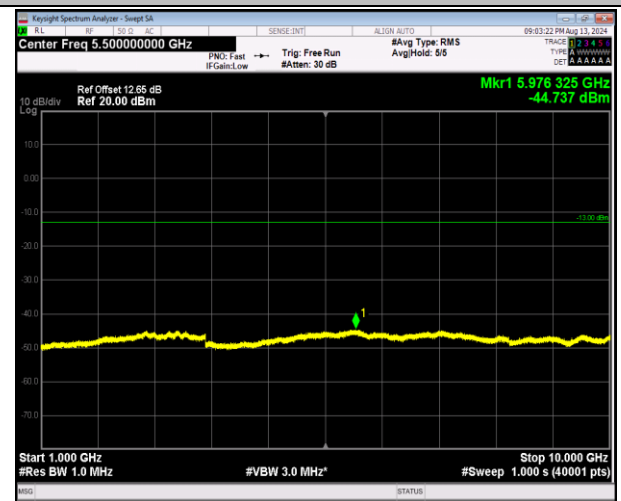
5-5-5MHz-3MHz-16QAM-16QAM-20595-20634-1RB#0-0RB #0-1000~10000MHz-PASS
