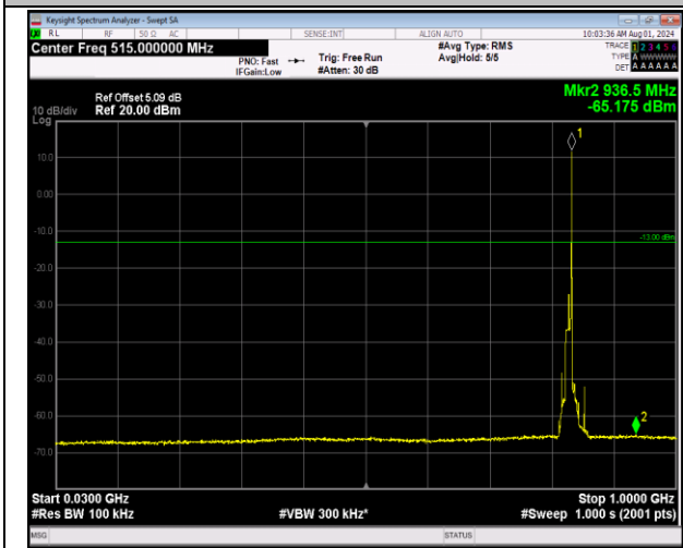
5-5-10MHz-10MHz-64QAM-64QAM-20476-20575-1RB#4 9-0RB#0-30~1000MHz-PASS
