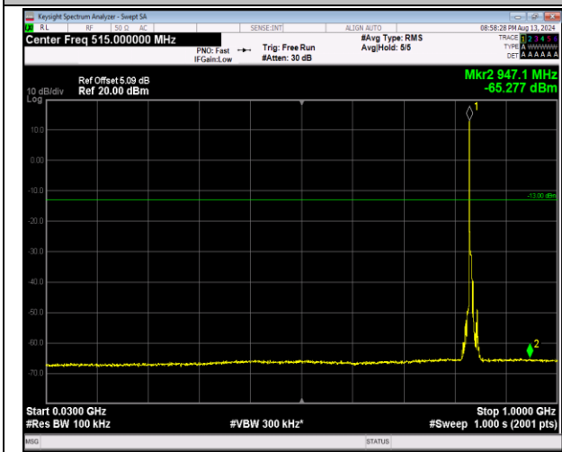
5-5-5MHz-3MHz-16QAM-16QAM-20510-20549-1RB#0-0 RB#0-30~1000MHz-PASS
