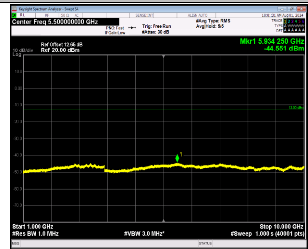
5-5-10MHz-10MHz-64QAM-64QAM-20450-20549-1RB#49- 0RB#0-1000~10000MHz-PASS
