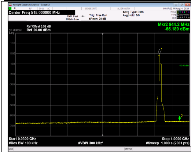
5-5-10MHz-10MHz-QPSK-QPSK-20450-20549-50RB#0-50RB#0-30~1000MHz-PASS
