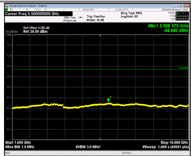
5-5-10MHz-10MHz-QPSK-QPSK-20450-20549-1RB#0-1RB #49-1000~10000MHz-PASS
