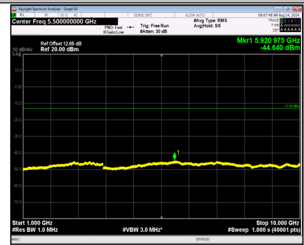
5-5-10MHz-10MHz-16QAM-16QAM-20450-20549-50RB#0- 50RB#0-1000~10000MHz-PASS
