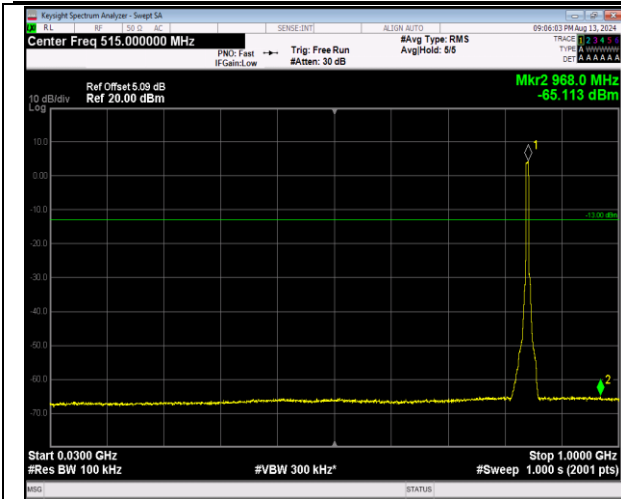
5-5-5MHz-3MHz-QPSK-QPSK-20595-20634-25RB#0-15 RB#0-30~1000MHz-PASS
