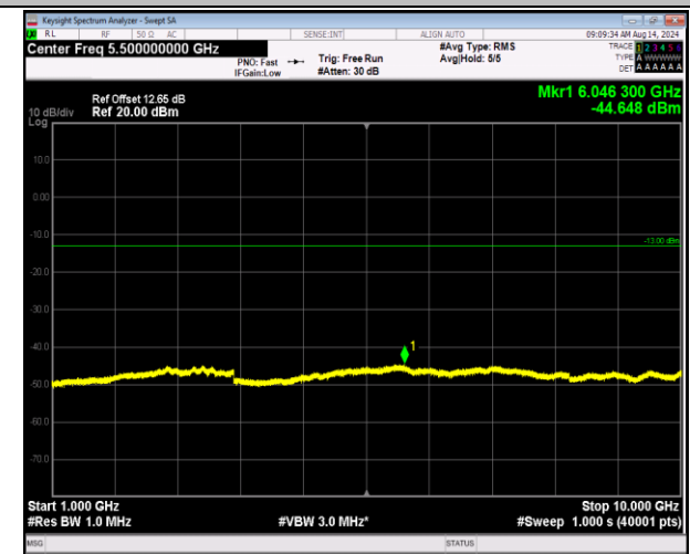
5-5-10MHz-10MHz-QPSK-QPSK-20476-20575-1RB#49-0R B#0-1000~10000MHz-PASS
