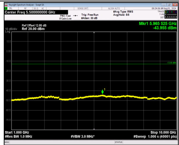
5-5-5MHz-3MHz-64QAM-64QAM-20595-20634-1RB#0-0RB#0-1000~10000MHz-PASS
