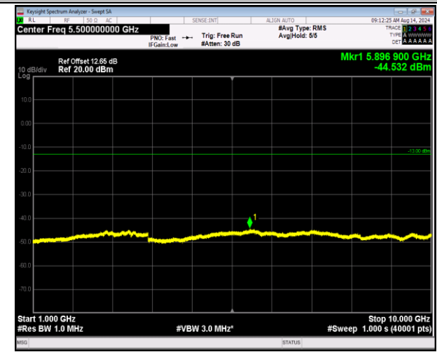
5-5-10MHz-10MHz-16QAM-16QAM-20476-20575-50RB#0- 50RB#0-1000~10000MHz-PASS
