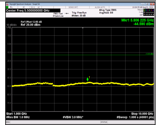
5-5-10MHz-10MHz-64QAM-64QAM-20476-20575-50RB#0- 50RB#0-1000~10000MHz-PASS
