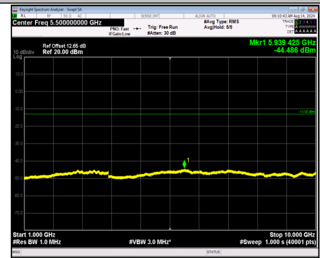
5-5-10MHz-10MHz-QPSK-QPSK-20476-20575-1RB#0-1RB #49-1000~10000MHz-PASS
