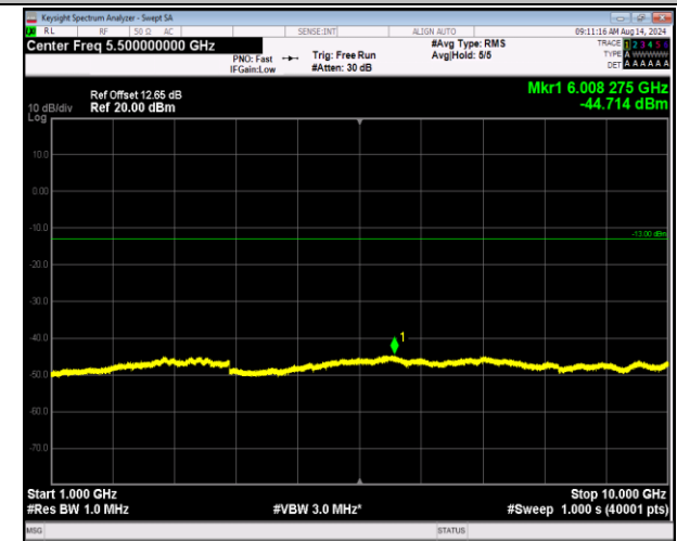
5-5-10MHz-10MHz-16QAM-16QAM-20476-20575-1RB#0-1RB#49-1000~10000MHz-PASS
