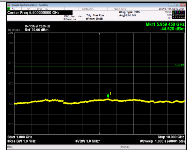
5-5-10MHz-10MHz-64QAM-64QAM-20450-20549-1RB#0-0 RB#0-1000~10000MHz-PASS
