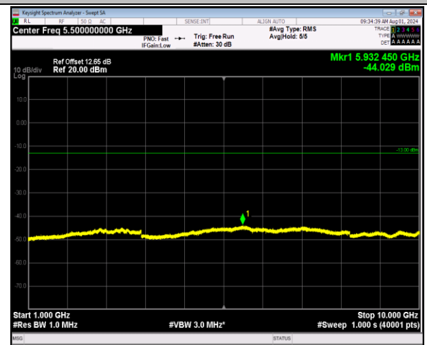
5-5-5MHz-3MHz-64QAM-64QAM-20595-20634-1RB#24-OR B#0-1000~10000MHz-PASS
