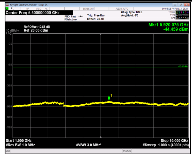
5-5-5MHz-3MHz-QPSK-QPSK-20595-20634-25RB#0-15RB #0-1000~10000MHz-PASS
