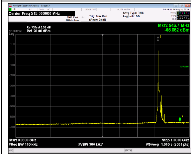
5-5-10MHz-10MHz-16QAM-16QAM-20450-20549-1RB#0-0RB#0-30~1000MHz-PASS
