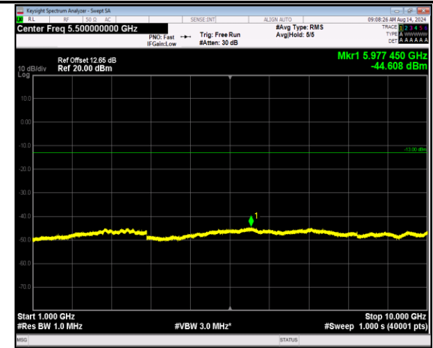
5-5-10MHz-10MHz-QPSK-QPSK-20476-20575-1RB#0-0RB #0-1000~10000MHz-PASS
