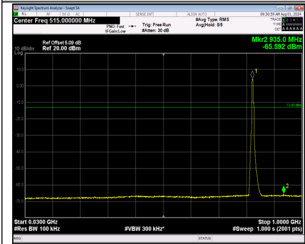
5-5-5MHz-3MHz-64QAM-64QAM-20425-20464-25RB#0- 15RB#0-30~1000MHz-PASS
