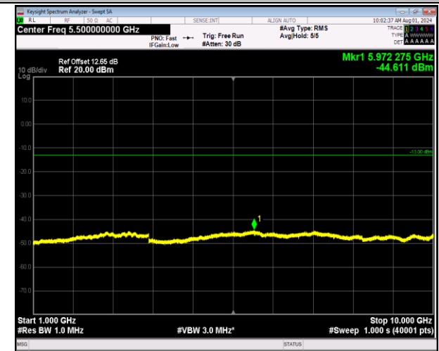
5-5-10MHz-10MHz-64QAM-64QAM-20450-20549-50RB#0- 50RB#0-1000~10000MHz-PASS
