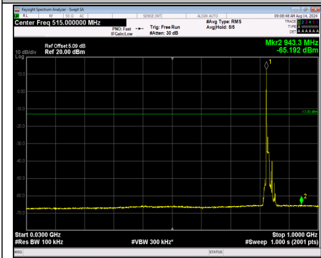
5-5-10MHz-10MHz-16QAM-16QAM-20476-20575-1RB#0-0RB#0-30~1000MHz-PASS
