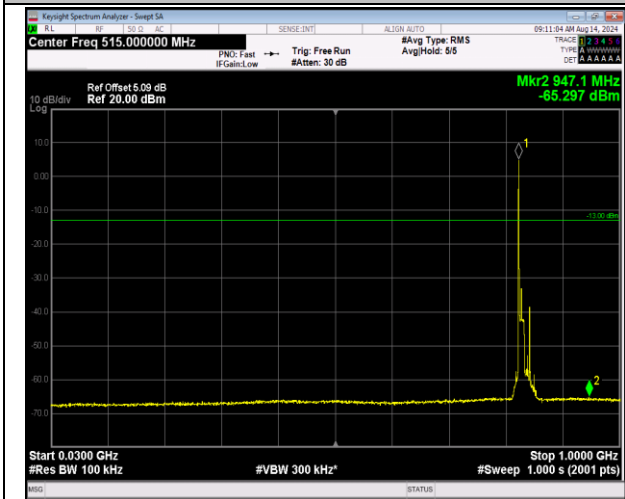
5-5-10MHz-10MHz-16QAM-16QAM-20476-20575-1RB#0-1RB#49-30~1000MHz-PASS
