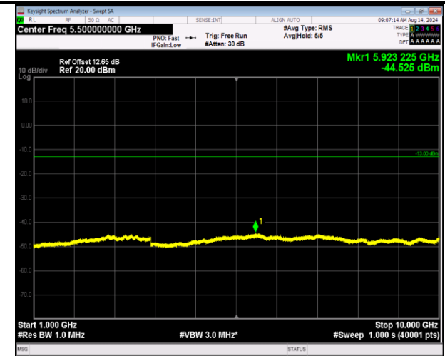
5-5-10MHz-10MHz-QPSK-QPSK-20450-20549-50RB#0-50RB#0-1000~10000MHz-PASS
