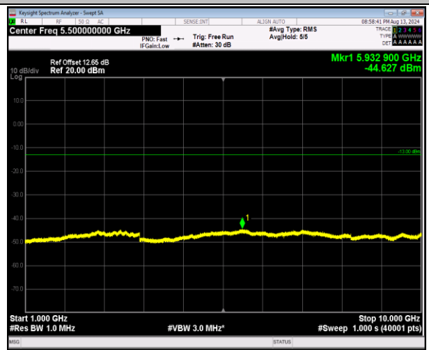
5-5-5MHz-3MHz-16QAM-16QAM-20510-20549-1RB#0-0RB #0-1000~10000MHz-PASS
