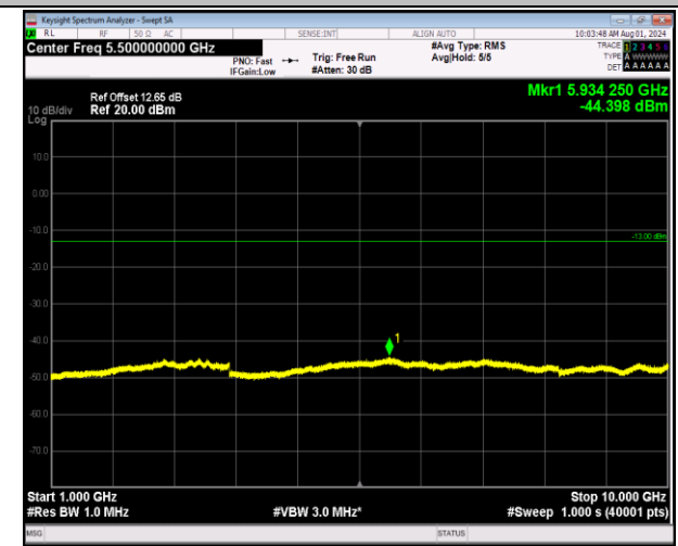
5-5-10MHz-10MHz-64QAM-64QAM-20476-20575-1RB#49- 0RB#0-1000~10000MHz-PASS
