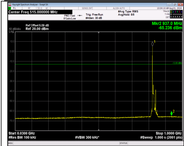
5-5-10MHz-10MHz-64QAM-64QAM-20476-20575-1RB#0 -1RB#49-30~1000MHz-PASS
