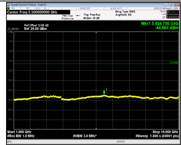
5-5-10MHz-10MHz-64QAM-64QAM-20476-20575-1RB#0-0 RB#0-1000~10000MHz-PASS
