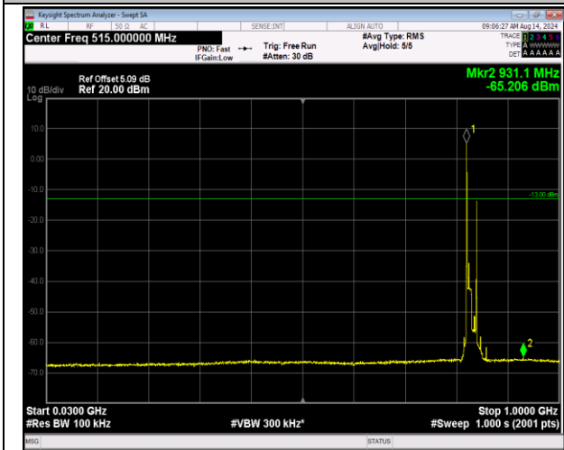
5-5-10MHz-10MHz-16QAM-16QAM-20450-20549-1RB#0-1RB#49-30~1000MHz-PASS
