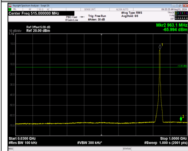
5-5-5MHz-3MHz-64QAM-64QAM-20595-20634-25RB#0- 15RB#0-30~1000MHz-PASS
