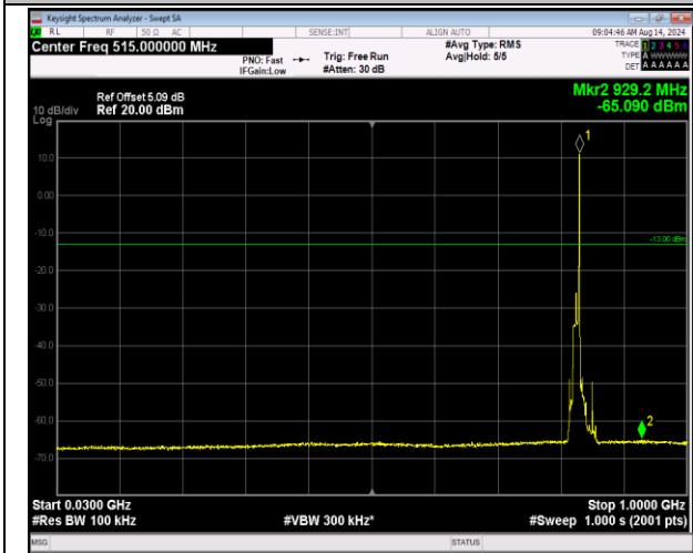
5-5-10MHz-10MHz-QPSK-QPSK-20450-20549-1RB#49-49 ORB#0-30~1000MHz-PASS
