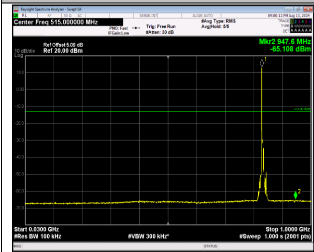
5-5-5MHz-3MHz-QPSK-QPSK-20510-20549-1RB#0-1RB #15-30~1000MHz-PASS
