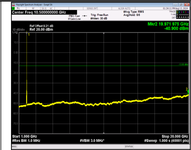
2-2-5MHz-20MHz-16QAM-16QAM-18808-18925-1RB#24-0 RB#0-1000~20000MHz-PASS
