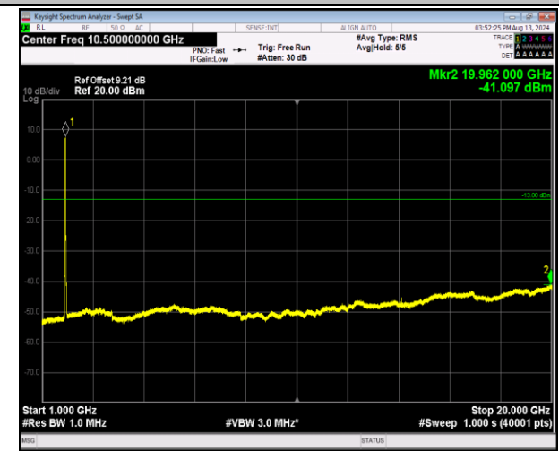
2-2-20MHz-20MHz-16QAM-16QAM-18801-18999-100RB#0 -100RB#0-1000~20000MHz-PASS
