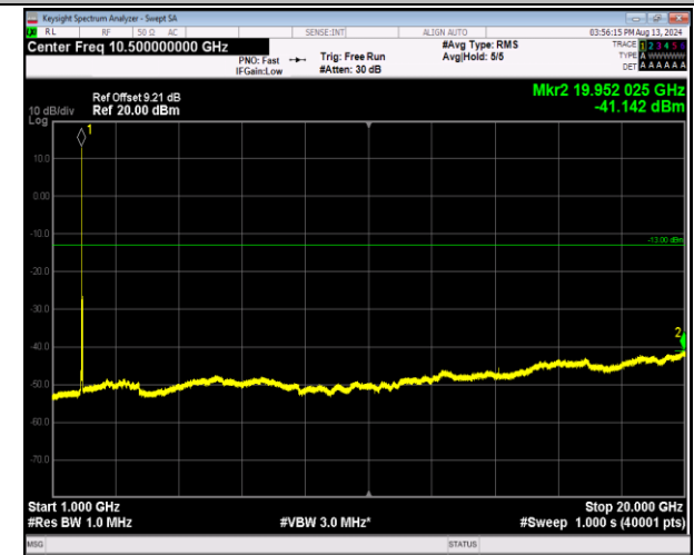
2-2-20MHz-20MHz-16QAM-16QAM-18902-19100-1RB#0-1 RB#99-1000~20000MHz-PASS
