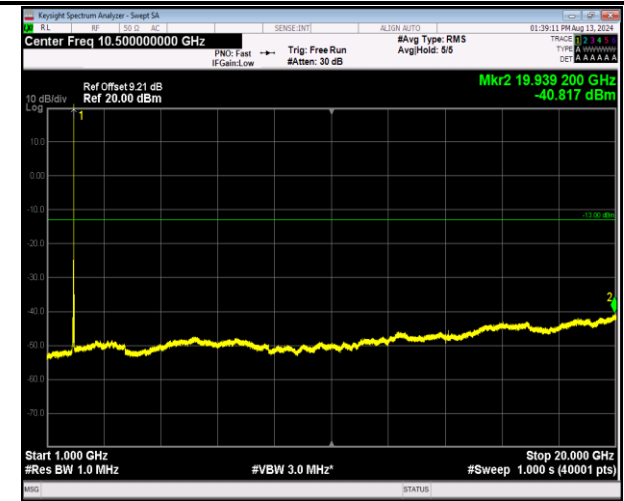
2-2-5MHz-20MHz-16QAM-16QAM-18983-19100-1RB#24-0 RB#0-1000~20000MHz-PASS
