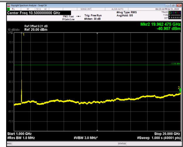
2-2-5MHz-20MHz-64QAM-64QAM-18808-18925-1RB#24-0RB#0-1000~20000MHz-PASS
