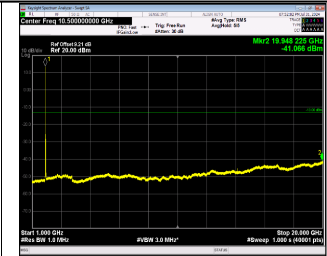
2-2-20MHz-20MHz-64QAM-64QAM-18801-18999-1RB#0-1 RB#99-1000~20000MHz-PASS
