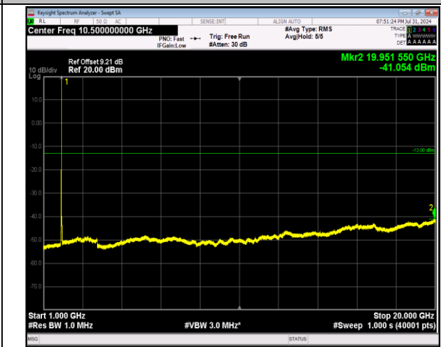
2-2-20MHz-20MHz-64QAM-64QAM-18801-18999-1RB#99-0RB#0-1000~20000MHz-PASS
