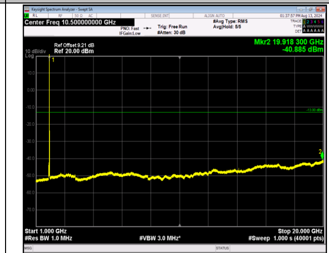
2-2-5MHz-20MHz-16QAM-16QAM-18983-19100-1RB#0-0RB#0-1000~20000MHz-PASS
