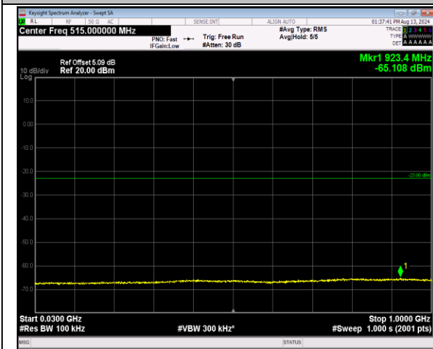
2-2-5MHz-20MHz-16QAM-16QAM-18983-19100-1RB#0-0RB#0-30~1000MHz-PASS
