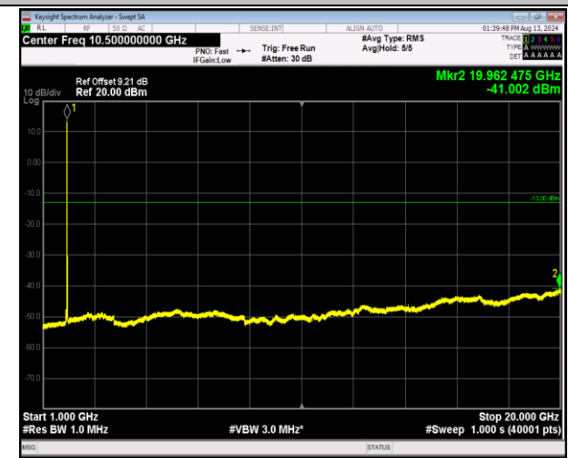
2-2-5MHz-20MHz-QPSK-QPSK-18983-19100-1RB#0-1RB# 99-1000~20000MHz-PASS
