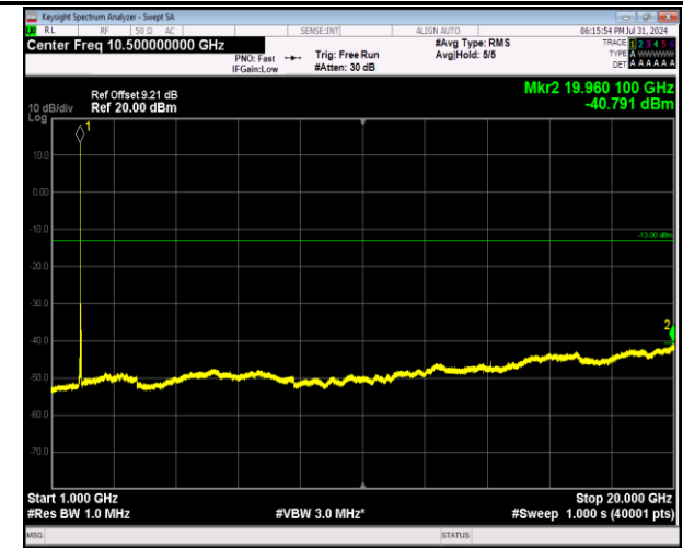
2-2-5MHz-20MHz-64QAM-64QAM-18808-18925-1RB#0-1RB#99-1000~20000MHz-PASS
