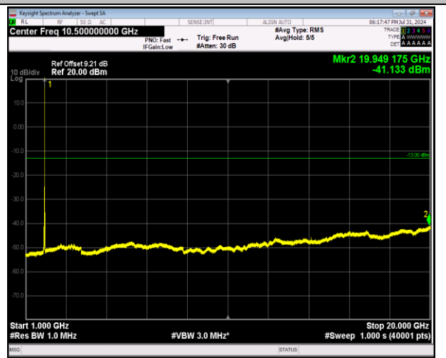
2-2-5MHz-20MHz-64QAM-64QAM-18983-19100-1RB#24-0RB#0-1000~20000MHz-PASS
