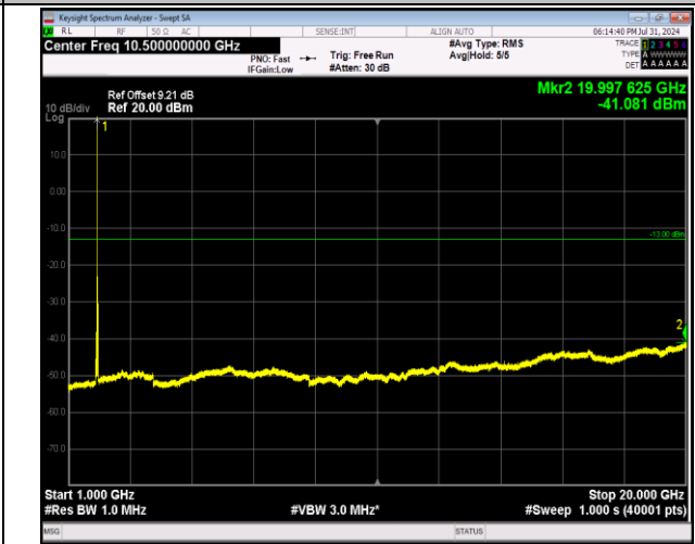
2-2-5MHz-20MHz-64QAM-64QAM-18808-18925-1RB#0-0R B#0-1000~20000MHz-PASS
