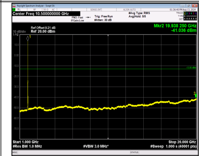
2-2-5MHz-20MHz-16QAM-16QAM-18808-18925-25RB#0-1 00RB#0-1000~20000MHz-PASS
