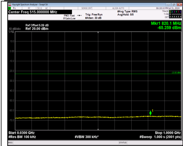
2-2-5MHz-20MHz-64QAM-64QAM-18983-19100-1RB#0-1RB#99-30~1000MHz-PASS
