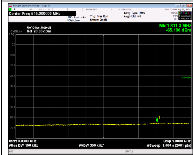
2-2-5MHz-20MHz-16QAM-16QAM-18983-19100-25RB#0 -100RB#0-30~1000MHz-PASS
