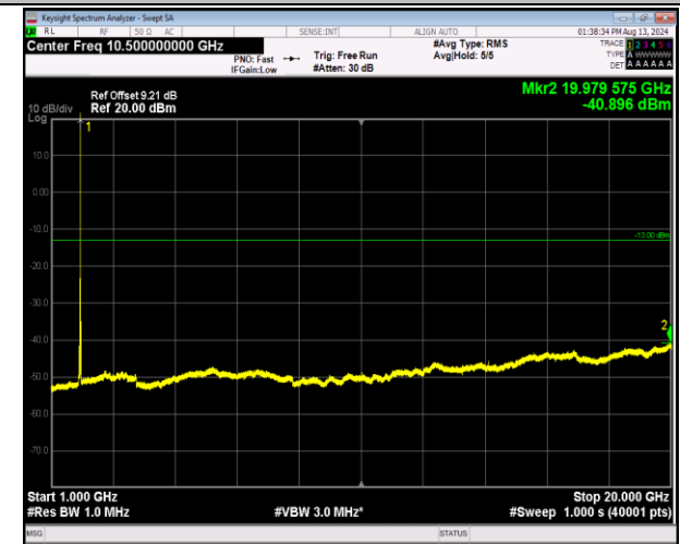
2-2-5MHz-20MHz-QPSK-QPSK-18983-19100-1RB#24-0RB #0-1000~20000MHz-PASS
