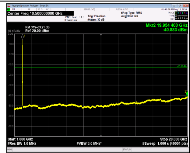
2-2-5MHz-20MHz-16QAM-16QAM-18983-19100-25RB#0-1 00RB#0-1000~20000MHz-PASS
