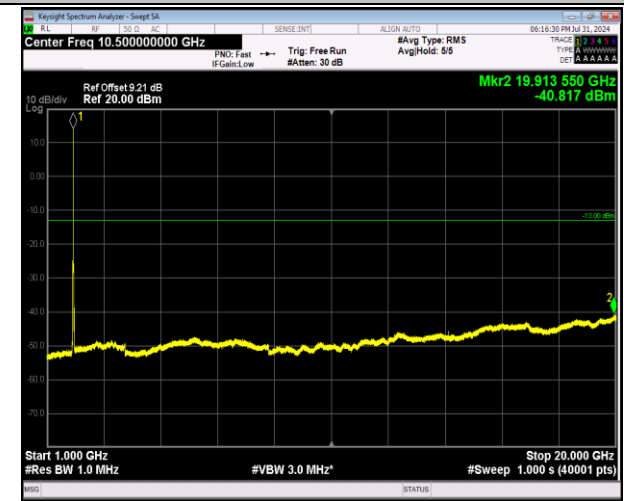
2-2-5MHz-20MHz-64QAM-64QAM-18808-18925-25RB#0-100RB#0-1000~20000MHz-PASS
