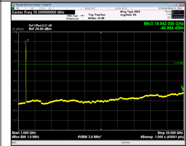
2-2-20MHz-20MHz-64QAM-64QAM-18700-18898-100RB#0-100RB#0-1000~20000MHz-PASS
