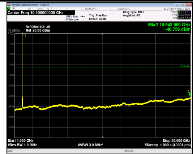
2-2-5MHz-20MHz-QPSK-QPSK-18983-19100-1RB#0-0RB# 0-1000~20000MHz-PASS
