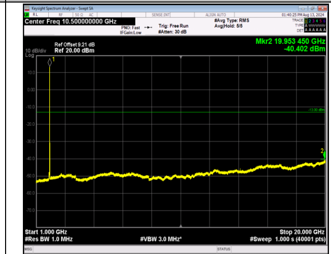
2-2-5MHz-20MHz-16QAM-16QAM-18983-19100-1RB#0-1RB#99-1000~20000MHz-PASS
