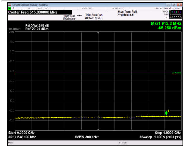
2-2-5MHz-20MHz-64QAM-64QAM-18808-18925-1RB#0-0 0RB#0-30~1000MHz-PASS
