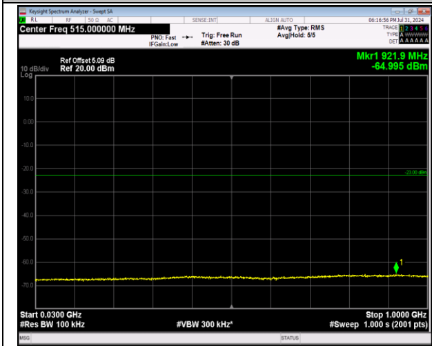
2-2-5MHz-20MHz-64QAM-64QAM-18983-19100-1RB#0-0 0RB#0-30~1000MHz-PASS
