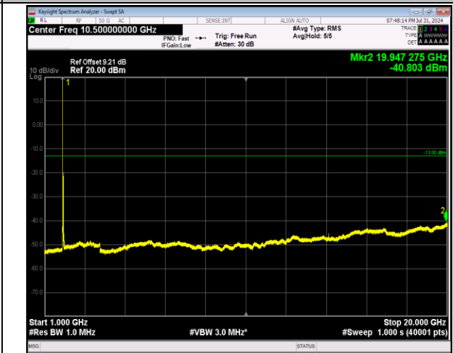
2-2-20MHz-20MHz-64QAM-64QAM-18700-18898-1RB#0-0 RB#0-1000~20000MHz-PASS
