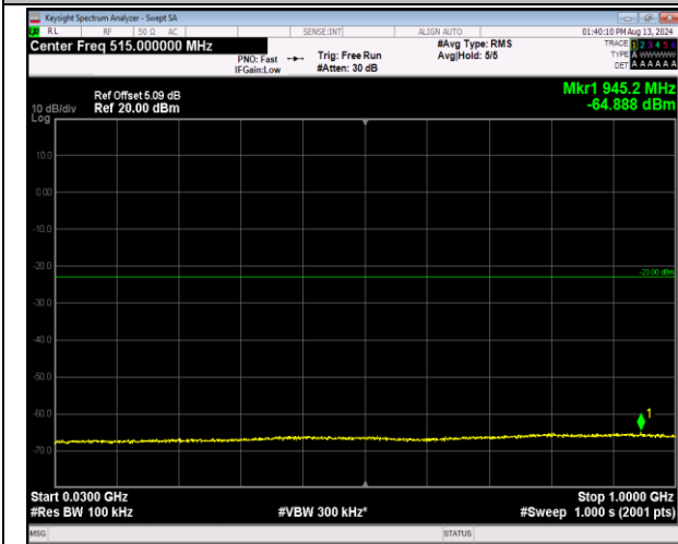
2-2-5MHz-20MHz-16QAM-16QAM-18983-19100-1RB#0-1RB#99-30~1000MHz-PASS
