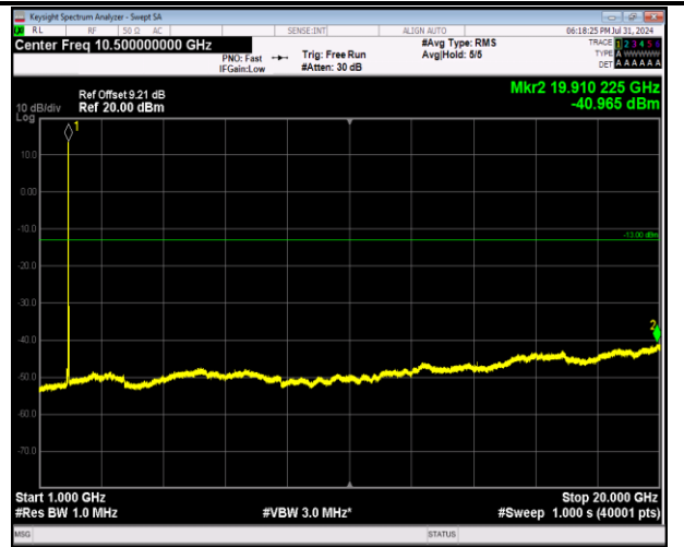
2-2-5MHz-20MHz-64QAM-64QAM-18983-19100-1RB#0-1RB#99-1000~20000MHz-PASS
