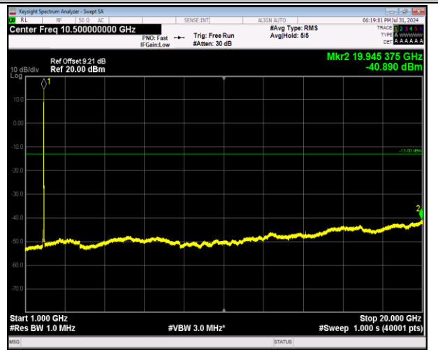
2-2-5MHz-20MHz-64QAM-64QAM-18983-19100-25RB#0-100RB#0-1000~20000MHz-PASS
