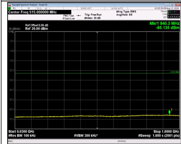
2-2-20MHz-20MHz-16QAM-16QAM-18902-19100-1RB#0 -1RB#99-30~1000MHz-PASS
