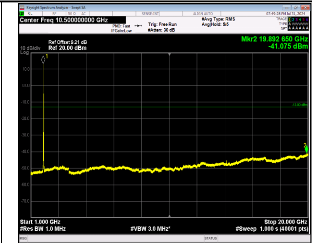
2-2-20MHz-20MHz-64QAM-64QAM-18700-18898-1RB#0-1 RB#99-1000~20000MHz-PASS
