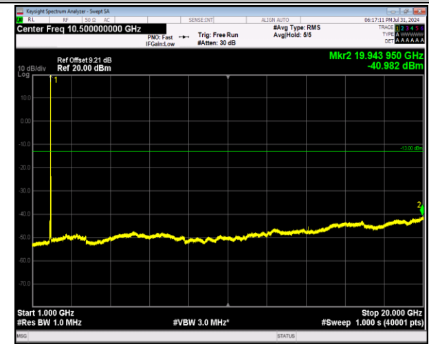
2-2-5MHz-20MHz-64QAM-64QAM-18983-19100-1RB#0-0R B#0-1000~20000MHz-PASS
