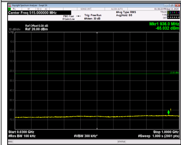
2-2-5MHz-20MHz-16QAM-16QAM-18808-18925-25RB#0 -100RB#0-30~1000MHz-PASS
