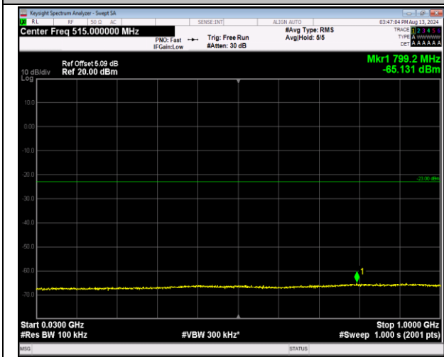
2-2-20MHz-20MHz-16QAM-16QAM-18700-18898-100RB #0-100RB#0-30~1000MHz-PASS
