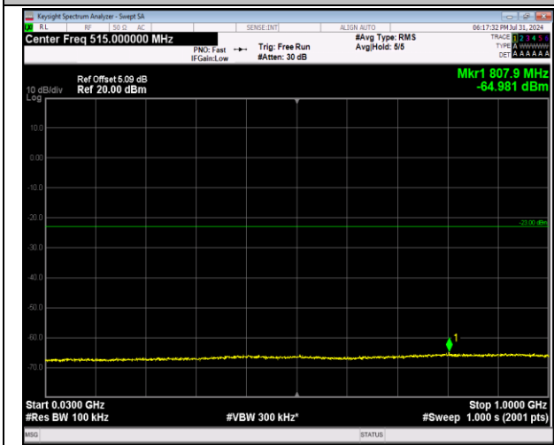
2-2-5MHz-20MHz-64QAM-64QAM-18983-19100-1RB#24-0RB#0-30~1000MHz-PASS
