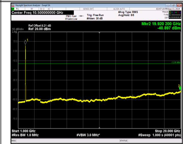
2-2-20MHz-20MHz-16QAM-16QAM-18700-18898-100RB#0 -100RB#0-1000~20000MHz-PASS
