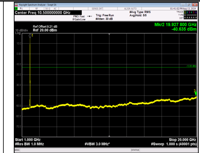
2-2-5MHz-20MHz-QPSK-QPSK-18983-19100-25RB#0-100 RB#0-1000~20000MHz-PASS
