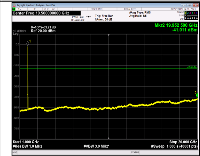
2-2-20MHz-20MHz-64QAM-64QAM-18801-18999-100RB#0-100RB#0-1000~20000MHz-PASS
