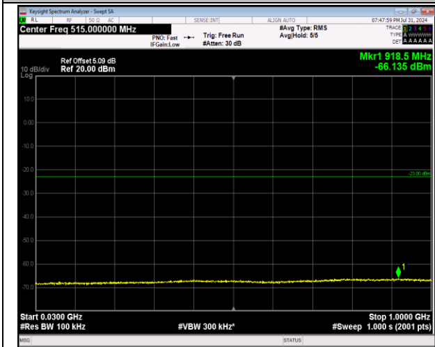
2-2-20MHz-20MHz-64QAM-64QAM-18700-18898-1RB#0 -ORB#0-30~1000MHz-PASS
