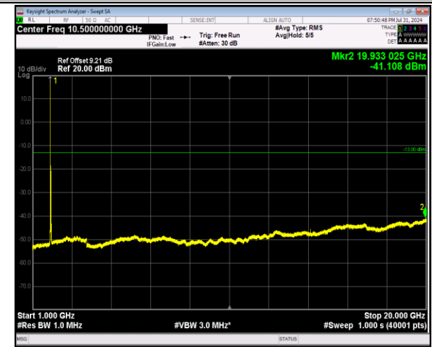
2-2-20MHz-20MHz-64QAM-64QAM-18801-18999-1RB#0-0 RB#0-1000~20000MHz-PASS
