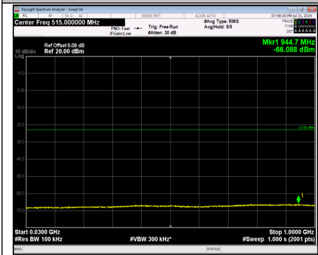
2-2-20MHz-20MHz-64QAM-64QAM-18700-18898-1RB#9 9-0RB#0-30~1000MHz-PASS
