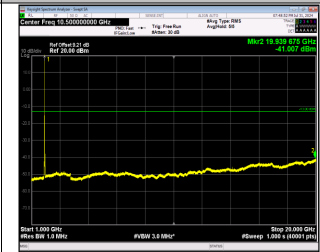
2-2-20MHz-20MHz-64QAM-64QAM-18700-18898-1RB#99-0RB#0-1000~20000MHz-PASS
