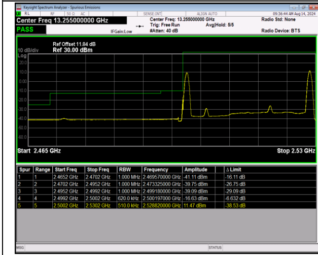
7-7-10MHz-20MHz-QPSK@QPSK-QPSK@QPSK-20805- 20949-1RB#0@50RB#0-1RB#99@100RB#0-PASS
