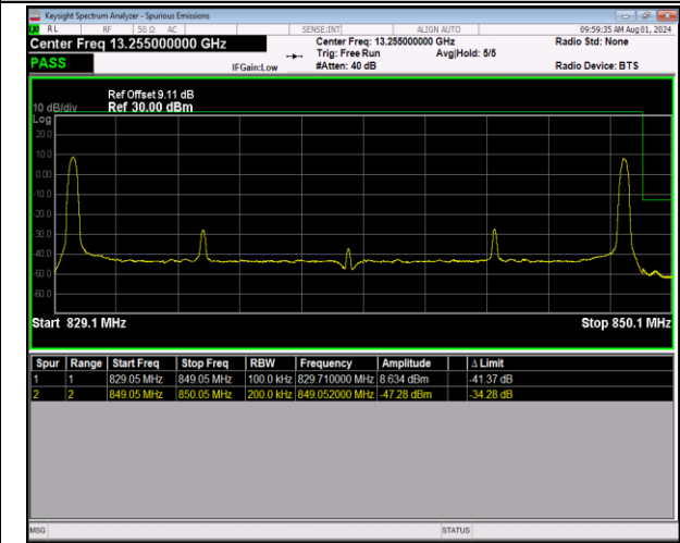
5-5-10MHz-10MHz-64QAM@64QAM-64QAM@64QAM-2 0501-20600-1RB#0@50RB#0-1RB#49@50RB#0-PASS
