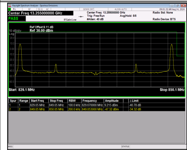
5-5-10MHz-10MHz-QPSK@QPSK-QPSK@QPSK-20501- 20600-1RB#0@50RB#0-1RB#49@50RB#0-PASS
