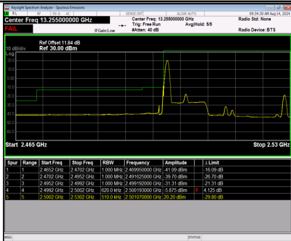
7-7-10MHz-20MHz-16QAM@16QAM-16QAM@16QAM-20805-20949-1RB#0@50RB#0-0RB#0@100RB#0-FAIL
