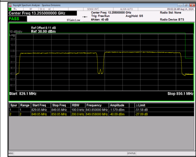
5-5-10MHz-10MHz-QPSK@QPSK-QPSK@QPSK-20501- 20600-50RB#0@50RB#0-50RB#0@50RB#0-PASS
