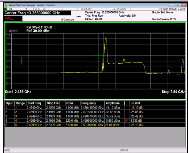
7-7-20MHz-20MHz-QPSK@QPSK-QPSK@QPSK-20850-
