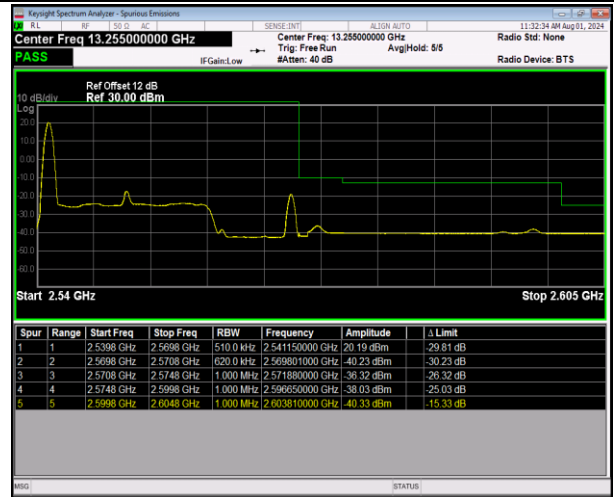
7-7-20MHz-10MHz-64QAM@64QAM-64QAM@64QAM-2 1251-21395-1RB#0@100RB#0-0RB#0@50RB#0-PASS
