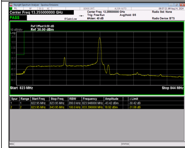
5-5-10MHz-10MHz-16QAM@16QAM-16QAM@16QAM-2 0450-20549-1RB#49@50RB#0-0RB#0@50RB#0-PASS
