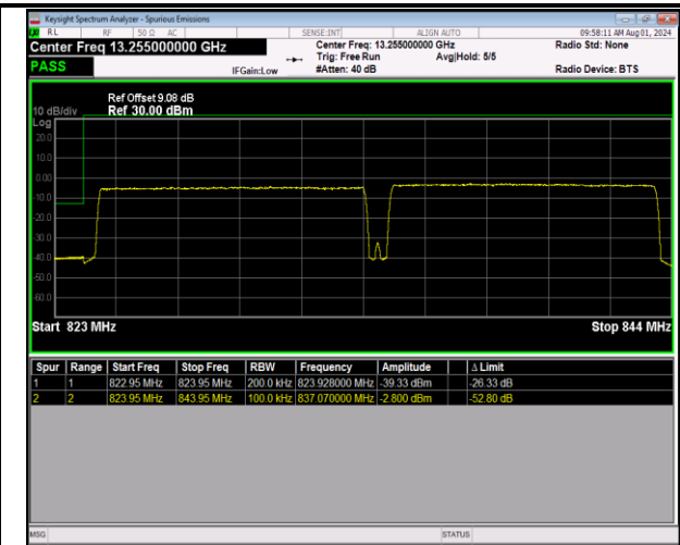
5-5-10MHz-10MHz-64QAM@64QAM-64QAM@64QAM-2 0450-20549-50RB#0@50RB#0-50RB#0@50RB#0-PASS
