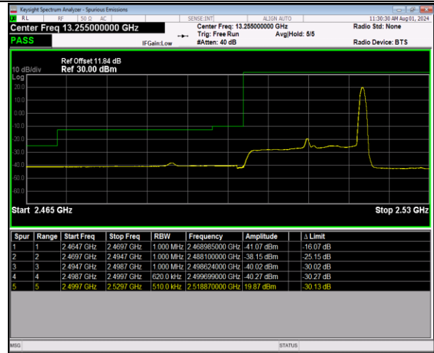
7-7-20MHz-10MHz-64QAM@64QAM-64QAM@64QAM-2 0850-20994-1RB#99@100RB#0-0RB#0@50RB#0-PASS
