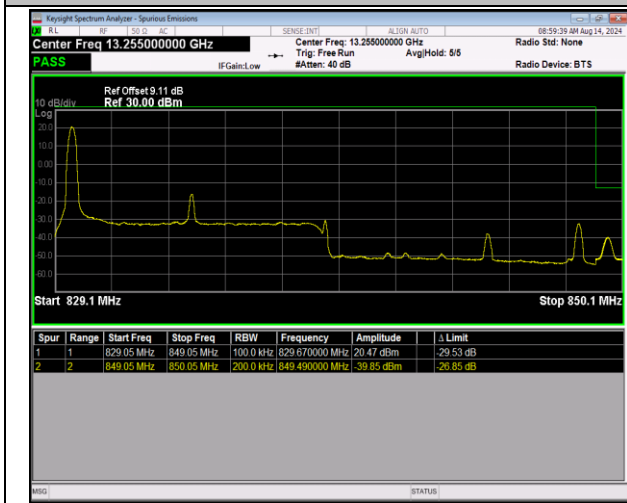
5-5-10MHz-10MHz-QPSK@QPSK-QPSK@QPSK-20501- 20600-1RB#0@50RB#0-0RB#0@50RB#0-PASS
