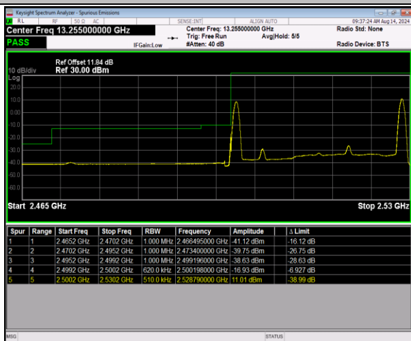
7-7-10MHz-20MHz-16QAM@16QAM-16QAM@16QAM-20805-20949-1RB#0@50RB#0-1RB#99@100RB#0-PASS
