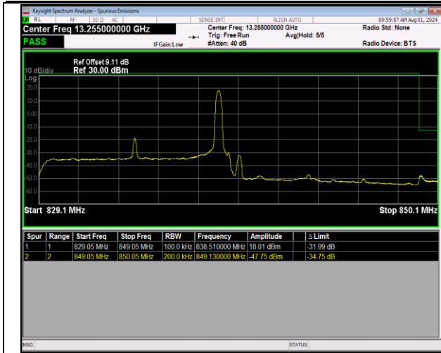
5-5-10MHz-10MHz-64QAM@64QAM-64QAM@64QAM-2 0501-20600-1RB#49@50RB#0-0RB#0@50RB#0-PASS
