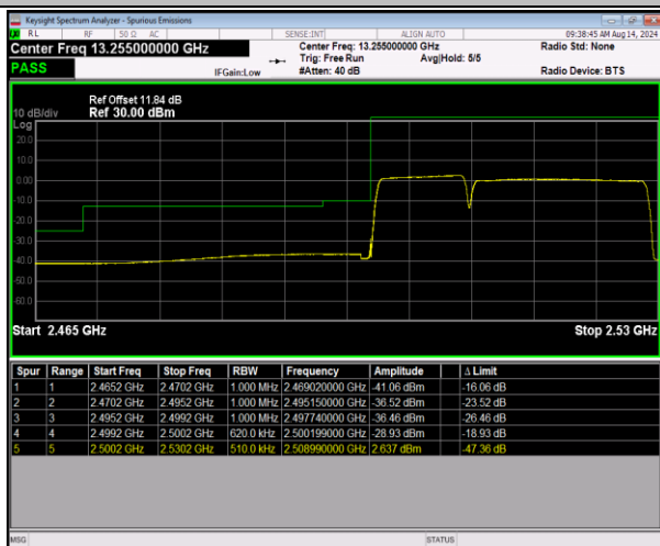
7-7-10MHz-20MHz-16QAM@16QAM-16QAM@16QAM-20805-20949-50RB#0@50RB#0-100RB#0@100RB#0-PASS
