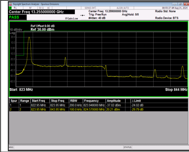
5-5-10MHz-10MHz-QPSK@QPSK-QPSK@QPSK-20450- 20549-1RB#0@50RB#0-0RB#0@50RB#0-PASS
