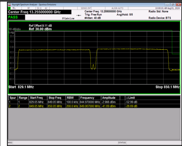
5-5-10MHz-10MHz-64QAM@64QAM-64QAM@64QAM-2 0501-20600-50RB#0@50RB#0-50RB#0@50RB#0-PASS
