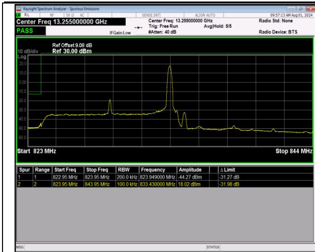
5-5-10MHz-10MHz-64QAM@64QAM-64QAM@64QAM-2 0450-20549-1RB#49@50RB#0-0RB#0@50RB#0-PASS
