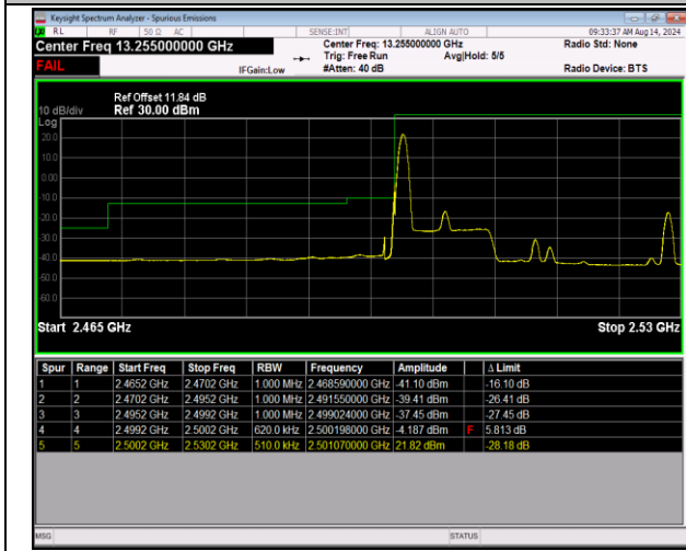
7-7-10MHz-20MHz-QPSK@QPSK-QPSK@QPSK-20805- 20949-1RB#0@50RB#0-0RB#0@100RB#0-FAIL
