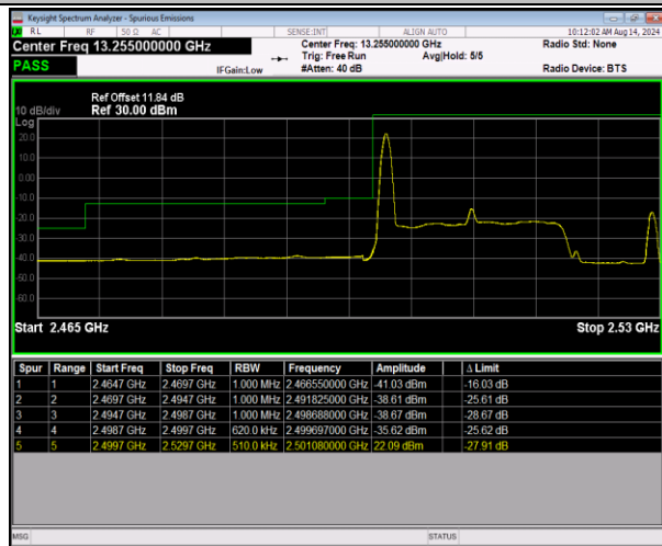
7-7-20MHz-10MHz-QPSK@QPSK-QPSK@QPSK-20850-
