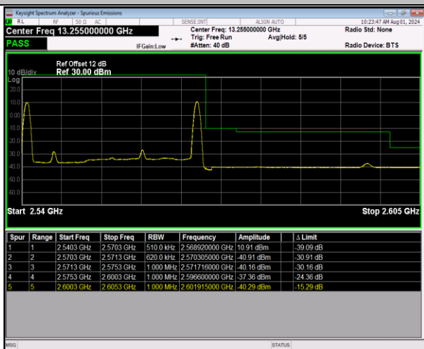
7-7-10MHz-20MHz-64QAM@64QAM-64QAM@64QAM-2 1206-21350-1RB#0@50RB#0-1RB#99@100RB#0-PASS
