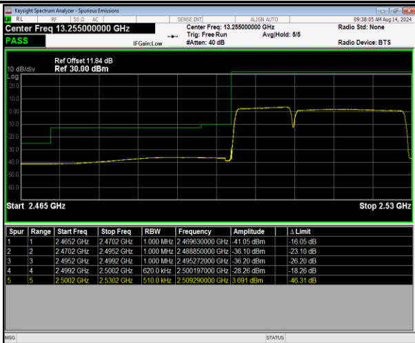
7-7-10MHz-20MHz-QPSK@QPSK-QPSK@QPSK-20805-20949-50RB#0@50RB#0-100RB#0@100RB#0-PASS
