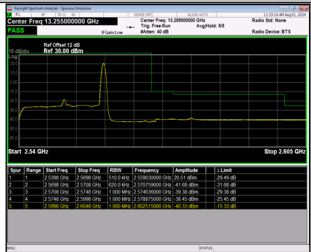
7-7-20MHz-10MHz-64QAM@64QAM-64QAM@64QAM-2 1251-21395-1RB#99@100RB#0-0RB#0@50RB#0-PASS
