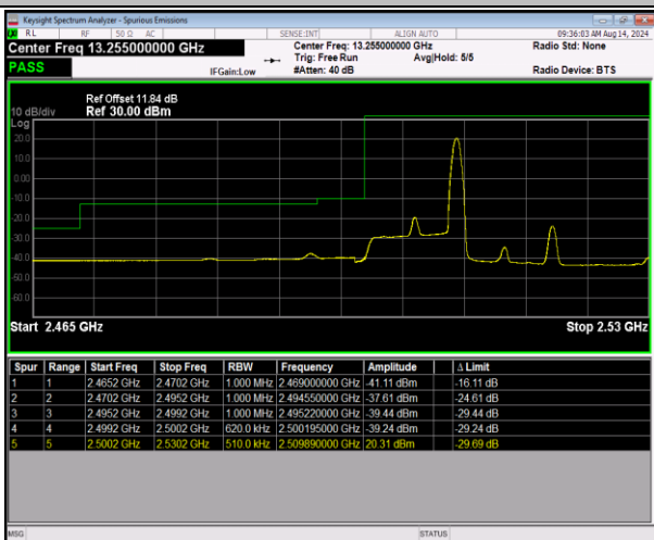
7-7-10MHz-20MHz-16QAM@16QAM-16QAM@16QAM-20805-20949-1RB#49@50RB#0-0RB#0@100RB#0-PASS
