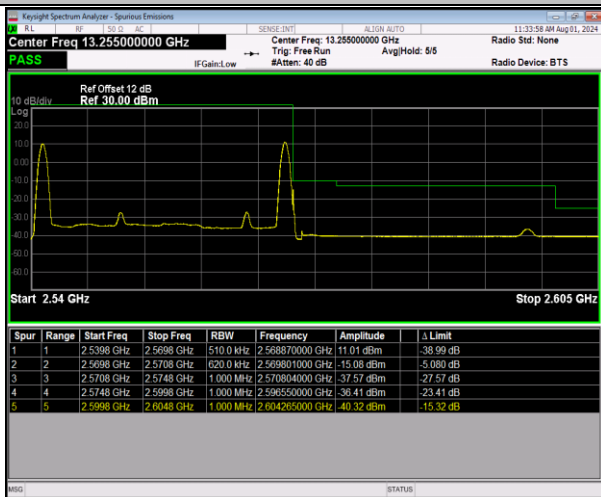
7-7-20MHz-10MHz-64QAM@64QAM-64QAM@64QAM-2 1251-21395-1RB#0@100RB#0-1RB#49@50RB#0-PASS
