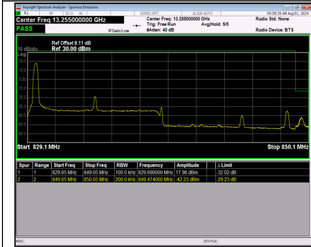
5-5-10MHz-10MHz-64QAM@64QAM-64QAM@64QAM-2 0501-20600-1RB#0@50RB#0-0RB#0@50RB#0-PASS
