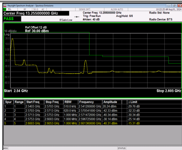
7-7-10MHz-20MHz-64QAM@64QAM-64QAM@64QAM-2 1206-21350-1RB#0@50RB#0-0RB#0@100RB#0-PASS
