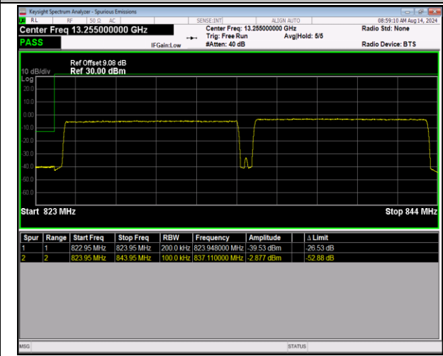
5-5-10MHz-10MHz-16QAM@16QAM-16QAM@16QAM-2 0450-20549-50RB#0@50RB#0-50RB#0@50RB#0-PASS
