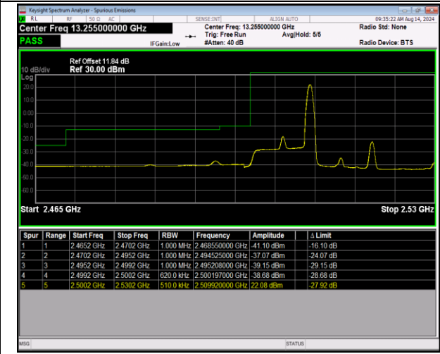
7-7-10MHz-20MHz-QPSK@QPSK-QPSK@QPSK-20805- 20949-1RB#49@50RB#0-0RB#0@100RB#0-PASS
