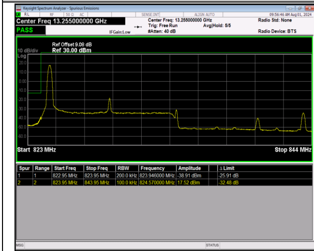
5-5-10MHz-10MHz-64QAM@64QAM-64QAM@64QAM-2 0450-20549-1RB#0@50RB#0-0RB#0@50RB#0-PASS
