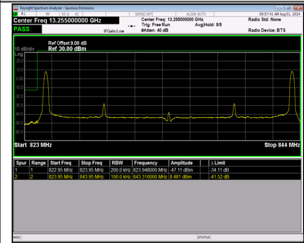
5-5-10MHz-10MHz-64QAM@64QAM-64QAM@64QAM-2 0450-20549-1RB#0@50RB#0-1RB#49@50RB#0-PASS
