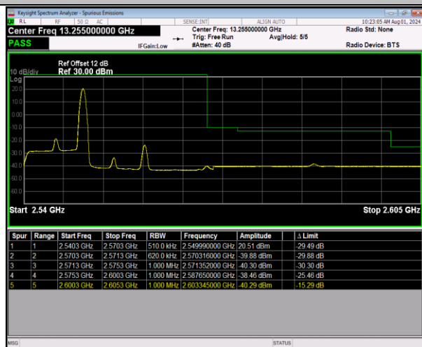
7-7-10MHz-20MHz-64QAM@64QAM-64QAM@64QAM-2 1206-21350-1RB#49@50RB#0-0RB#0@100RB#0-PASS
