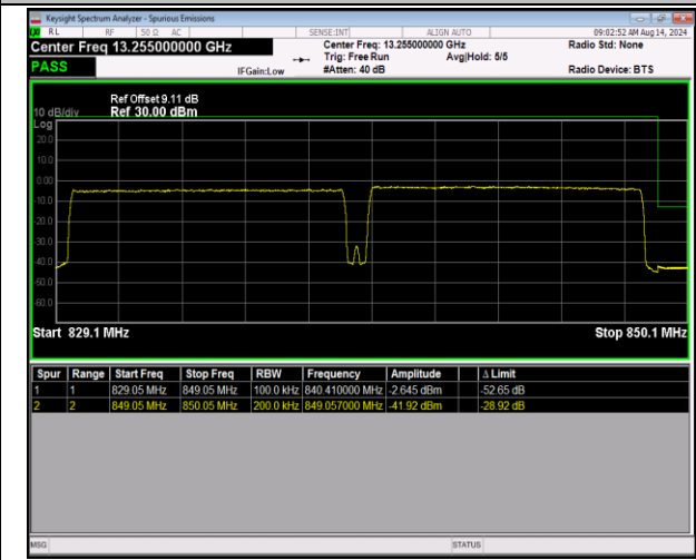
5-5-10MHz-10MHz-16QAM@16QAM-16QAM@16QAM-2 0501-20600-50RB#0@50RB#0-50RB#0@50RB#0-PASS
