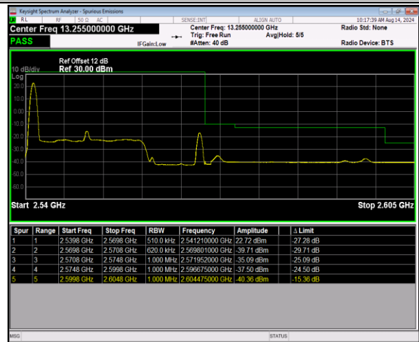
7-7-20MHz-10MHz-QPSK@QPSK-QPSK@QPSK-21251-
