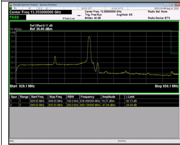
5-5-10MHz-10MHz-16QAM@16QAM-16QAM@16QAM-2 0501-20600-1RB#49@50RB#0-0RB#0@50RB#0-PASS
