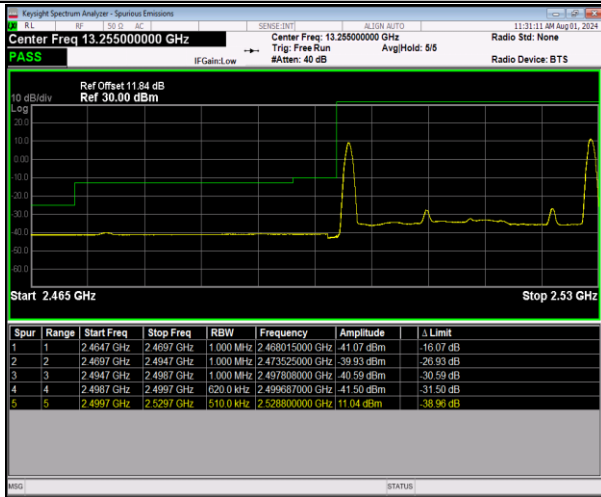
7-7-20MHz-10MHz-64QAM@64QAM-64QAM@64QAM-2 0850-20994-1RB#0@100RB#0-1RB#49@50RB#0-PASS
