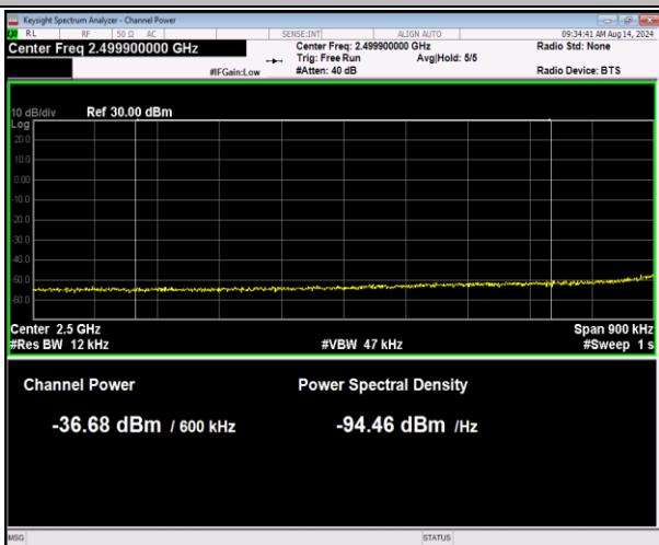
7-7-10MHz-20MHz-16QAM@16QAM-16QAM@16QAM-20805-20949-1RB#0@50RB#0-0RB#0@100RB#0-PASS_Final1
