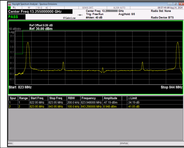
5-5-10MHz-10MHz-QPSK@QPSK-QPSK@QPSK-20450- 20549-1RB#0@50RB#0-1RB#49@50RB#0-PASS
