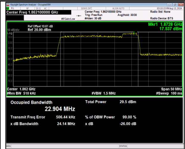
2-2-20MHz-5MHz-16QAM-16QAM-18700-18817-100RB #0-25RB#0-PASS
