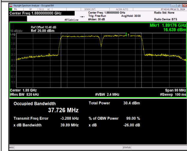
2-2-20MHz-20MHz-64QAM-64QAM-18801-18999-100RB#0-100RB#0-PASS
