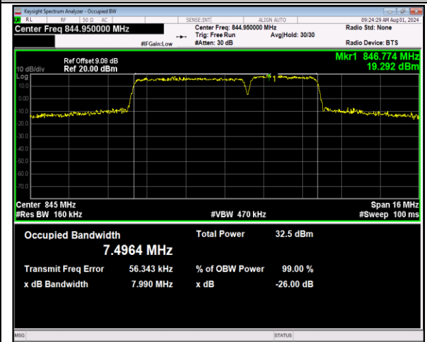
5-5-5MHz-3MHz-64QAM-64QAM-20595-20634-25RB#0-15 -15RB#0-PASS
