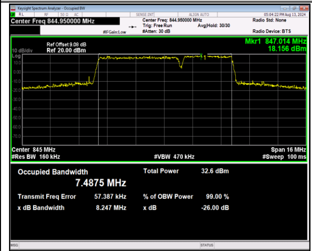
5-5-5MHz-3MHz-QPSK-QPSK-20595-20634-25RB#0-15 RB#0-PASS
