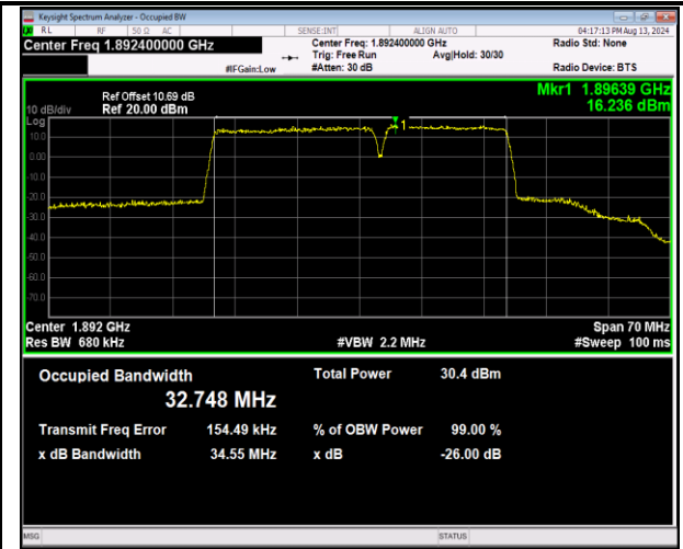
2-2-20MHz-15MHz-16QAM-16QAM-18951-19122-100RB#0-75RB#0-PASS
