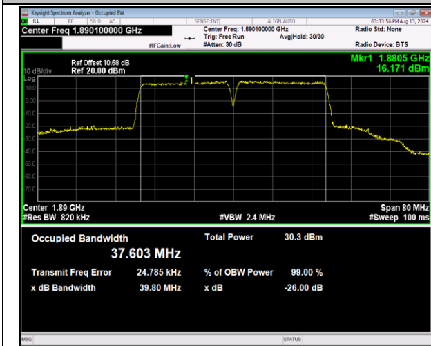
2-2-20MHz-20MHz-16QAM-16QAM-18902-19100-100RB#0-100RB#0-PASS
