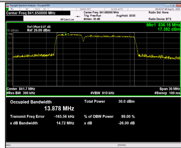
5-5-5MHz-10MHz-64QAM-64QAM-20528-20600-25RB#0-50RB#0-PASS
