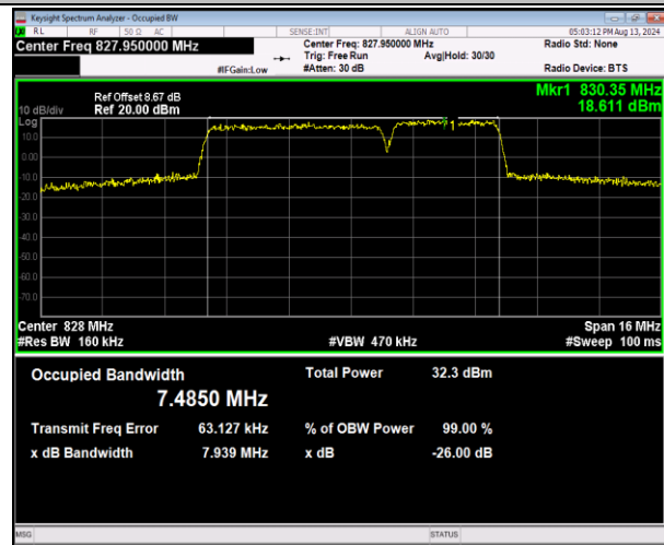
5-5-5MHz-3MHz-16QAM-16QAM-20425-20464-25RB#0-1 5RB#0-PASS
