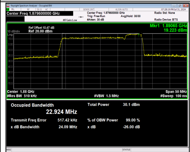
2-2-20MHz-5MHz-64QAM-64QAM-18875-18992-100RB #0-25RB#0-PASS
