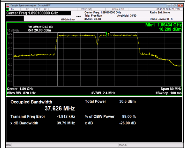
2-2-20MHz-20MHz-64QAM-64QAM-18902-19100-100RB#0-100RB#0-PASS
