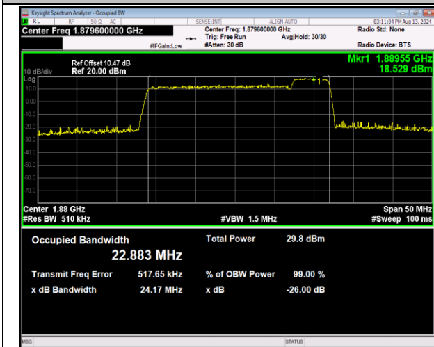
2-2-20MHz-5MHz-16QAM-16QAM-18875-18992-100RB#0-25RB#0-PASS
