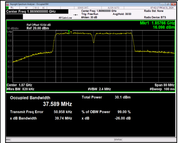
2-2-20MHz-20MHz-64QAM-64QAM-18700-18898-100RB#0-100RB#0-PASS
