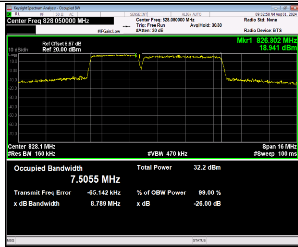
5-5-3MHz-5MHz-64QAM-64QAM-20416-20455-15RB#0-25 5RB#0-PASS
