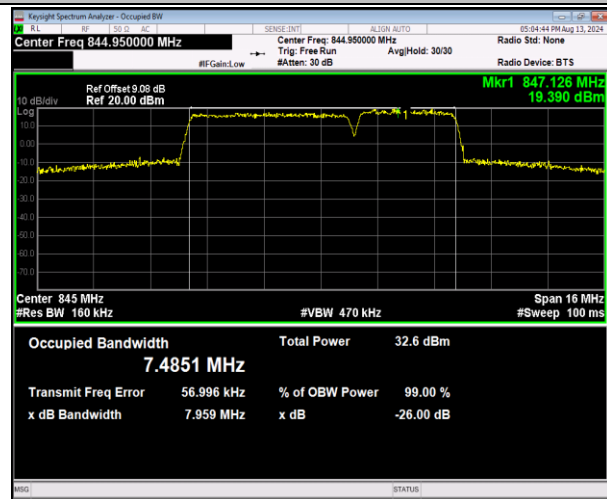
5-5-5MHz-3MHz-16QAM-16QAM-20595-20634-25RB#0-15 5RB#0-PASS
