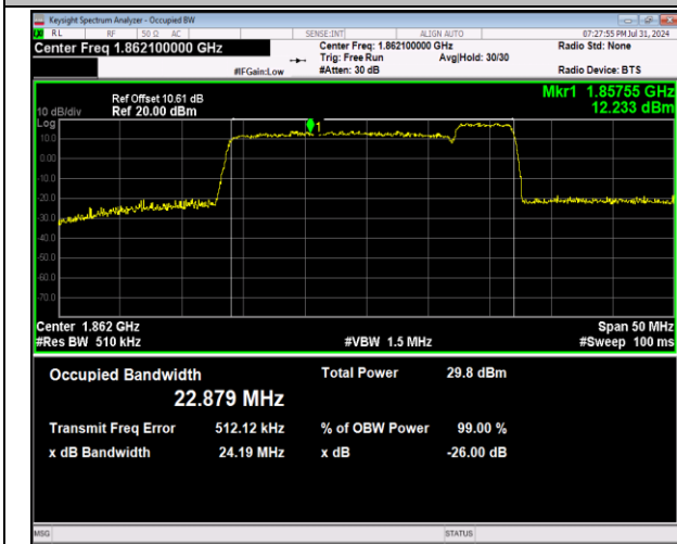
2-2-20MHz-5MHz-64QAM-64QAM-18700-18817-100RB#0-25RB#0-PASS
