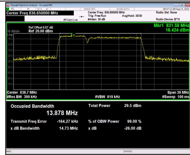
5-5-5MHz-10MHz-16QAM-16QAM-20478-20550-25RB#0-50RB#0-PASS
