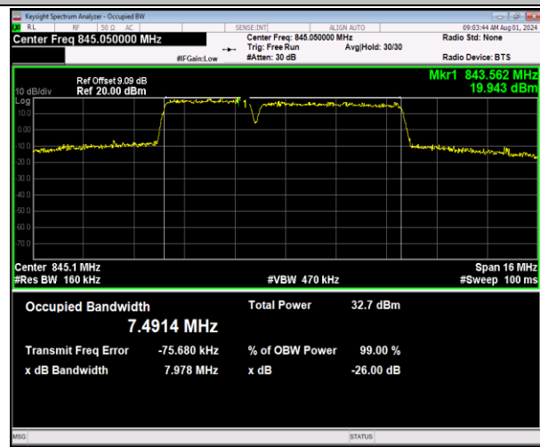
5-5-3MHz-5MHz-64QAM-64QAM-20586-20625-15RB#0-2 5RB#0-PASS
