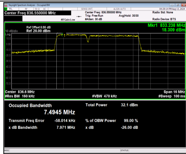
5-5-3MHz-5MHz-16QAM-16QAM-20501-20540-15RB#0-25 5RB#0-PASS
