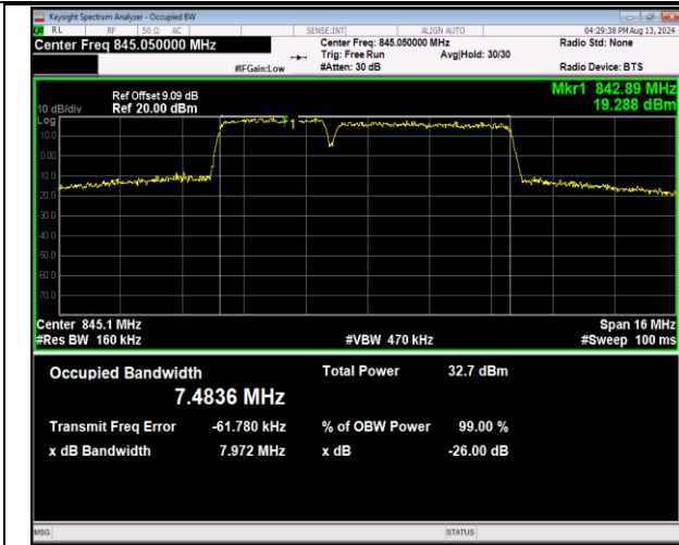
5-5-3MHz-5MHz-QPSK-QPSK-20586-20625-15RB#0-25 RB#0-PASS
