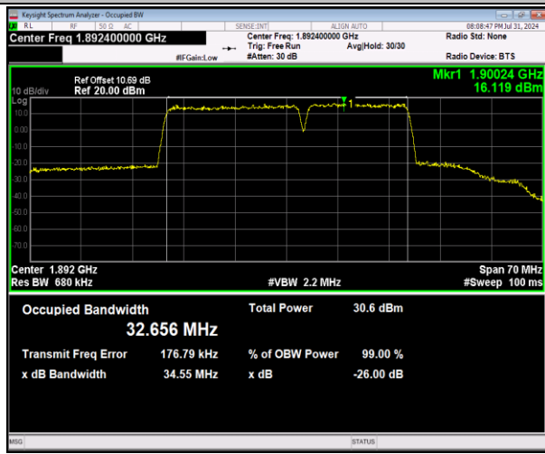
2-2-20MHz-15MHz-64QAM-64QAM-18951-19122-100RB#0-75RB#0-PASS
