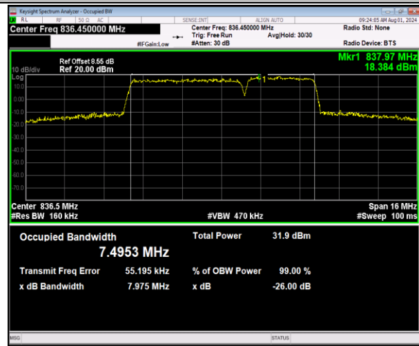
5-5-5MHz-3MHz-64QAM-64QAM-20510-20549-25RB#0-15 5RB#0-PASS
