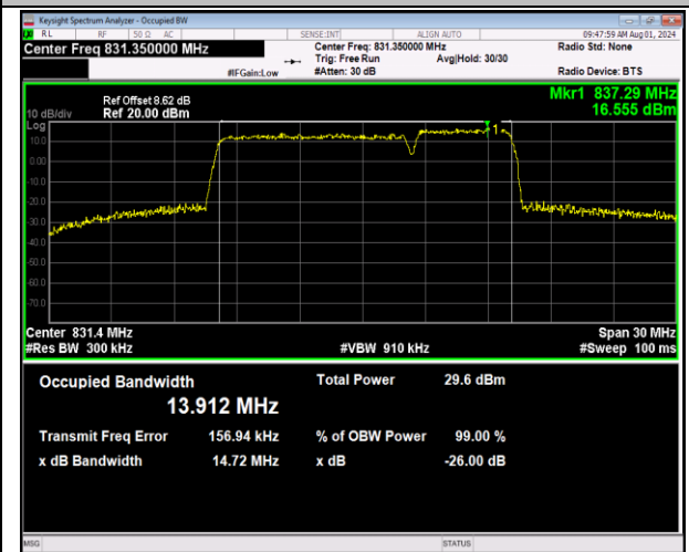
5-5-10MHz-5MHz-64QAM-64QAM-20450-20522-50RB#0-0-25RB#0-PASS
