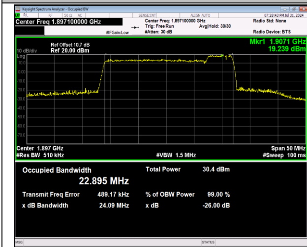
2-2-20MHz-5MHz-64QAM-64QAM-19050-19167-100RB# 0-25RB#0-PASS
