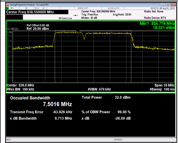
5-5-3MHz-5MHz-64QAM-64QAM-20501-20540-15RB#0-25 -25RB#0-PASS
