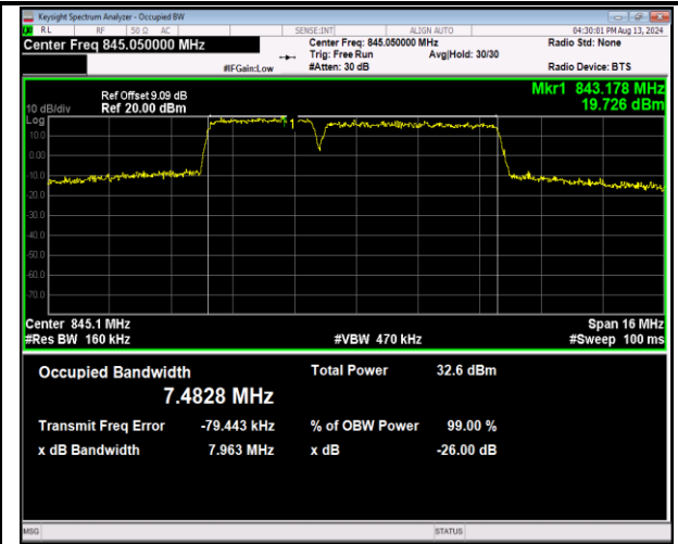
5-5-3MHz-5MHz-16QAM-16QAM-20586-20625-15RB#0-80 -25RB#0-PASS
