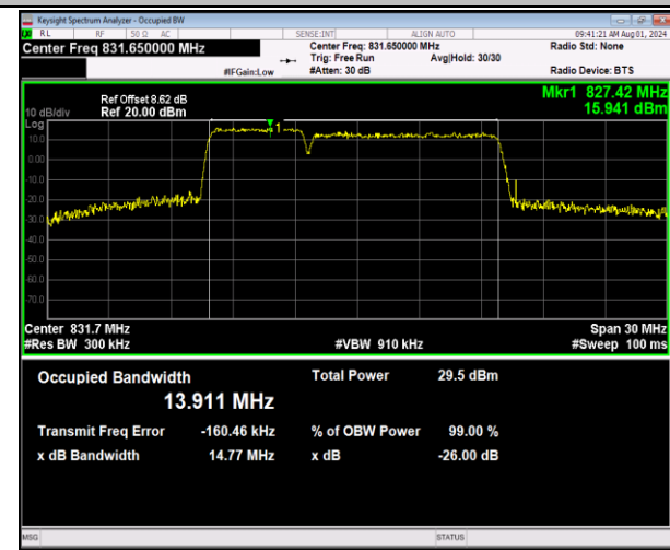
5-5-5MHz-10MHz-64QAM-64QAM-20428-20500-25RB#0-50RB#0-PASS
