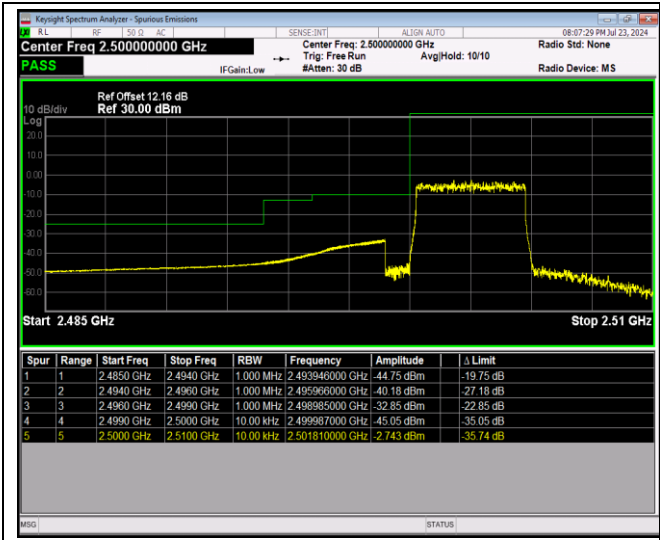
Band7-5MHz-64QAM-20775-25RB#0
