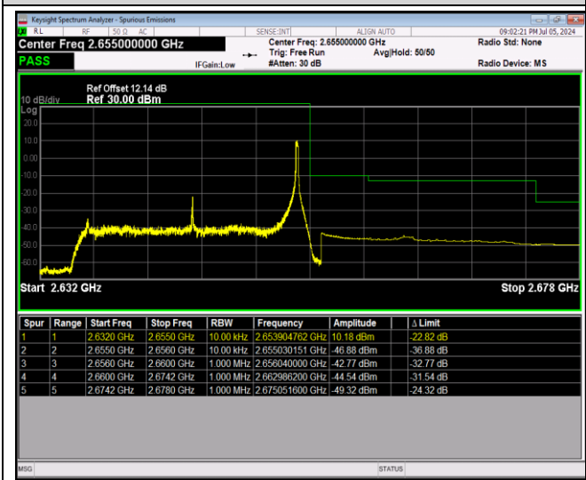
Band41-20MHz-16QAM-40140-1RB#0
