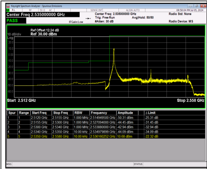
Band41-20MHz-QPSK-40140-100RB#0
