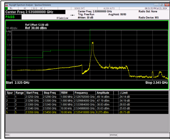
Band41-5MHz-64QAM-40065-25RB#0
