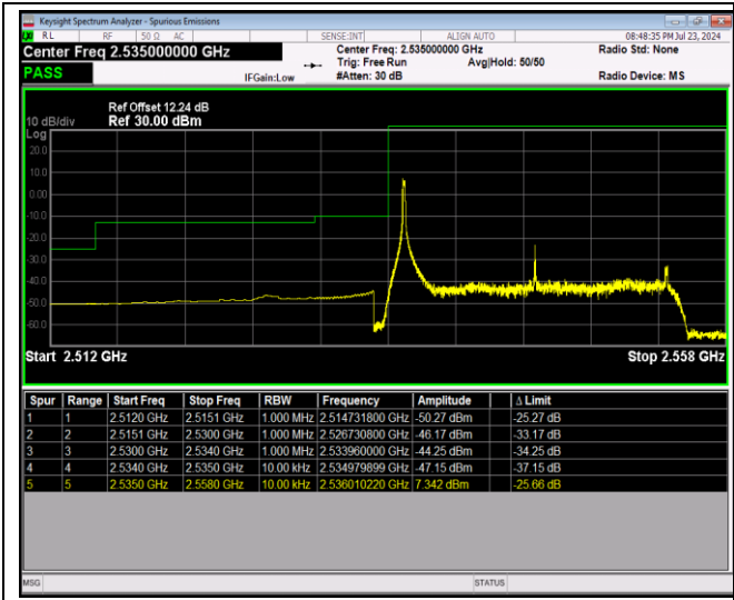
Band41-20MHz-64QAM-40140-100RB#0
