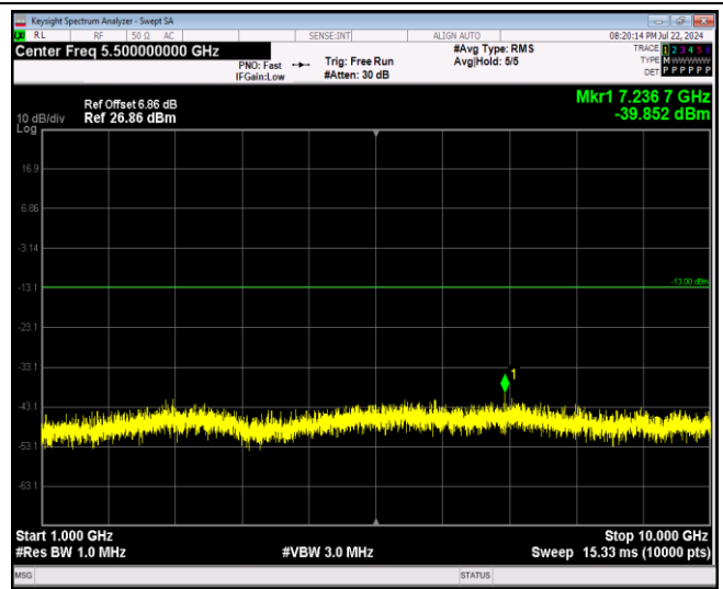
Band5-10MHz-64QAM-20600-1RB#0-Range2:1000~10000MHz
