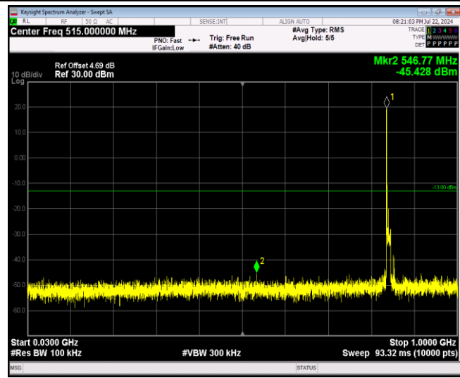
Band7-5MHz-QPSK-20775-1RB#0-Range1:30~1000MHz
