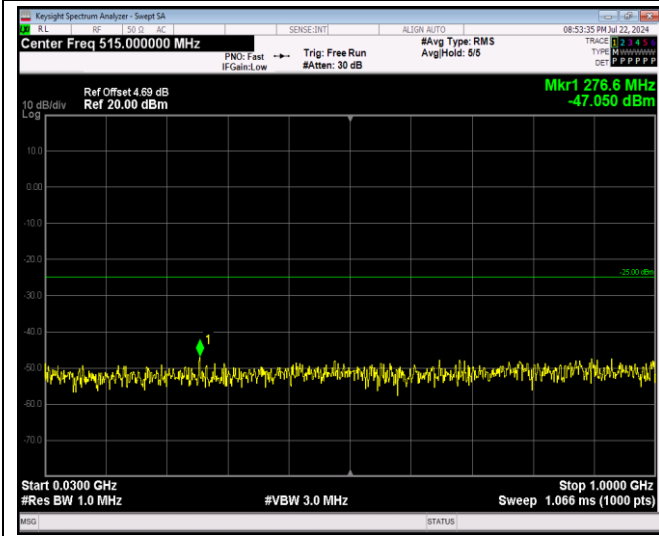
Band7-20MHz-QPSK-21100-1RB#0-Range1:30~100 OMHz
