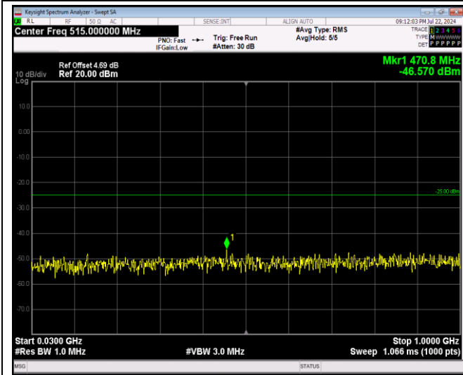
Band41-5MHz-64QAM-40640-1RB#0-Range1:30~1000MHz
