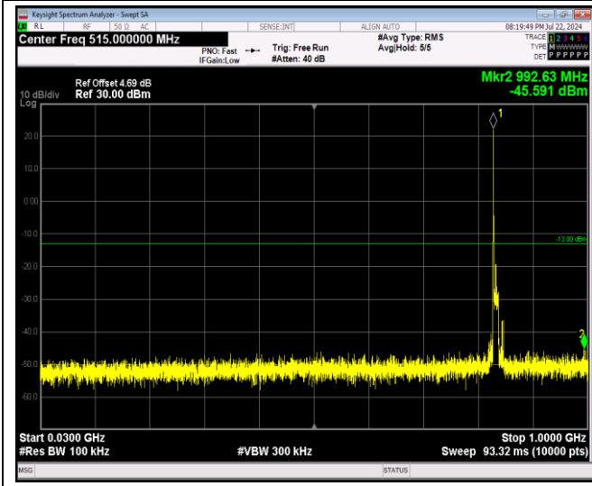
Band5-10MHz-16QAM-20525-1RB#0-Range1:30~1000MHz
