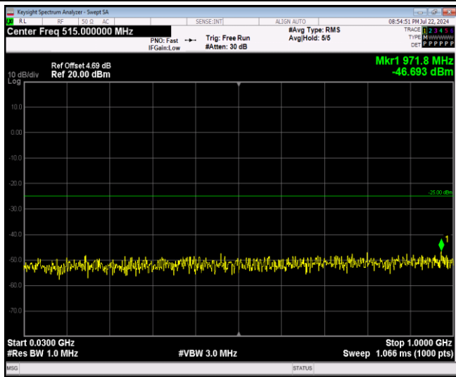
Band7-20MHz-64QAM-20850-1RB#0-Range1:30~1000MHz
