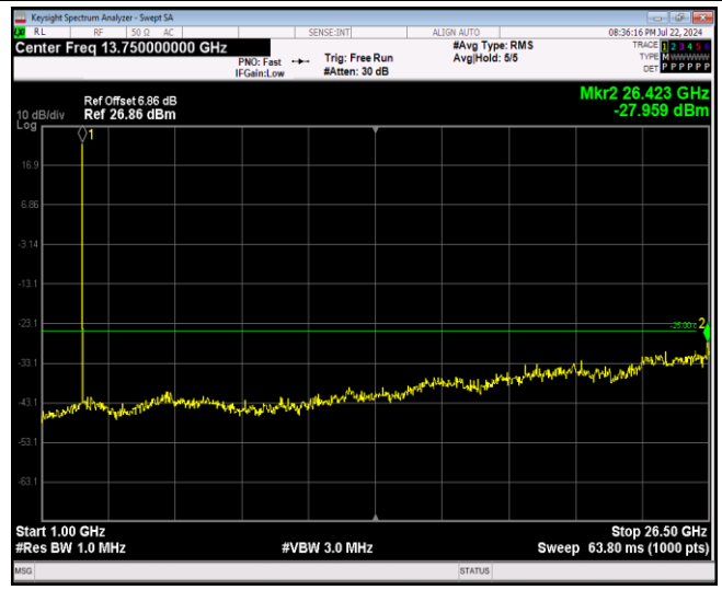
Band7-5MHz-16QAM-21425-1RB#0-Range2:1000~265 00MHz
