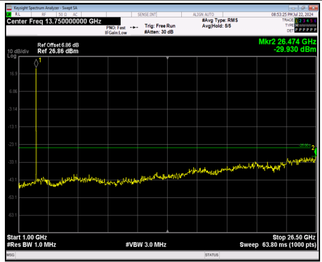
Band7-20MHz-64QAM-20850-1RB#0-Range2:1000~26500MHz
