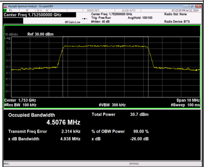
Band4-5MHz-64QAM-20175-25RB#0
