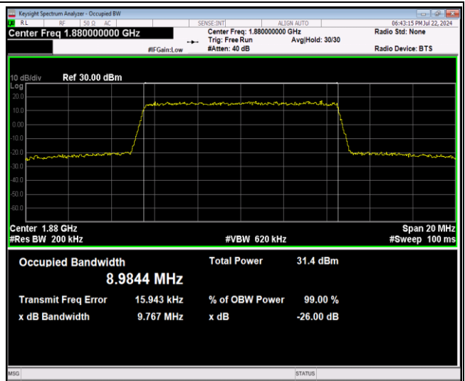
Band2-10MHz-64QAM-18650-50RB#0
