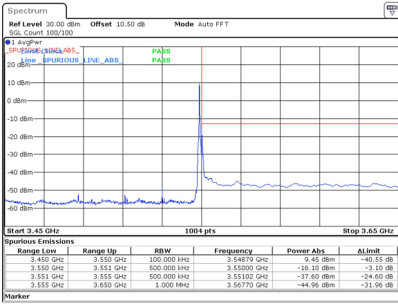
40MHz_30kHz_3530MHz_DFT-s-OFDM QPSK_RB1@105 -16.10 dBm
