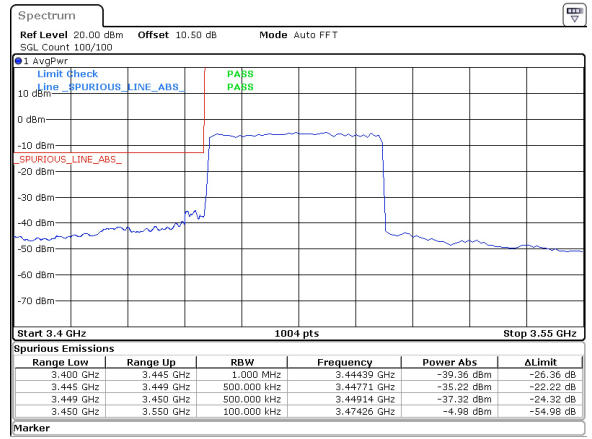
50MHz_30kHz_3475MHz_DFT-s-OFDM QPSK_RB128@0 -35.22 dBm
