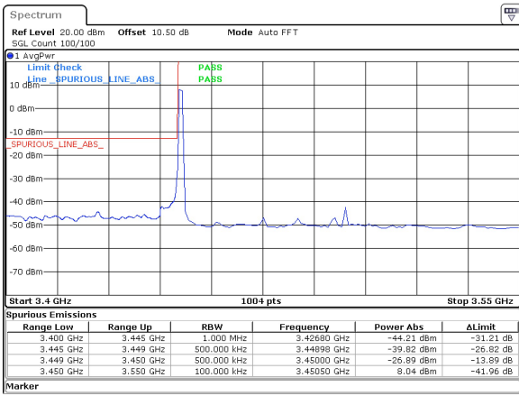
50MHz_15kHz_3475MHz_DFT-s-OFDM QPSK_RB1@0 -26.89 dBm
