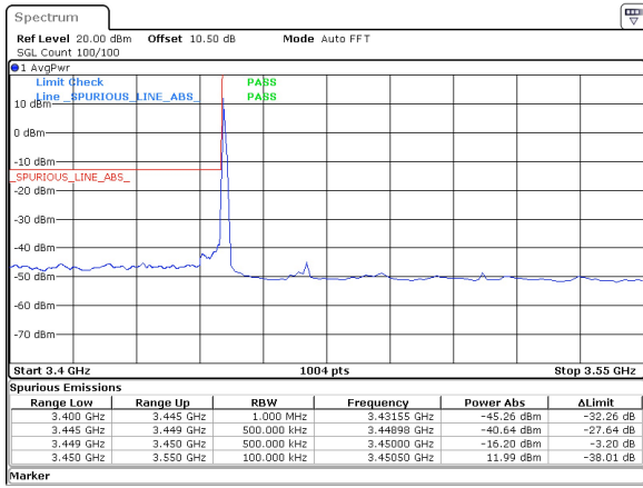
40MHz_15kHz_3470MHz_DFT-s-OFDM QPSK_RB1@0 -16.20 dBm
