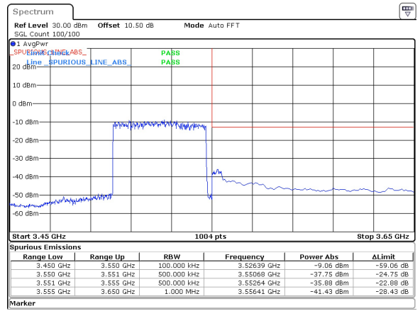
50MHz_30kHz_3525MHz_DFT-s-OFDM QPSK_RB128@0 -35.88 dBm
