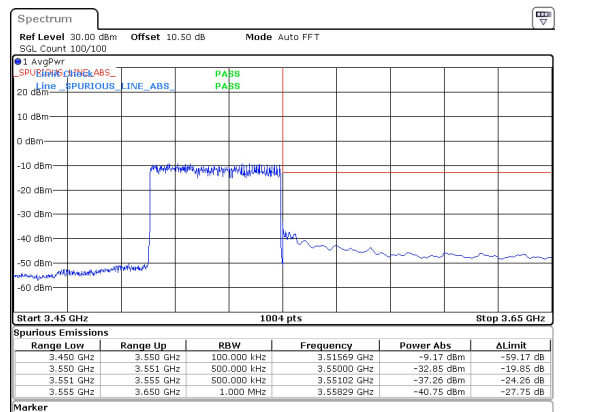
50MHz_15kHz_3525MHz_DFT-s-OFDM QPSK_RB270@0 -32.85 dBm
