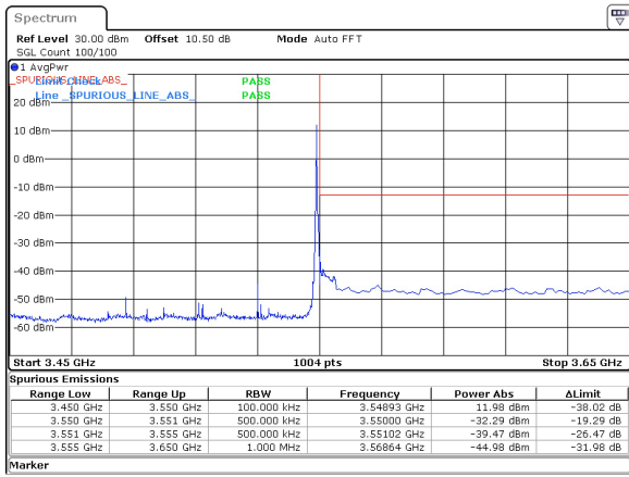
40MHz_15kHz_3530MHz_DFT-s-OFDM QPSK_RB1@215 -32.29 dBm
