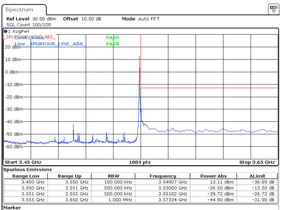
50MHz_15kHz_3525MHz_DFT-s-OFDM QPSK_RB1@269 -26.50 dBm
