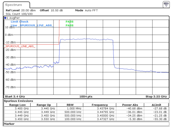
50MHz_15kHz_3475MHz_DFT-s-OFDM QPSK_RB270@0 -34.25 dBm
