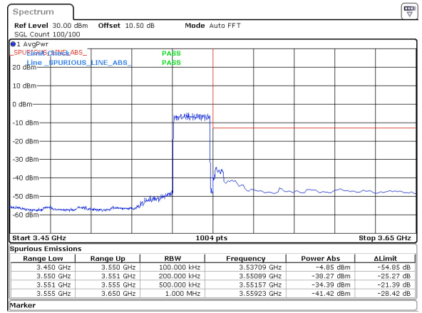
20MHz_15kHz_3540MHz_DFT-s-OFDM QPSK_RB100@0 -34.39 dBm
