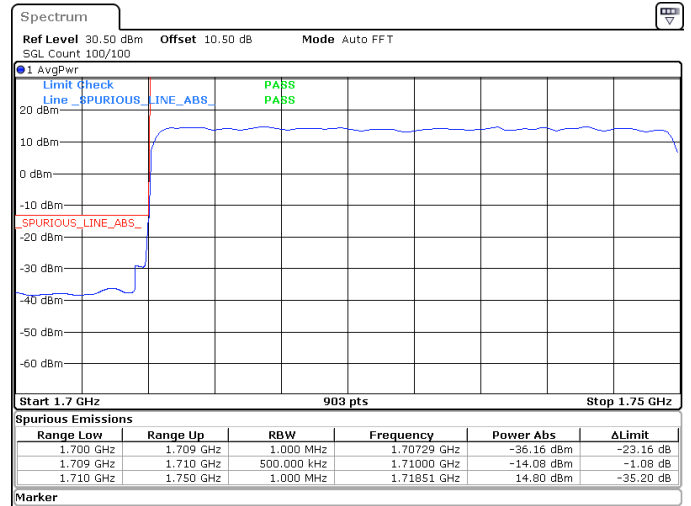
40MHz_15kHz_1730MHz_DFT-s-OFDM QPSK_RB216@0 -14.08 dBm
