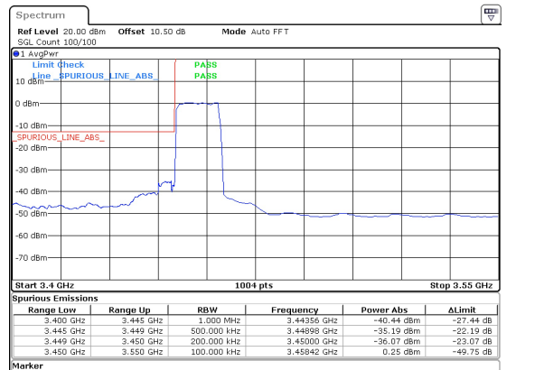
15MHz_15kHz_3457.5MHz_DFT-s-OFDM QPSK_RB75@0 -35.19 dBm
