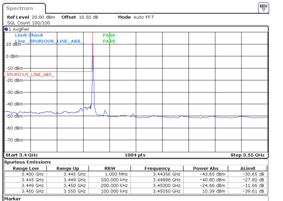
15MHz_15kHz_3457.5MHz_DFT-s-OFDM QPSK_RB1@0 -24.66 dBm
