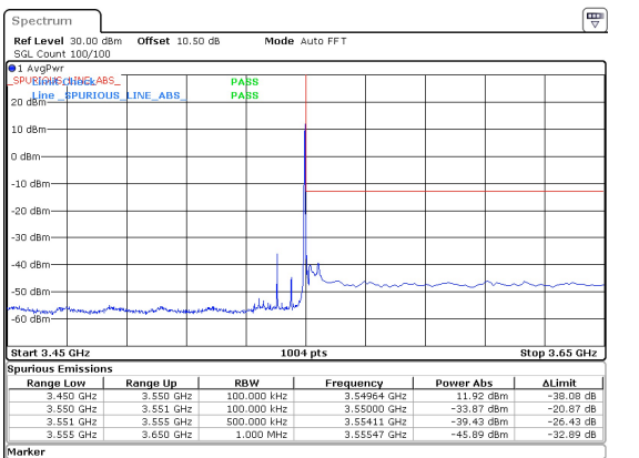
10MHz_15kHz_3545MHz_DFT-s-OFDM QPSK_RB1@51 -33.87 dBm
