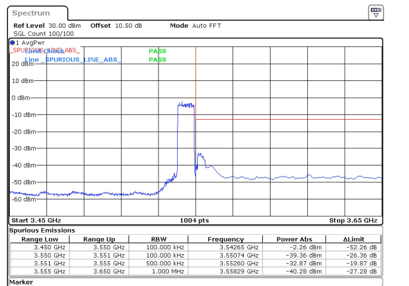
10MHz_15kHz_3545MHz_DFT-s-OFDM QPSK_RB50@0 -32.87 dBm
