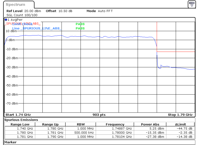
40MHz_15kHz_1760MHz_DFT-s-OFDM QPSK_RB216@0 -15.35 dBm
