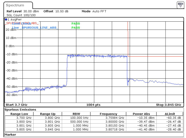
50MHz_15kHz_3775MHz_DFT-s-OFDM QPSK_RB270@0&-39.47 dBm
