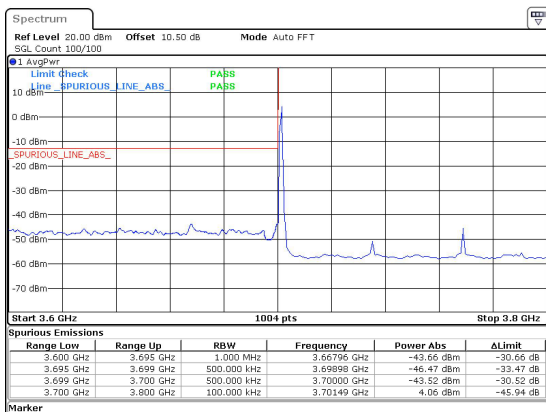
70MHz_30kHz_3735MHz_DFT-s-OFDM QPSK_RB1@0&-43.52 dBm
