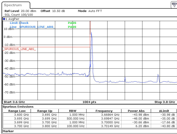
80MHz_30kHz_3740MHz_DFT-s-OFDM QPSK_RB1@0&-30.66 dBm
