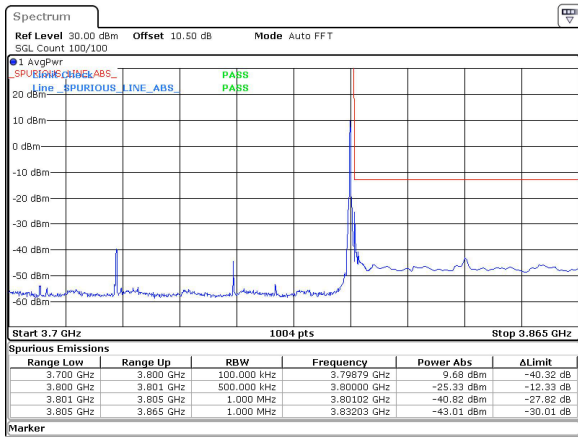
70MHz_30kHz_3765MHz_DFT-s-OFDM QPSK_RB1@188&-25.33 dBm
