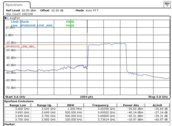
50MHz_30kHz_3725MHz_DFT-s-OFDM QPSK_RB128@0&-39.60 dBm
