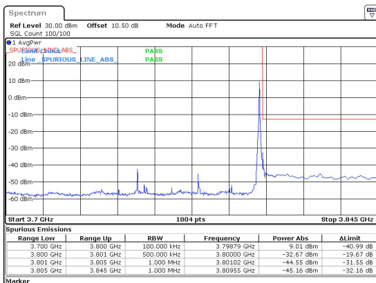
50MHz_30kHz_3775MHz_DFT-s-OFDM QPSK_RB1@132&-32.67 dBm
