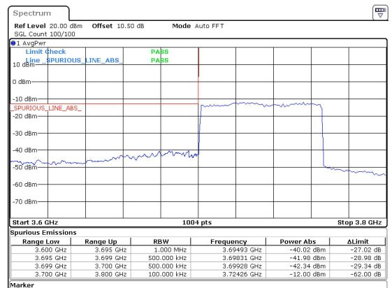
70MHz_30kHz_3735MHz_DFT-s-OFDM QPSK_RB180@0&-40.02 dBm
