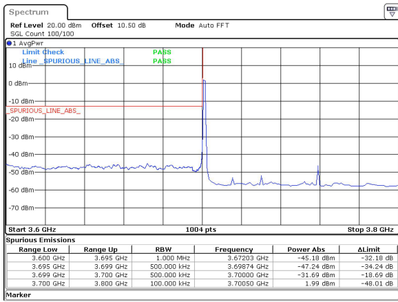
60MHz_30kHz_3730MHz_DFT-s-OFDM QPSK_RB1@0&-31.69 dBm
