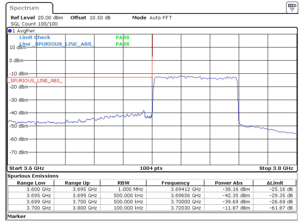
60MHz_30kHz_3730MHz_DFT-s-OFDM QPSK_RB162@0&-38.16 dBm
