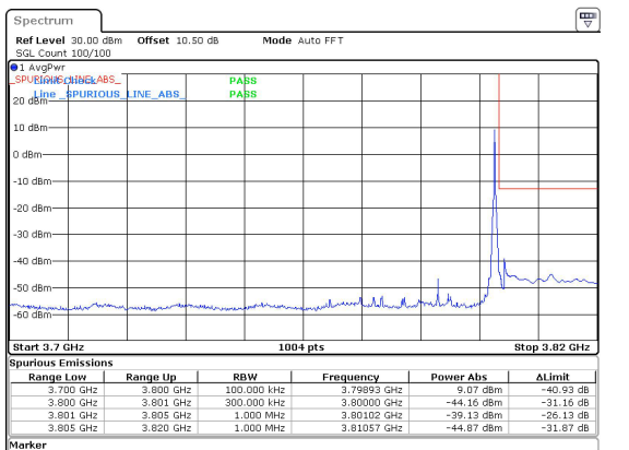
25MHz_30kHz_3787.5MHz_DFT-s-OFDM QPSK_RB1@64&-39.13 dBm
