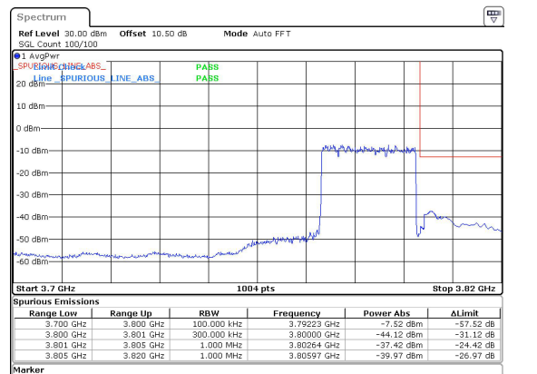
25MHz_30kHz_3787.5MHz_DFT-s-OFDM QPSK_RB64@0&-37.42 dBm
