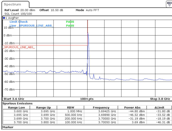
15MHz_30kHz_3707.5MHz_DFT-s-OFDM QPSK_RB1@0&-31.19 dBm
