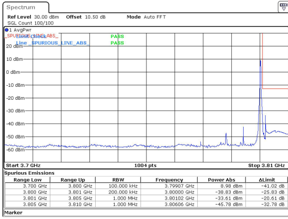
15MHz_30kHz_3792.5MHz_DFT-s-OFDM QPSK_RB1@37&-33.61 dBm
