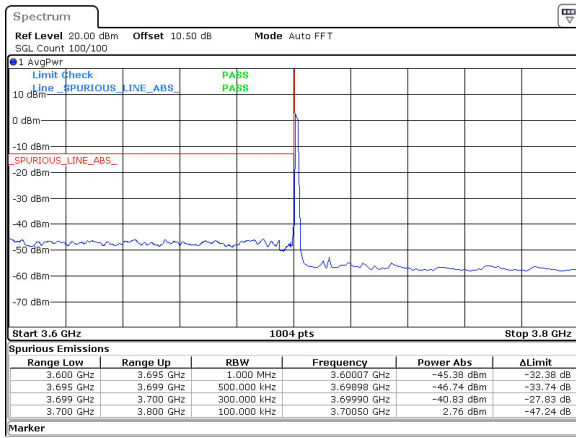
25MHz_30kHz_3712.5MHz_DFT-s-OFDM QPSK_RB1@0&-40.83 dBm
