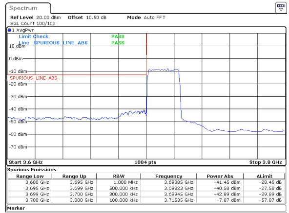
25MHz_30kHz_3712.5MHz_DFT-s-OFDM QPSK_RB64@0&-40.58 dBm
