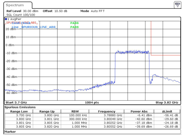
25MHz_15kHz_3787.5MHz_DFT-s-OFDM QPSK_RB128@0&-37.18 dBm
