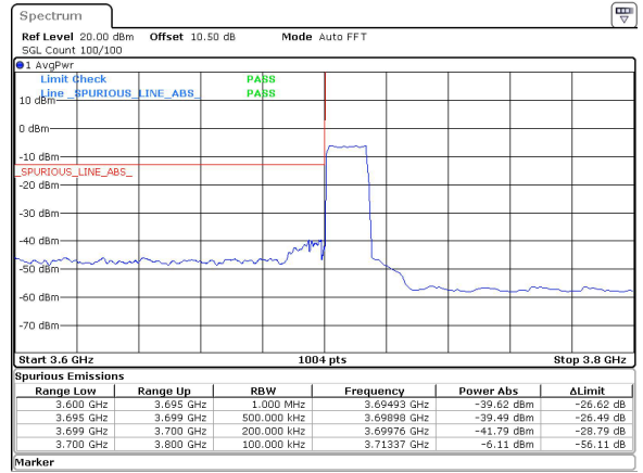
15MHz_15kHz_3707.5MHz_DFT-s-OFDM QPSK_RB75@0&-39.49 dBm
