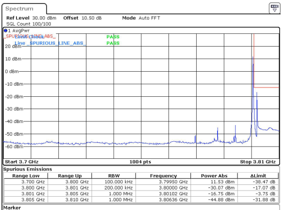
15MHz_15kHz_3792.5MHz_DFT-s-OFDM QPSK_RB1@78&-16.75 dBm
