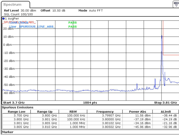
10MHz_30kHz_3795MHz_DFT-s-OFDM QPSK_RB1@23&-34.16 dBm
