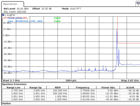
25MHz_15kHz_3787.5MHz_DFT-s-OFDM QPSK_RB1@132&-21.81 dBm
