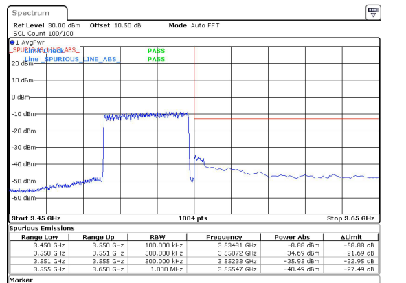
50MHz_30kHz_3525MHz_DFT-s-OFDM QPSK_RB128@0&-34.69 dBm
