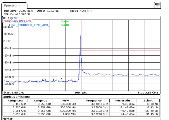
50MHz_30kHz_3525MHz_DFT-s-OFDM QPSK_RB1@132&-21.43 dBm
