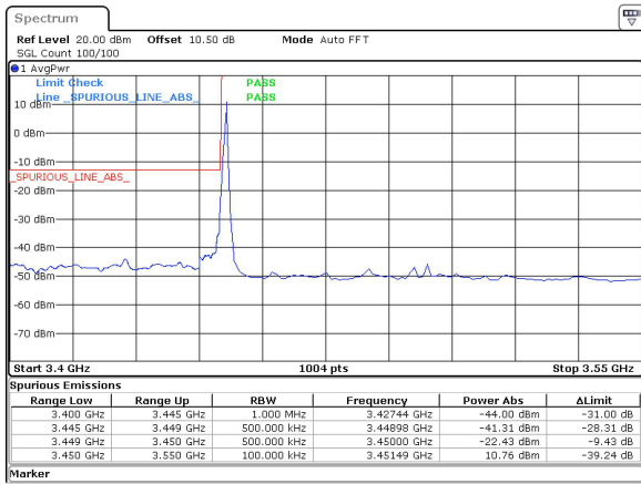
50MHz_30kHz_3475MHz_DFT-s-OFDM QPSK_RB1@0&-22.43 dBm
