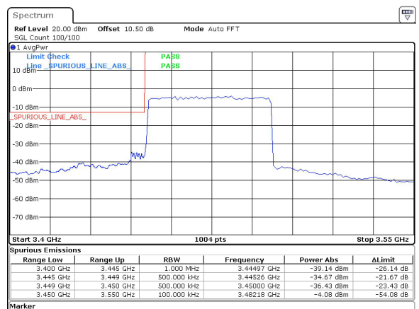
50MHz_30kHz_3475MHz_DFT-s-OFDM QPSK_RB128@0&-34.67 dBm
