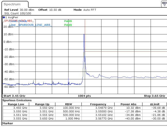
40MHz_30kHz_3530MHz_DFT-s-OFDM QPSK_RB1@105&-17.38 dBm
