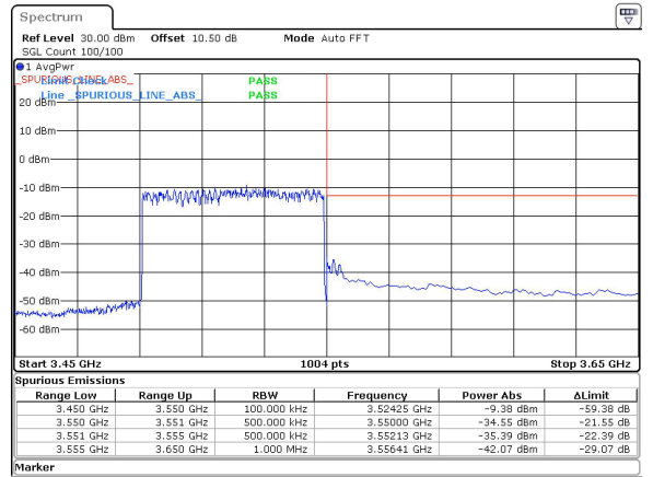
60MHz_30kHz_3520MHz_DFT-s-OFDM QPSK_RB162@0&-34.55 dBm
