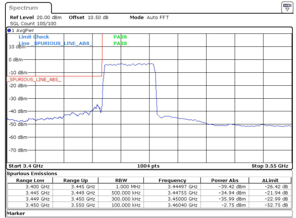
30MHz_30kHz_3465MHz_DFT-s-OFDM QPSK_RB75@0&-34.94 dBm
