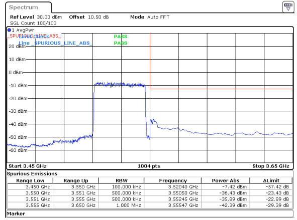
40MHz_30kHz_3530MHz_DFT-s-OFDM QPSK_RB100@0&-35.89 dBm
