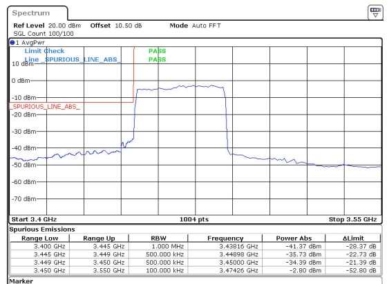
40MHz_30kHz_3470MHz_DFT-s-OFDM QPSK_RB100@0&-34.39 dBm
