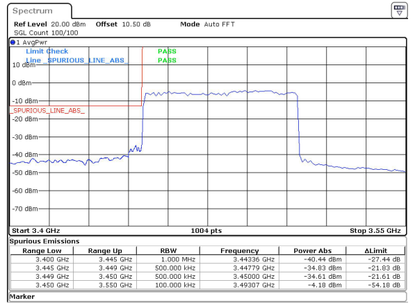
60MHz_30kHz_3480MHz_DFT-s-OFDM QPSK_RB162@0&-34.61 dBm
