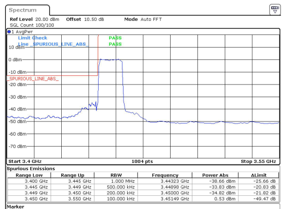
15MHz_30kHz_3457.5MHz_DFT-s-OFDM QPSK_RB36@0&-33.83 dBm
