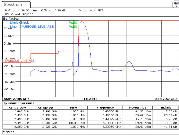
20MHz_15kHz_2510MHz_DFT-s-OFDM QPSK_RB1@0&28.49 dBm
