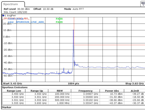
15MHz_30kHz_3542.5MHz_DFT-s-OFDM QPSK_RB1@37&-31.50 dBm
