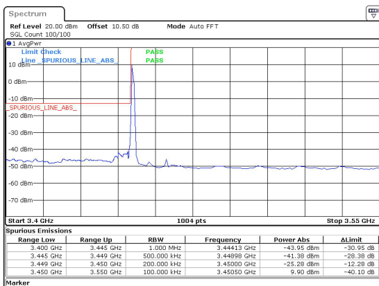
15MHz_30kHz_3457.5MHz_DFT-s-OFDM QPSK_RB1@0&-25.28 dBm
