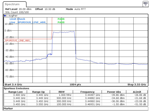
25MHz_30kHz_3462.5MHz_DFT-s-OFDM QPSK_RB64@0&-34.68 dBm
