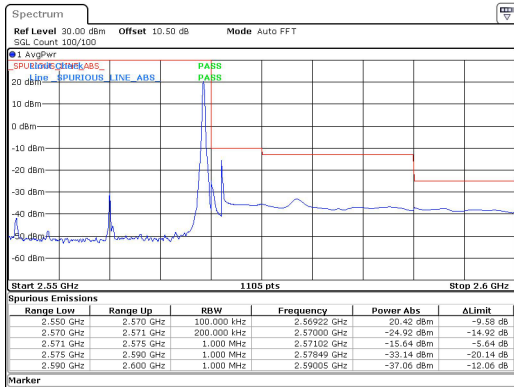
20MHz_15kHz_2560MHz_DFT-s-OFDM QPSK_RB1@105&-15.64 dBm
