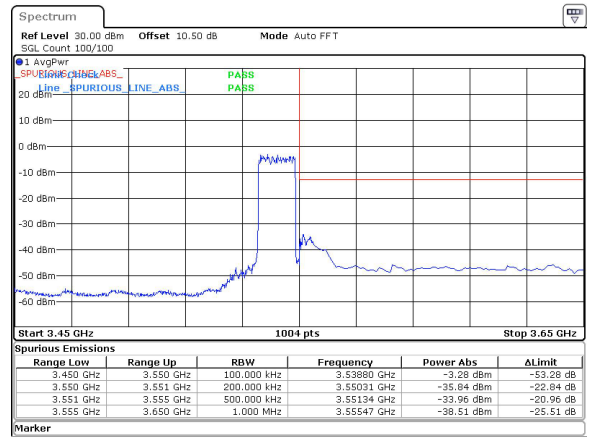
15MHz_30kHz_3542.5MHz_DFT-s-OFDM QPSK_RB36@0&-33.96 dBm
