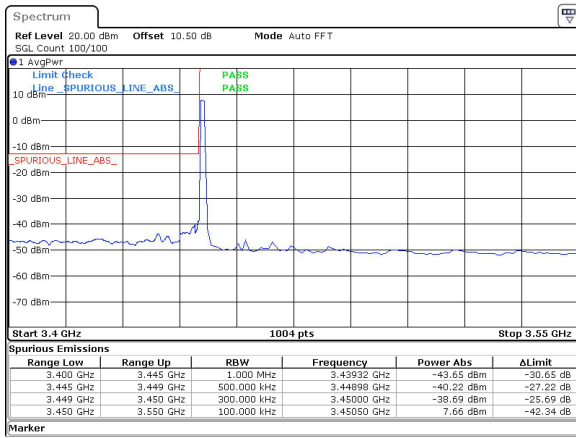
25MHz_30kHz_3462.5MHz_DFT-s-OFDM QPSK_RB1@0&-38.69 dBm
