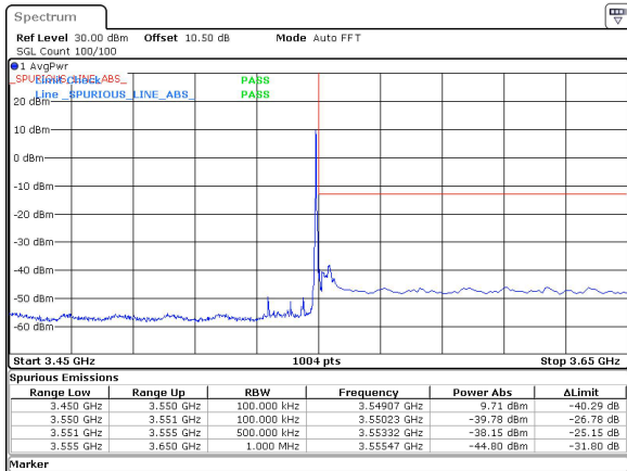
10MHz_30kHz_3545MHz_DFT-s-OFDM QPSK_RB1@23&-38.15 dBm
