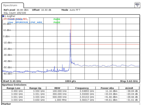
25MHz_30kHz_3537.5MHz_DFT-s-OFDM QPSK_RB1@64&-33.04 dBm
