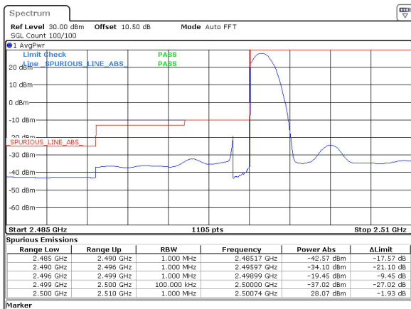
10MHz_15kHz_2505MHz_DFT-s-OFDM QPSK_RB1@0&28.07 dBm
