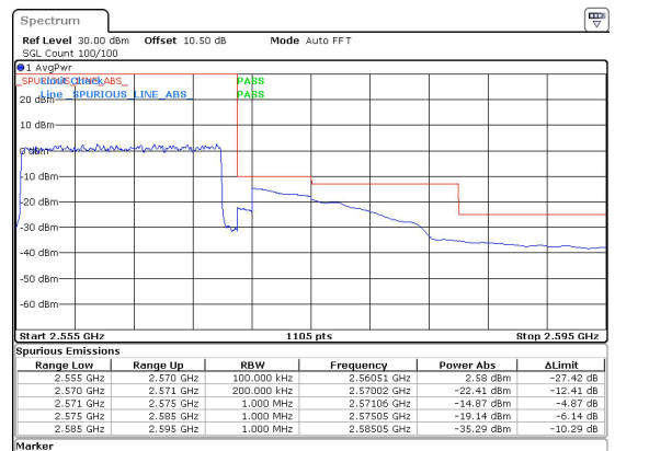
15MHz_15kHz_2562.5MHz_DFT-s-OFDM QPSK_RB75@0&-14.87 dBm
