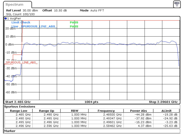
100MHz_30kHz_2546.01MHz_DFT-s-OFDM QPSK_RB270@0&-16.23 dBm
