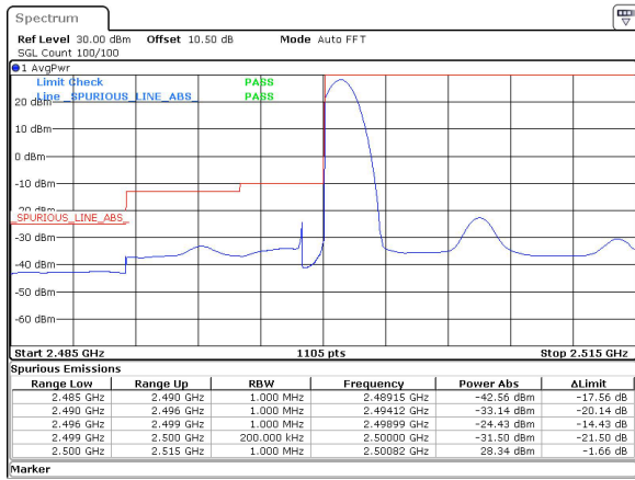
15MHz_15kHz_2507.5MHz_DFT-s-OFDM QPSK_RB1@0&28.34 dBm
