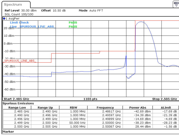
5MHz_15kHz_2502.5MHz_DFT-s-OFDM QPSK_RB1@0&28.44 dBm
