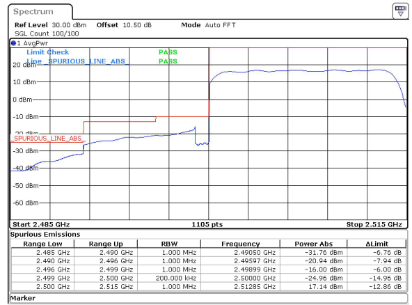
15MHz_15kHz_2507.5MHz_DFT-s-OFDM QPSK_RB75@0&-16.00 dBm
