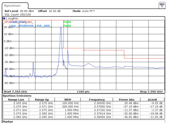
15MHz_15kHz_2562.5MHz_DFT-s-OFDM QPSK_RB1@78&-11.37 dBm
