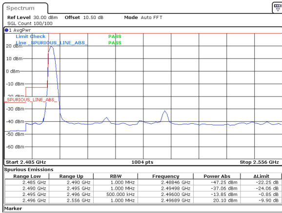
60MHz_30kHz_2526MHz_DFT-s-OFDM QPSK_RB1@0&-13.85 dBm
