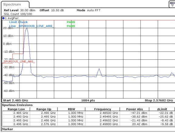
80MHz_30kHz_2536.02MHz_DFT-s-OFDM QPSK_RB1@0&-21.43 dBm
