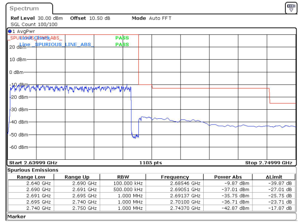
50MHz_30kHz_2664.99MHz_DFT-s-OFDM QPSK_RB128@0&-42.87 dBm
