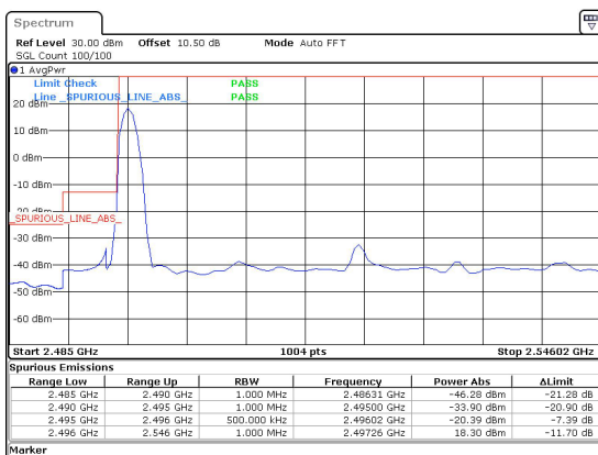
50MHz_30kHz_2521.02MHz_DFT-s-OFDM QPSK_RB1@0&-20.39 dBm
