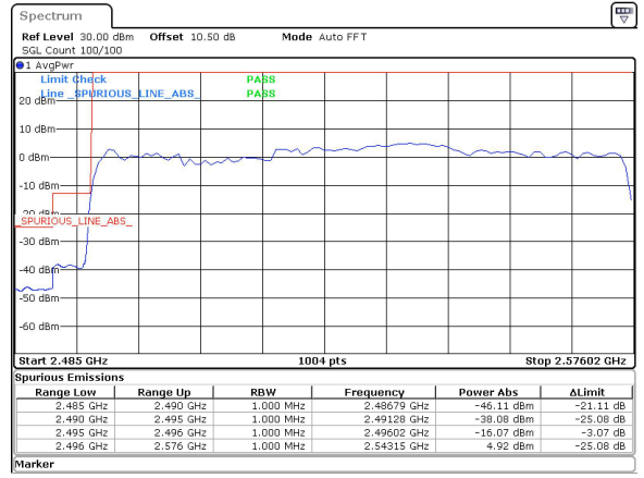
80MHz_30kHz_2536.02MHz_DFT-s-OFDM QPSK_RB216@0&-16.07 dBm
