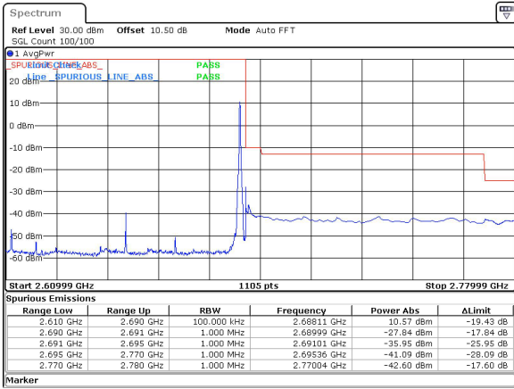
80MHz_30kHz_2649.99MHz_DFT-s-OFDM QPSK_RB1@216&-42.60 dBm
