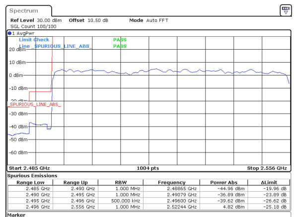
60MHz_30kHz_2526MHz_DFT-s-OFDM QPSK_RB162@0&-44.96 dBm
