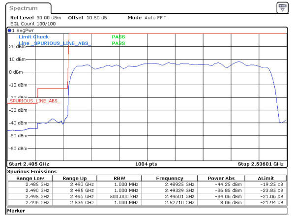
40MHz_30kHz_2516.01MHz_DFT-s-OFDM QPSK_RB100@0&-44.25 dBm
