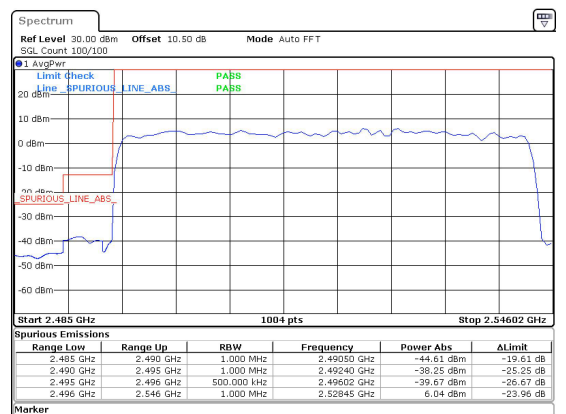
50MHz_30kHz_2521.02MHz_DFT-s-OFDM QPSK_RB128@0&-44.61 dBm
