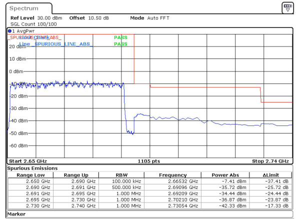
40MHz_30kHz_2670MHz_DFT-s-OFDM QPSK_RB100@0&-42.33 dBm
