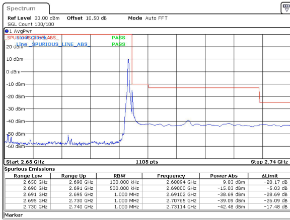
40MHz_30kHz_2670MHz_DFT-s-OFDM QPSK_RB1@105&-15.03 dBm
