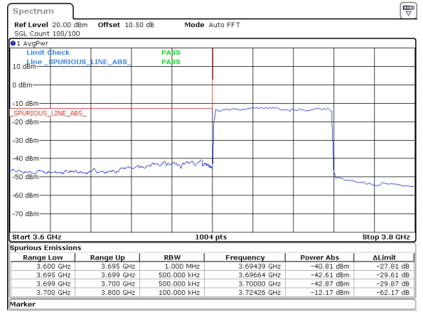
60MHz_30kHz_3730MHz_DFT-s-OFDM QPSK_RB162@0 -40.81 dBm
