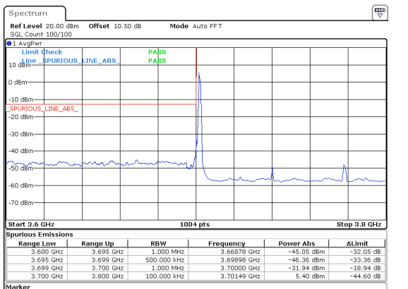
80MHz_30kHz_3740MHz_DFT-s-OFDM QPSK_RB1@0 -31.94 dBm
