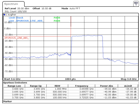
50MHz_30kHz_3725MHz_DFT-s-OFDM QPSK_RB128@0 -39.02 dBm
