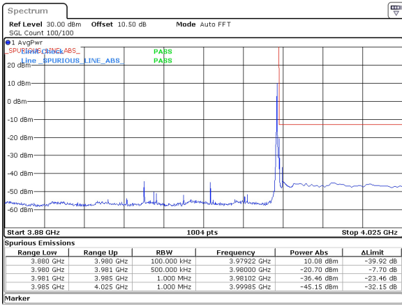
50MHz_15kHz_3955MHz_DFT-s-OFDM QPSK_RB1@269 -20.70 dBm
