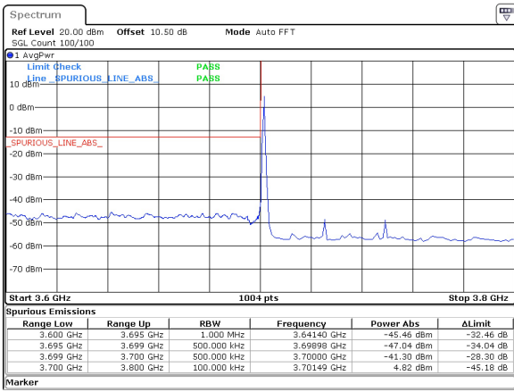
50MHz_30kHz_3725MHz_DFT-s-OFDM QPSK_RB1@0 -41.30 dBm
