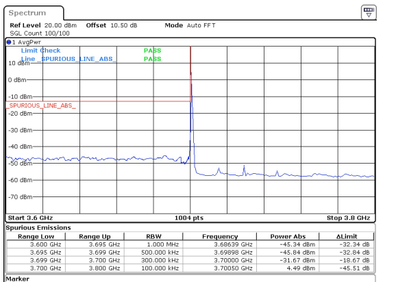
30MHz_15kHz_3715MHz_DFT-s-OFDM QPSK_RB1@0 -31.67 dBm
