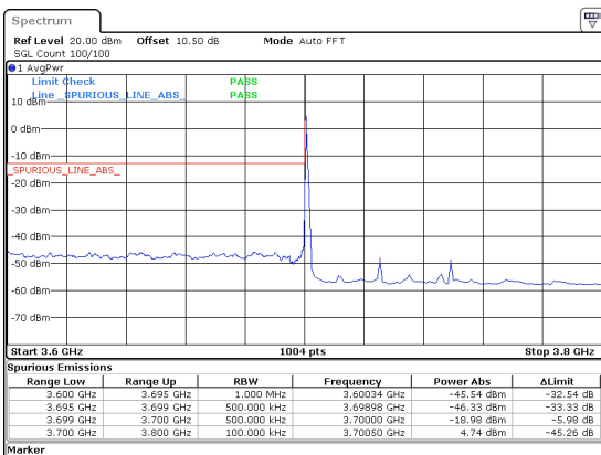
50MHz_15kHz_3725MHz_DFT-s-OFDM QPSK_RB1@0 -18.98 dBm
