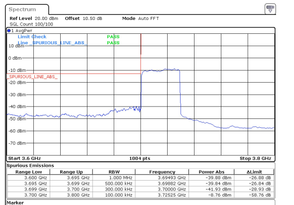
30MHz_15kHz_3715MHz_DFT-s-OFDM QPSK_RB160@0 -39.84 dBm
