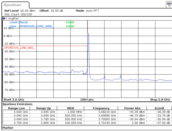
40MHz_15kHz_3720MHz_DFT-s-OFDM QPSK_RB1@0 -39.94 dBm
