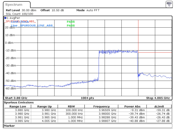
30MHz_15kHz_3965MHz_DFT-s-OFDM QPSK_RB160@0 -39.43 dBm
