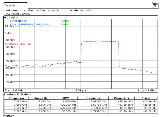
50MHz_15kHz_3725MHz_DFT-s-OFDM QPSK_RB270@0 -39.84 dBm
