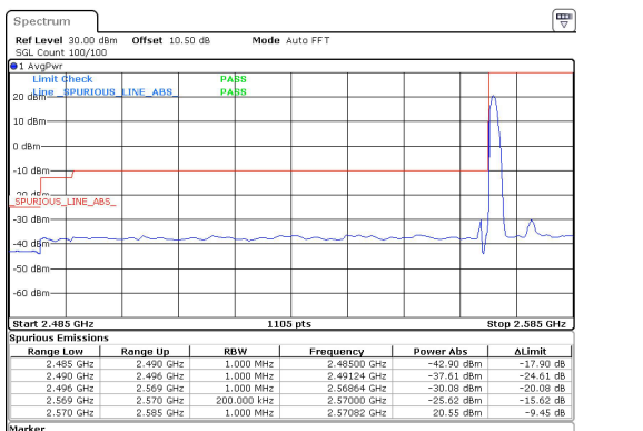
15MHz_30kHz_2577.5MHz_DFT-s-OFDM QPSK_RB1@0&20.55 dBm
