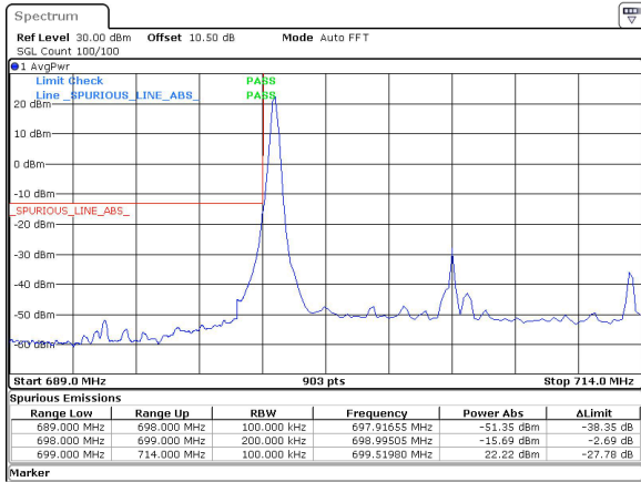
15MHz_15kHz_706.5MHz_DFT-s-OFDM QPSK_RB1@0&-15.69 dBm
