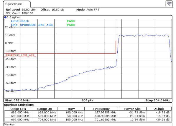
5MHz_15kHz_701.5MHz_DFT-s-OFDM QPSK_RB25@0&-28.34 dBm
