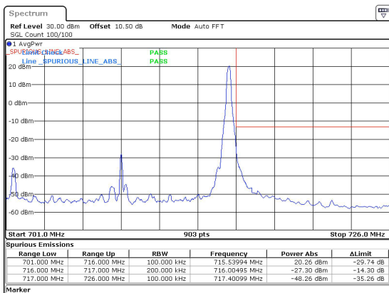
15MHz_15kHz_708.5MHz_DFT-s-OFDM QPSK_RB1@78&-27.30 dBm
