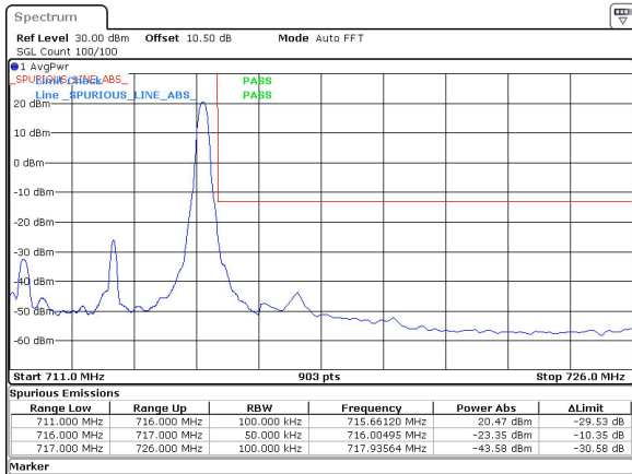
5MHz_15kHz_713.5MHz_DFT-s-OFDM QPSK_RB1@24&-23.35 dBm
