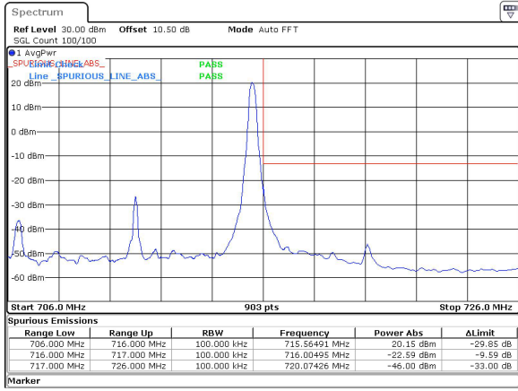
10MHz_15kHz_711MHz_DFT-s-OFDM QPSK_RB1@51&-22.59 dBm
