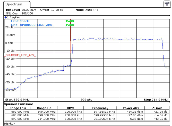
15MHz_15kHz_706.5MHz_DFT-s-OFDM QPSK_RB75@0&-27.06 dBm
