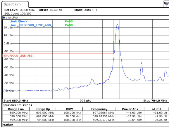
5MHz_15kHz_701.5MHz_DFT-s-OFDM QPSK_RB1@0&-17.96 dBm
