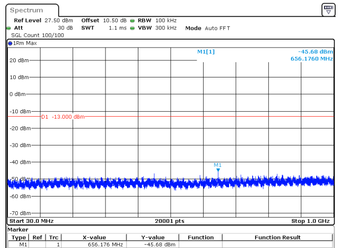
20MHz_15kHz_1720MHz_DFT-s-OFDM QPSK_RB100@0 -45.68 dBm
