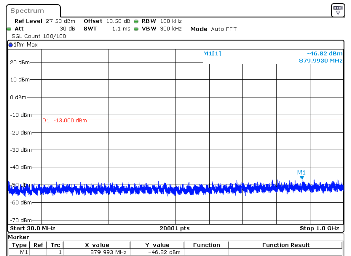
25MHz_15kHz_1722.5MHz_DFT-s-OFDM QPSK_RB128@0 -46.82 dBm
