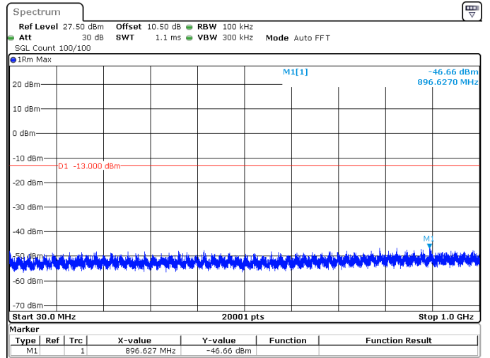
30MHz_15kHz_1745MHz_DFT-s-OFDM QPSK_RB1@0 -46.66 dBm
