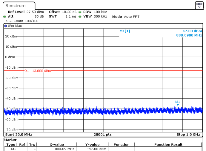
40MHz_15kHz_1730MHz_DFT-s-OFDM QPSK_RB216@0 -47.08 dBm
