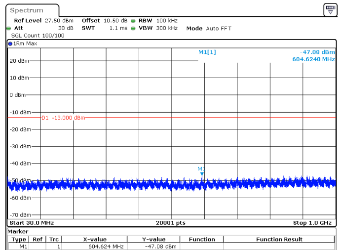
30MHz_15kHz_1725MHz_DFT-s-OFDM QPSK_RB160@0 -47.08 dBm
