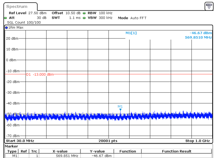
20MHz_15kHz_1745MHz_DFT-s-OFDM QPSK_RB100@0 -46.67 dBm
