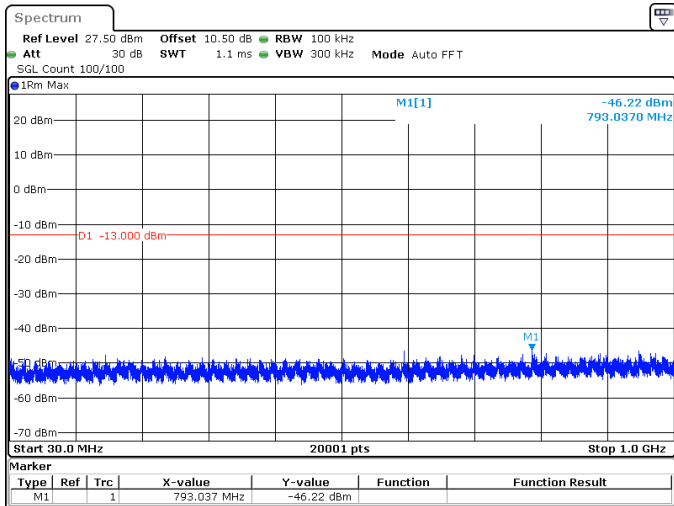
40MHz_15kHz_1730MHz_DFT-s-OFDM QPSK_RB1@215 -46.22 dBm
