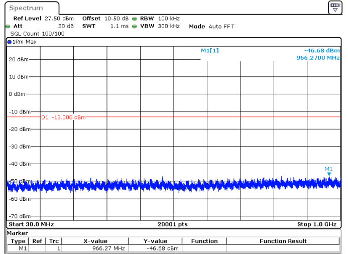
30MHz_15kHz_1745MHz_DFT-s-OFDM QPSK_RB1@159 -46.68 dBm
