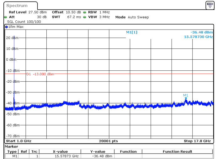
30MHz_15kHz_1725MHz_DFT-s-OFDM QPSK_RB1@159 -36.48 dBm
