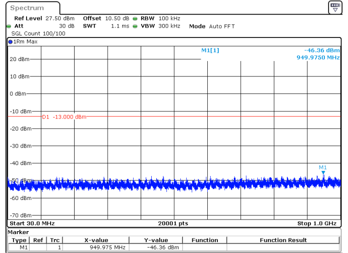
25MHz_15kHz_1745MHz_DFT-s-OFDM QPSK_RB1@132 -46.36 dBm
