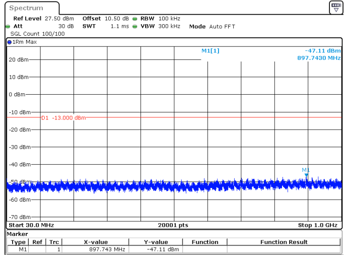
40MHz_15kHz_1745MHz_DFT-s-OFDM QPSK_RB1@215 -47.11 dBm
