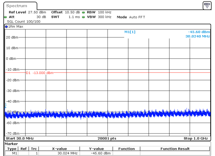
25MHz_15kHz_1745MHz_DFT-s-OFDM QPSK_RB128@0 -45.60 dBm
