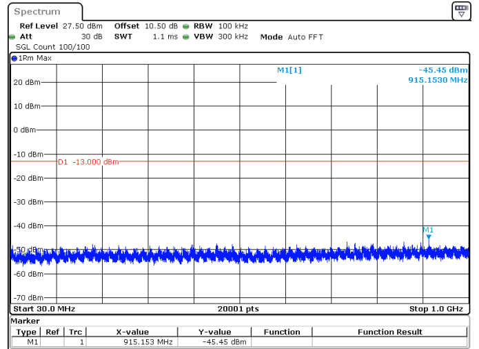
25MHz_15kHz_1745MHz_DFT-s-OFDM QPSK_RB1@0 -45.45 dBm
