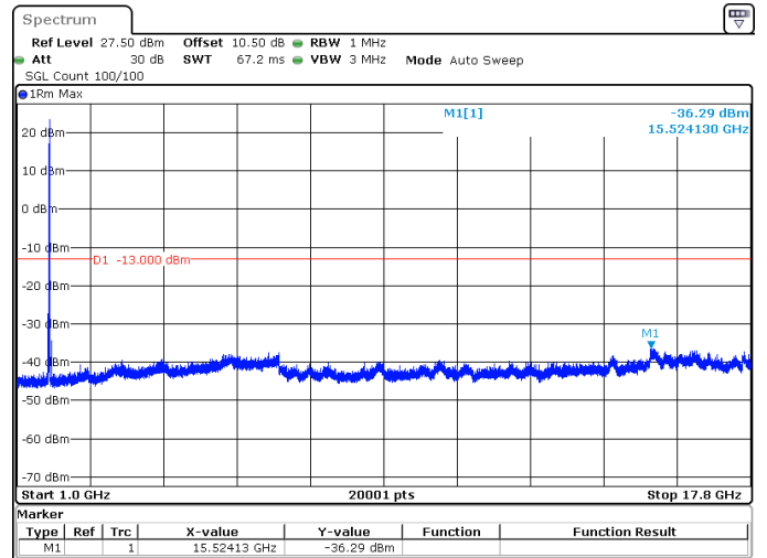
25MHz_15kHz_1722.5MHz_DFT-s-OFDM QPSK_RB1@132 -36.29 dBm
