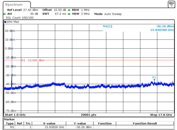
25MHz_15kHz_1767.5MHz_DFT-s-OFDM QPSK_RB1@132 -36.26 dBm
