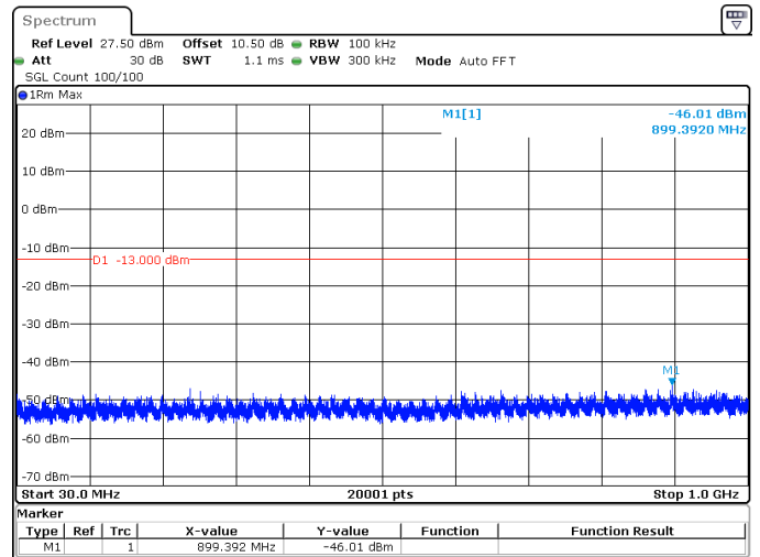
25MHz_15kHz_1767.5MHz_DFT-s-OFDM QPSK_RB128@0 -46.01 dBm
