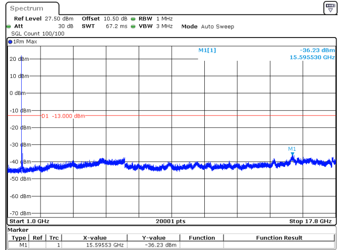
30MHz_15kHz_1725MHz_DFT-s-OFDM QPSK_RB1@0 -36.23 dBm
