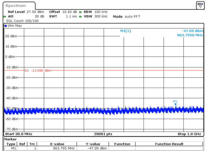
30MHz_15kHz_1745MHz_DFT-s-OFDM QPSK_RB160@0 -47.09 dBm
