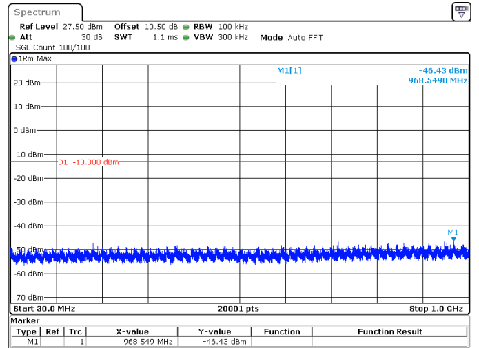
20MHz_15kHz_1745MHz_DFT-s-OFDM QPSK_RB1@105 -46.43 dBm
