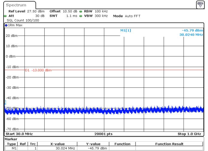
40MHz_15kHz_1760MHz_DFT-s-OFDM QPSK_RB216@0 -45.79 dBm
