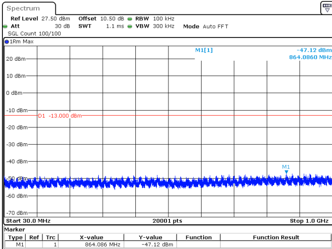
40MHz_15kHz_1745MHz_DFT-s-OFDM QPSK_RB216@0 -47.12 dBm
