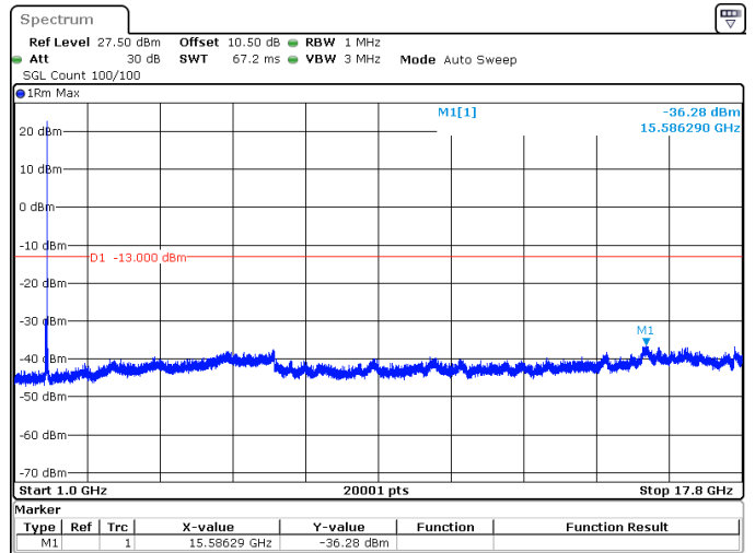
40MHz_15kHz_1730MHz_DFT-s-OFDM QPSK_RB1@215 -36.28 dBm
