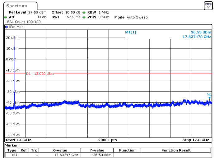
25MHz_15kHz_1767.5MHz_DFT-s-OFDM QPSK_RB1@0 -36.53 dBm
