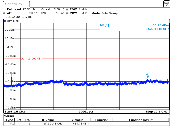
40MHz_15kHz_1760MHz_DFT-s-OFDM QPSK_RB1@0 -35.73 dBm
