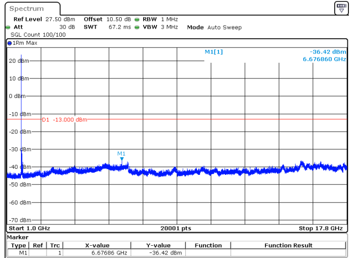
40MHz_15kHz_1730MHz_DFT-s-OFDM QPSK_RB1@0 -36.42 dBm
