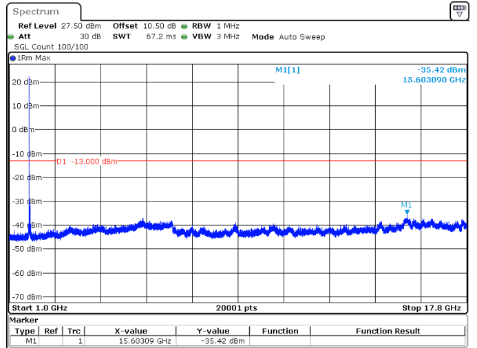
40MHz_15kHz_1745MHz_DFT-s-OFDM QPSK_RB1@0 -35.42 dBm
