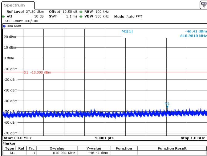
40MHz_15kHz_1745MHz_DFT-s-OFDM QPSK_RB1@0 -46.41 dBm
