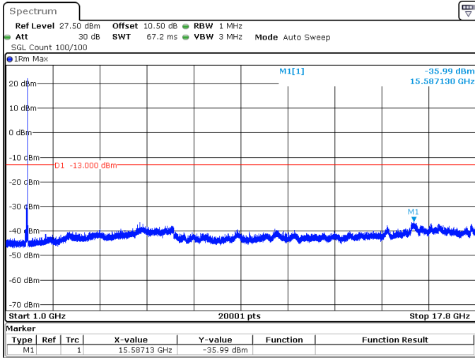
40MHz_15kHz_1745MHz_DFT-s-OFDM QPSK_RB1@215 -35.99 dBm
