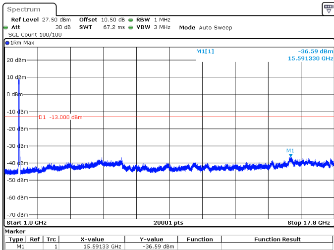
40MHz_15kHz_1730MHz_DFT-s-OFDM QPSK_RB216@0 -36.59 dBm
