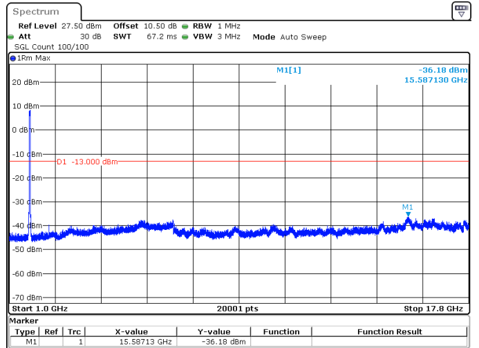
40MHz_15kHz_1745MHz_DFT-s-OFDM QPSK_RB216@0 -36.18 dBm
