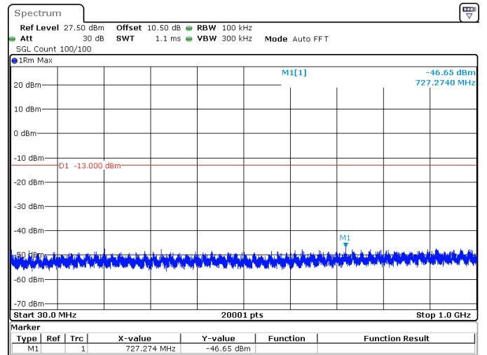
30MHz_15kHz_1765MHz_DFT-s-OFDM QPSK_RB160@0 -46.65 dBm
