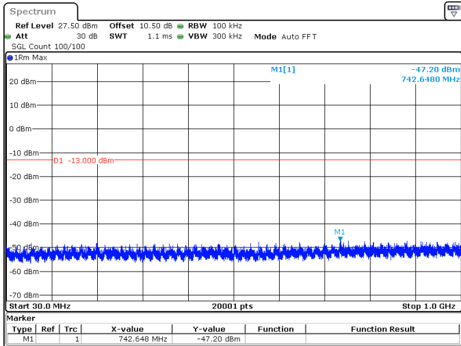
40MHz_15kHz_1730MHz_DFT-s-OFDM QPSK_RB1@0 -47.20 dBm
