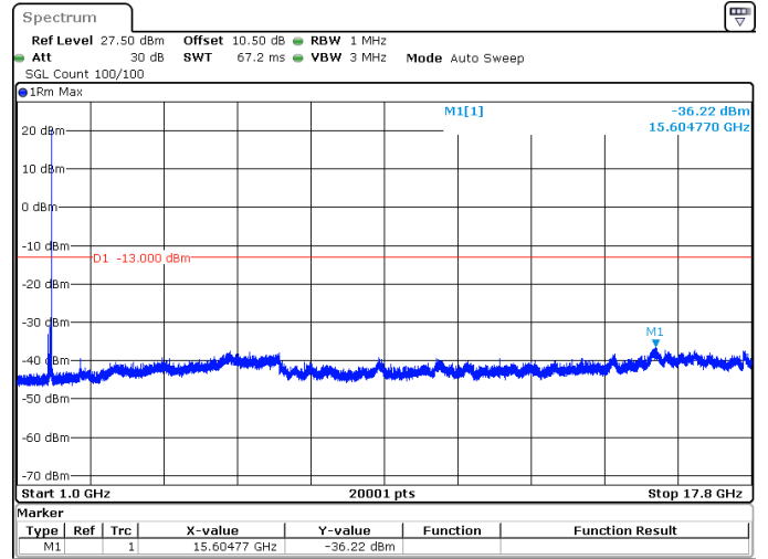
40MHz_15kHz_1760MHz_DFT-s-OFDM QPSK_RB1@215 -36.22 dBm
