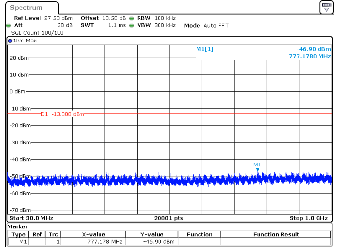
30MHz_15kHz_1765MHz_DFT-s-OFDM QPSK_RB1@159 -46.90 dBm
