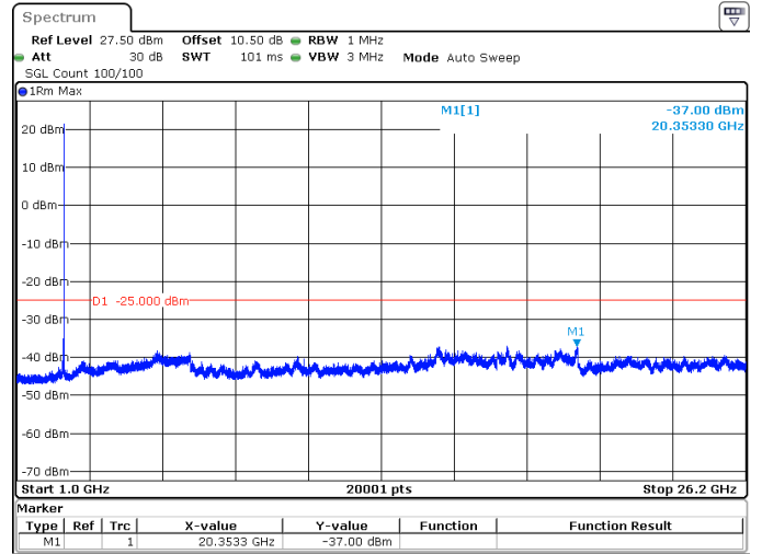
40MHz_30kHz_2600MHz_DFT-s-OFDM QPSK_RB1@105 -37.00 dBm
