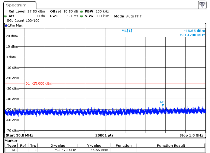
40MHz_30kHz_2600MHz_DFT-s-OFDM QPSK_RB1@0 -46.65 dBm
