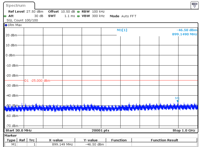
40MHz_30kHz_2600MHz_DFT-s-OFDM QPSK_RB100@0 -46.50 dBm
