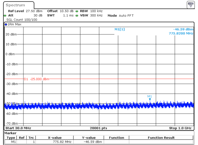
25MHz_30kHz_2607.5MHz_DFT-s-OFDM QPSK_RB1@64 -46.59 dBm
