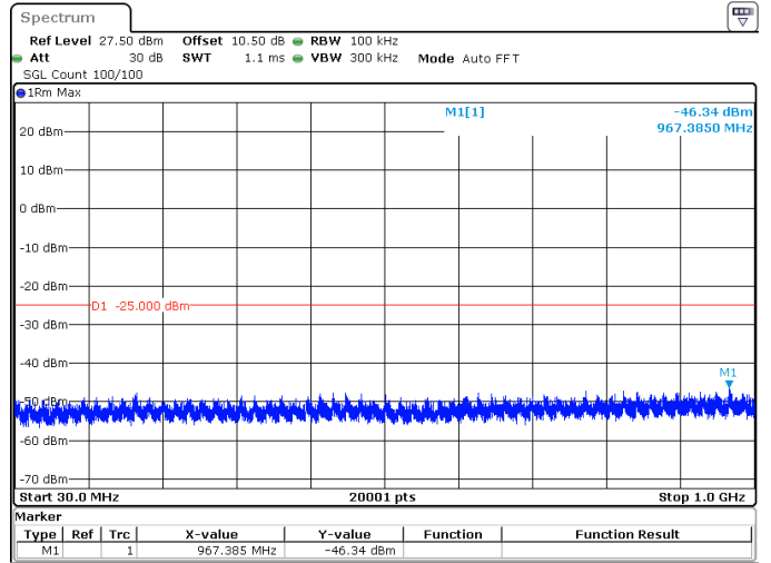
30MHz_30kHz_2605MHz_DFT-s-OFDM QPSK_RB1@77 -46.34 dBm
