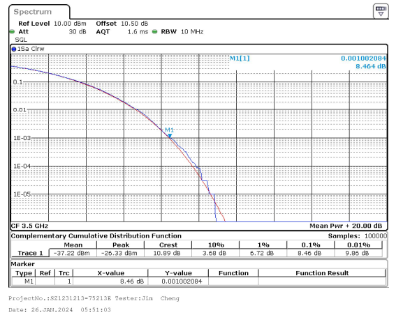
10MHz_30kHz_3500MHz_DFT-s-OFDM 256 QAM_RB24@0 8.46 dB
