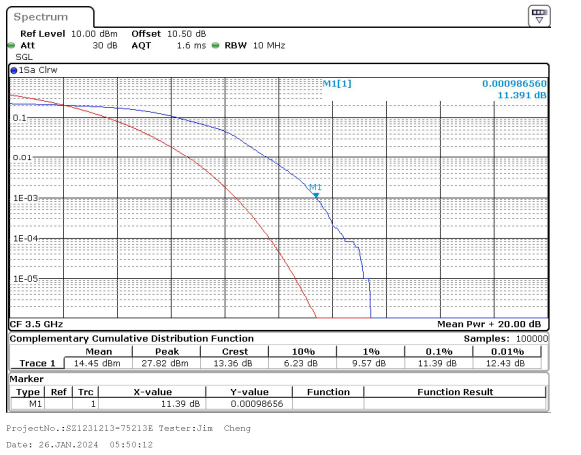
10MHz_30kHz_3500MHz_DFT-s-OFDM 16 QAM_RB24@0 11.39 dB
