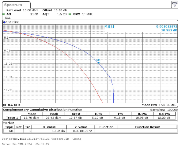
10MHz_30kHz_3500MHz_CP-OFDM 64 QAM_RB24@0 10.96 dB
