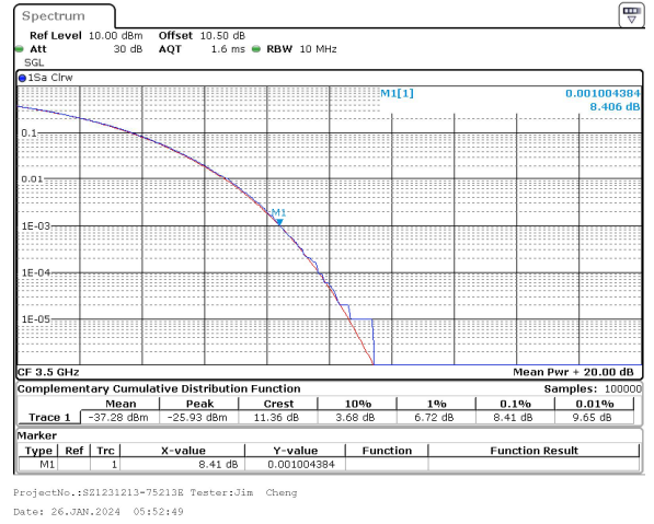
10MHz_30kHz_3500MHz_CP-OFDM 256 QAM_RB24@0 8.41 dB
