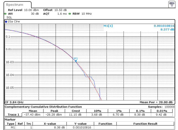
10MHz_15kHz_3840MHz_CP-OFDM QPSK_RB52@0 8.38 dB
