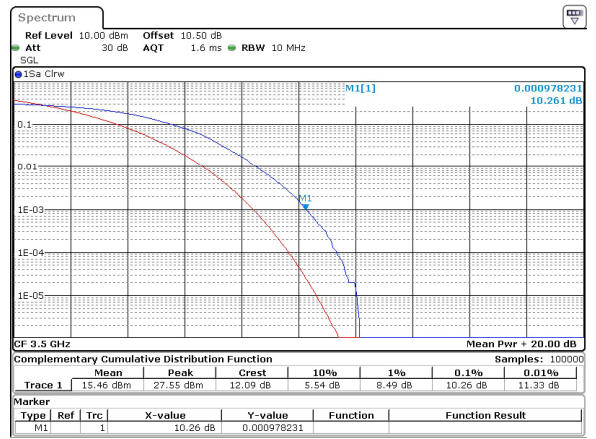
10MHz_30kHz_3500MHz_DFT-s-OFDM 64 QAM_RB24@0 10.26 dB
