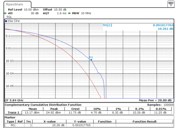
10MHz_15kHz_3840MHz_CP-OFDM 256 QAM_RB52@0 10.26 dB
