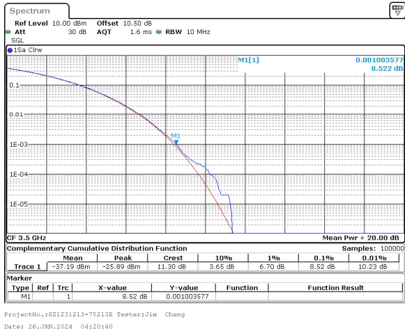
10MHz_15kHz_3500MHz_CP-OFDM 64 QAM_RB52@0 8.52 dB
