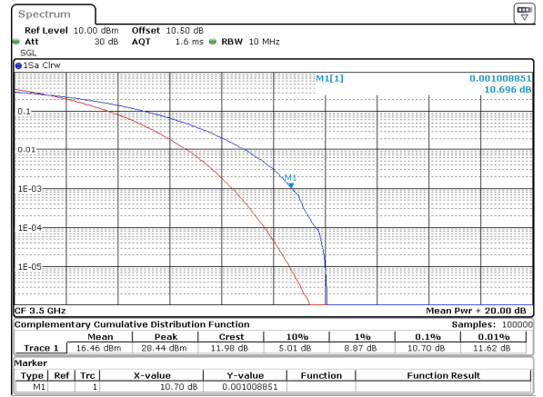
10MHz_30kHz_3500MHz_CP-OFDM 16 QAM_RB24@0 10.70 dB
