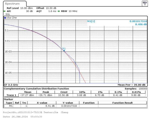
10MHz_15kHz_3500MHz_CP-OFDM 256 QAM_RB52@0 8.41 dB
