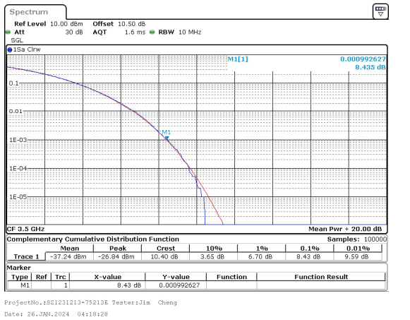
10MHz_15kHz_3500MHz_DFT-s-OFDM 16 QAM_RB50@0 8.43 dB
