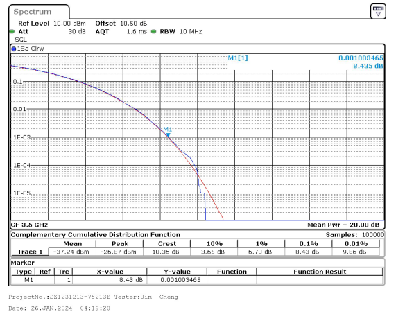
10MHz_15kHz_3500MHz_DFT-s-OFDM 256 QAM_RB50@0 8.43 dB
