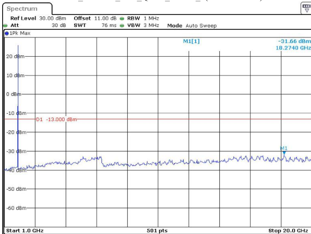
Band 2_1.4 MHz_Low_QPSK_RB6#0_2(1GHz-20GHz)
