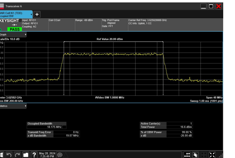
20MHz_30kHz_3625MHz_CP-OFDM 64QAM_RB51@0
