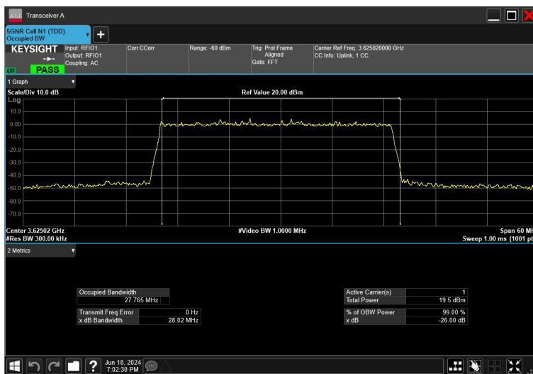
30MHz_30kHz_3625MHz_DFT-s-OFDM 16QAM_RB75@0
