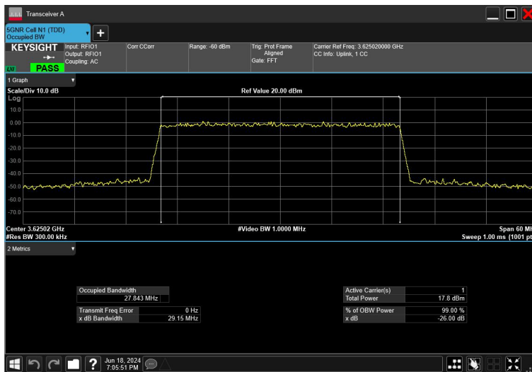
30MHz_30kHz_3625MHz_CP-OFDM 64QAM_RB78@0
