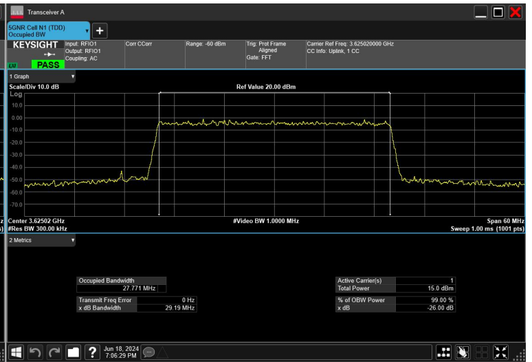
30MHz_30kHz_3625MHz_CP-OFDM 256QAM_RB78@0
