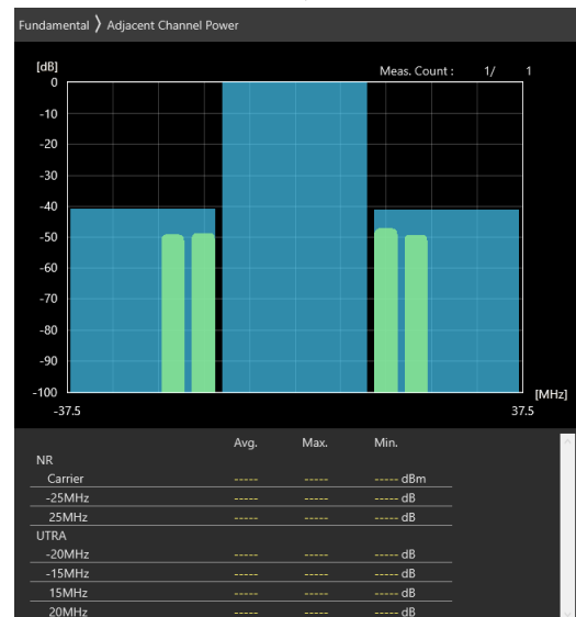
25MHz_15kHz_3687.5MHz_DFT-s-OFDM 16 QAM_RB1@132 -40.87 dB,-41.17 dB
