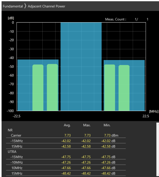
15MHz_30kHz_3692.5MHz_CP-OFDM QPSK_RB38@0 -42.02 dB,-42.58 dB
