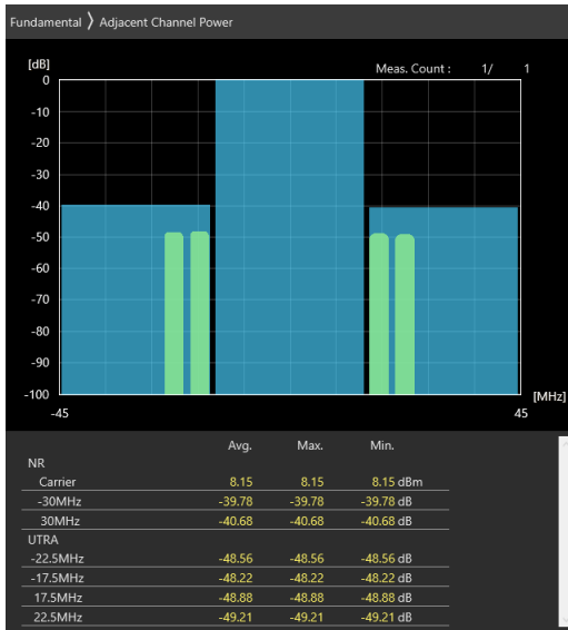
30MHz_30kHz_3565MHz_DFT-s-OFDM 64 QAM_RB75@0 -39.78 dB,-40.68 dB
