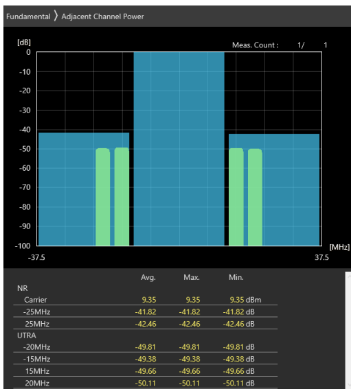
25MHz_30kHz_3562.5MHz_CP-OFDM QPSK_RB33@16 -41.82 dB,-42.46 dB
