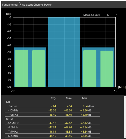
10MHz_30kHz_3695MHz_CP-OFDM QPSK_RB1@23 -43.36 dB,-43.4 dB
