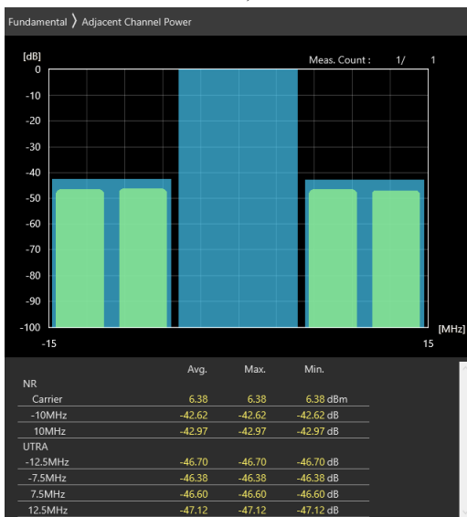
10MHz_30kHz_3555MHz_DFT-s-OFDM 256 QAM_RB24@0 -42.62 dB,-42.97 dB
