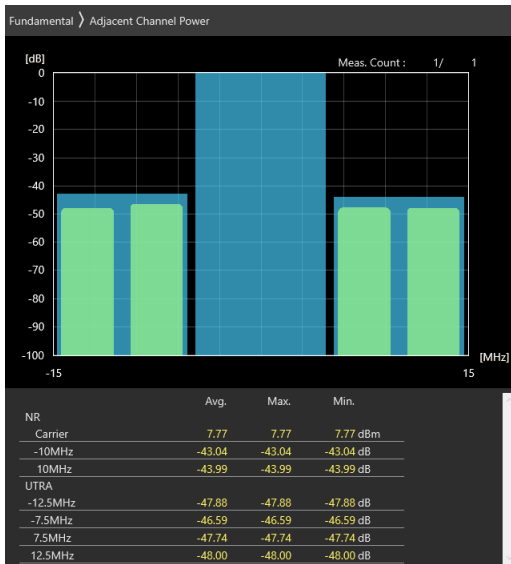
10MHz_30kHz_3555MHz_CP-OFDM 16 QAM_RB1@0 -43.04 dB,-43.99 dB
