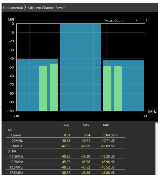
20MHz_15kHz_3560MHz_CP-OFDM 16 QAM_RB1@0 -40.71 dB,-42.09 dB
