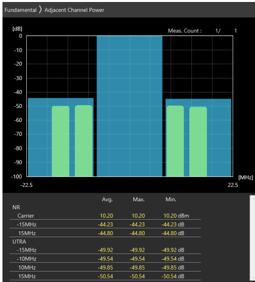
15MHz_15kHz_3692.5MHz_DFT-s-OFDM 16 QAM_RB36@18 -44.23 dB,-44.8 dB
