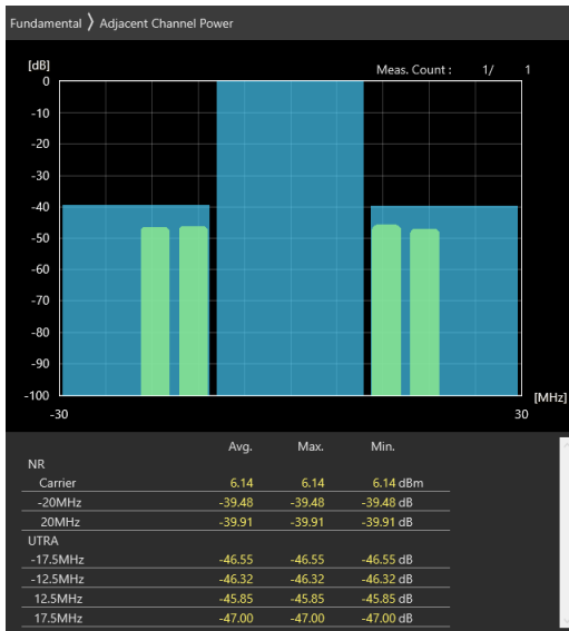
20MHz_30kHz_3690MHz_DFT-s-OFDM 256 QAM_RB1@50 -39.5 dB,-39.9 dB
