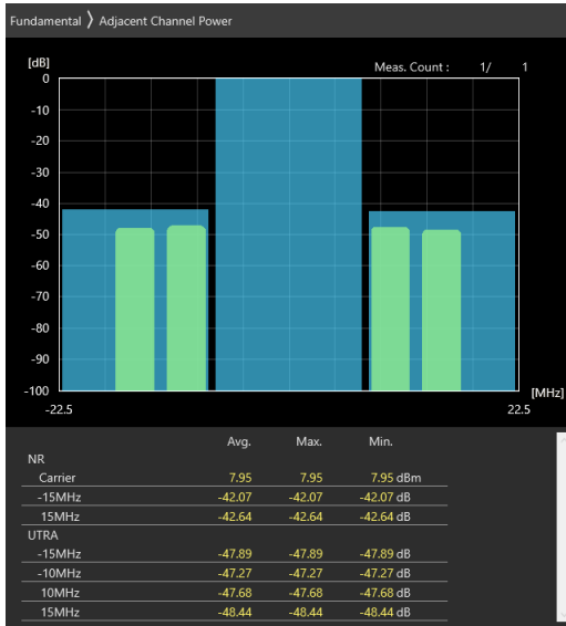
15MHz_30kHz_3692.5MHz_CP-OFDM QPSK_RB38@0 -42.07 dB,-42.64 dB
