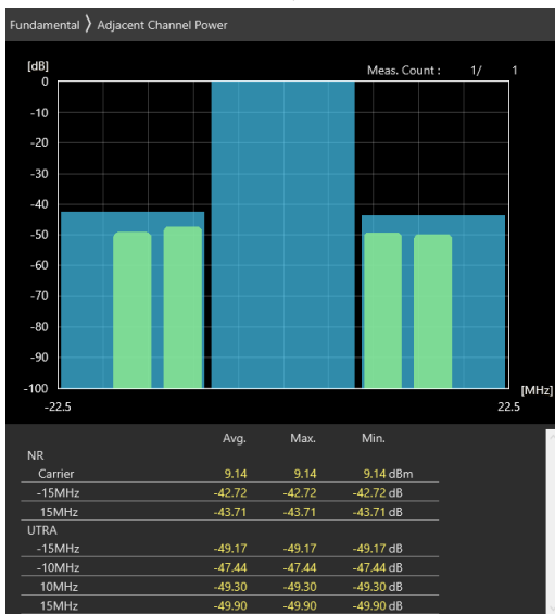
15MHz_30kHz_3557.5MHz_DFT-s-OFDM 16 QAM_RB1@0 -42.72 dB,-43.71 dB
