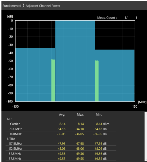
100MHz_30kHz_3600MHz_DFT-s-OFDM 64 QAM_RB270@ -34.18 dB,-36.05 dB
