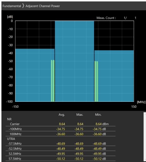
100MHz_30kHz_3600MHz_DFT-s-OFDM 16 QAM_RB270@0 -34.75 dB,-36.6 dB
