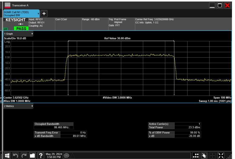
90MHz_30kHz_3625MHz_DFT-s-OFDM64QAM_RB243@0
