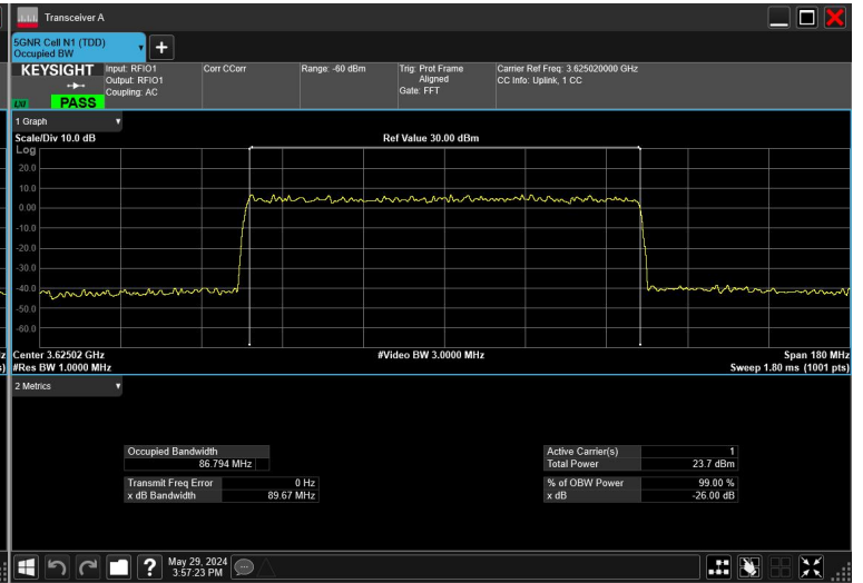
90MHz_30kHz_3625MHz_DFT-s-OFDM16QAM_RB243@0
