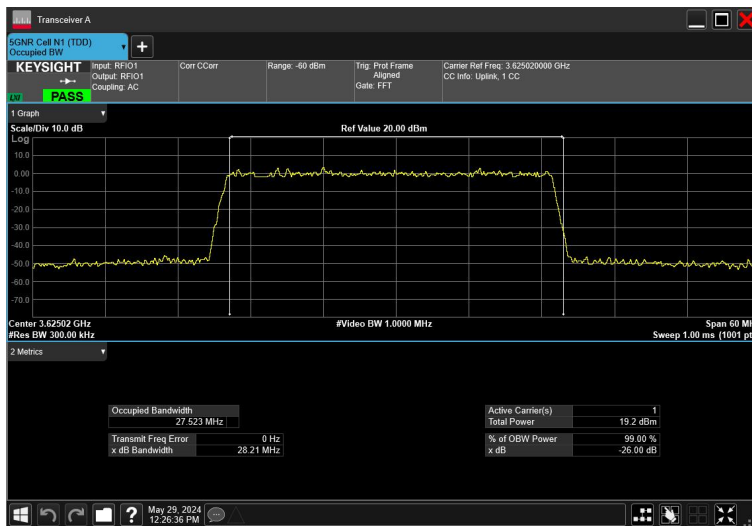
30MHz_30kHz_3625MHz_DFT-s-OFDM 256QAM_RB75@0
