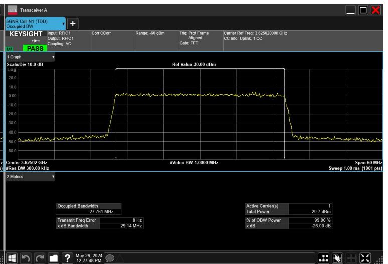
30MHz_30kHz_3625MHz_CP-OFDM 16QAM_RB78@0
