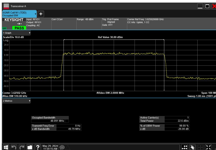
50MHz_15kHz_3625MHz_DFT-s-OFDM16QAM_RB270@0
