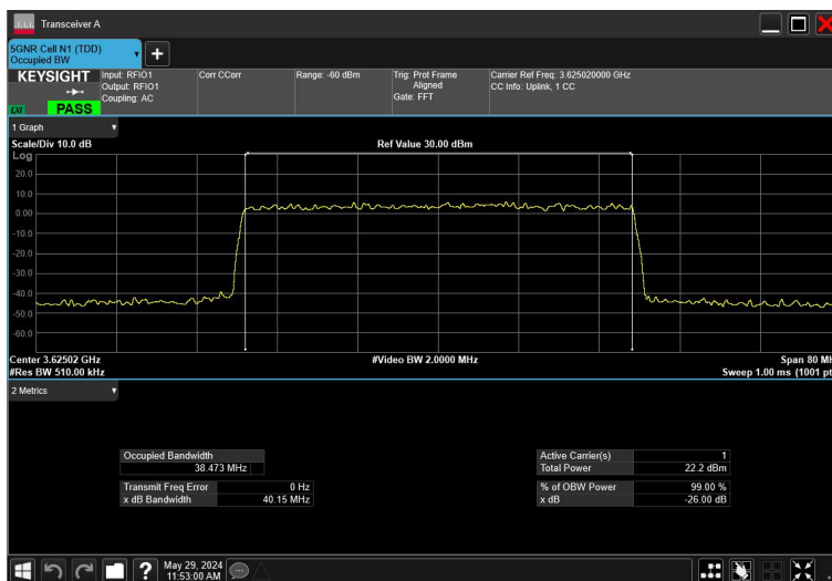
40MHz_15kHz_3625MHz_DFT-s-OFDM16QAM_RB216@0
