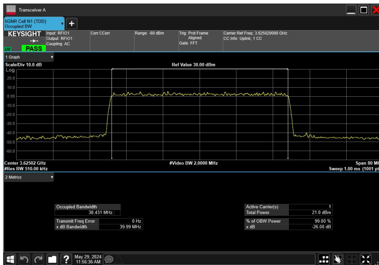
40MHz_15kHz_3625MHz_CP-OFDM64QAM_RB216@0
