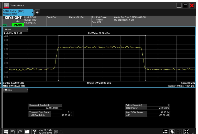
40MHz_30kHz_3625MHz_DFT-s-OFDM π/2 BPSK_RB100@0
