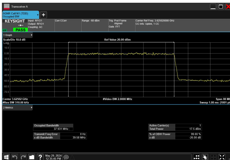
40MHz_30kHz_3625MHz_CP-OFDM 256QAM_RB106@0
