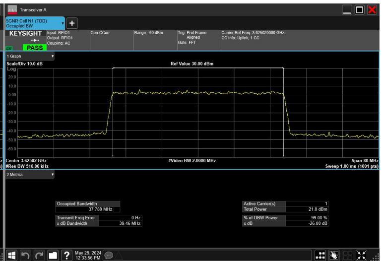
40MHz_30kHz_3625MHz_CP-OFDM 16QAM_RB106@0
