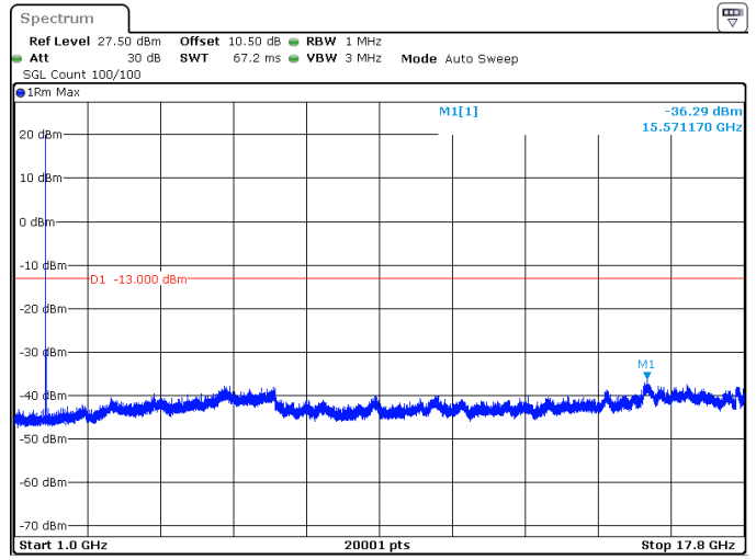
5MHz_15kHz_1712.5MHz_DFT-s-OFDM QPSK_RB1@0 -36.29 dBm
