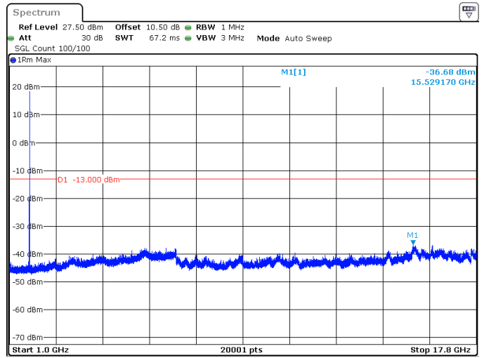
5MHz_15kHz_1712.5MHz_DFT-s-OFDM QPSK_RB1@24 -36.68 dBm
