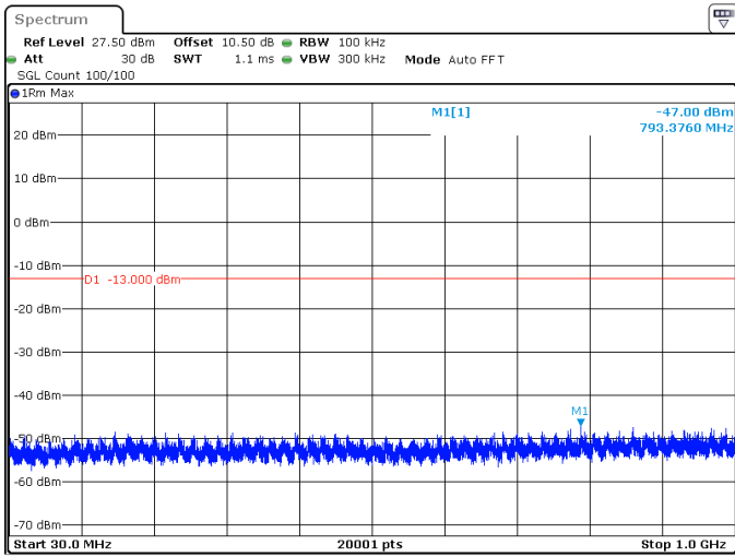
5MHz_15kHz_1712.5MHz_DFT-s-OFDM QPSK_RB1@24 -47.00 dBm
