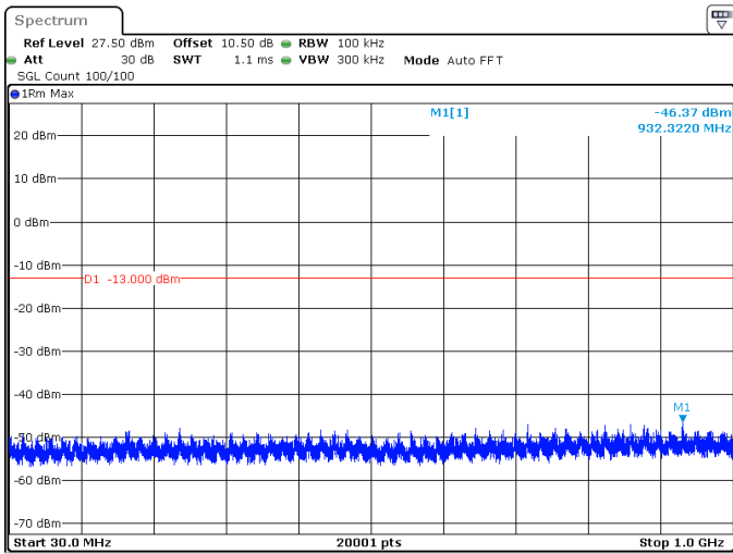
5MHz_15kHz_1712.5MHz_DFT-s-OFDM QPSK_RB25@0 -46.37 dBm
