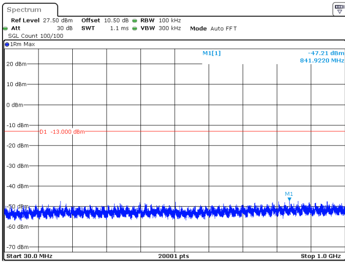
5MHz_15kHz_1712.5MHz_DFT-s-OFDM QPSK_RB1@0 -47.21 dBm
