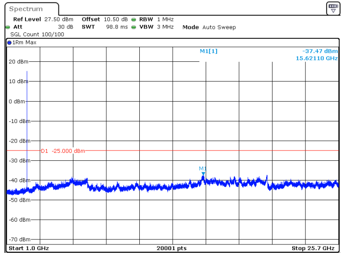
5MHz_15kHz_2502.5MHz_DFT-s-OFDM QPSK_RB1@24 -37.47 dBm
