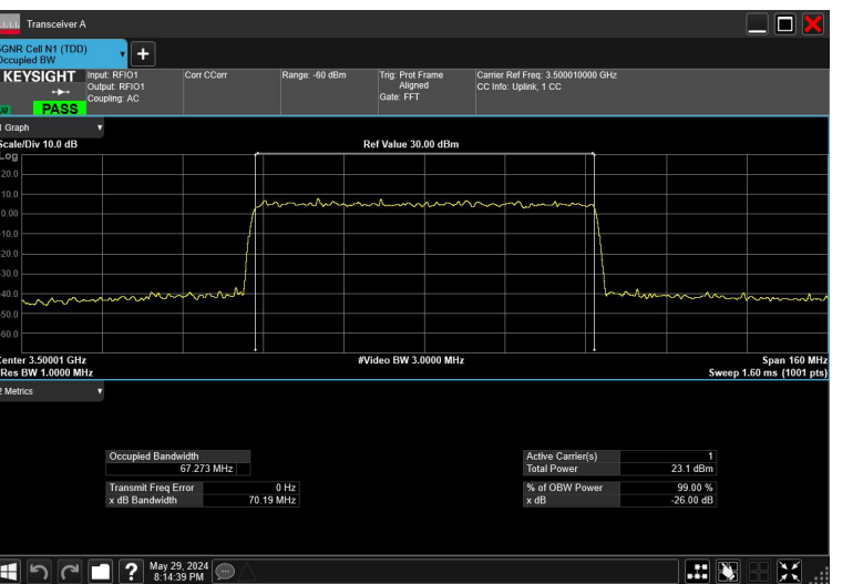
70MHz_30kHz_3500MHz_CP-OFDM 64QAM_RB189@0
