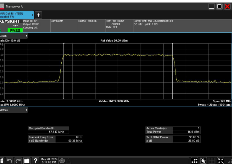
60MHz_30kHz_3500MHz_DFT-s-OFDM256QAM_RB162@0
