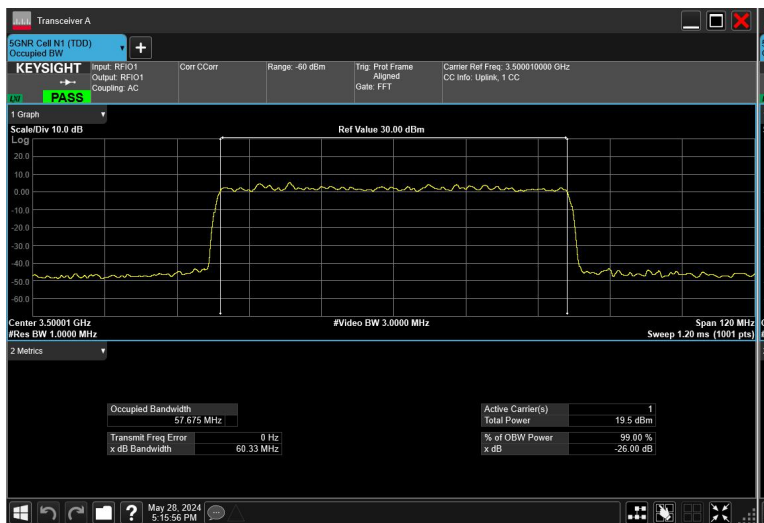
60MHz_30kHz_3500MHz_DFT-s-OFDM16QAM_RB162@0
