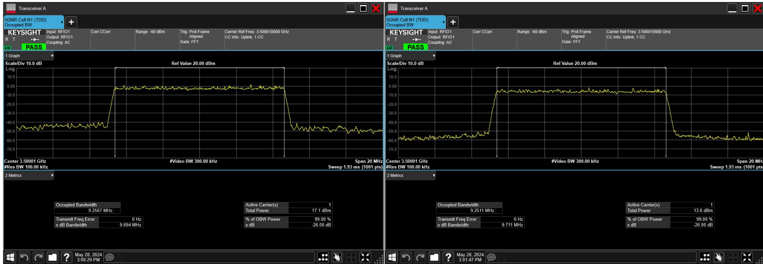
10MHz_15kHz_3500MHz_CP-OFDM16QAM_RB52@0
