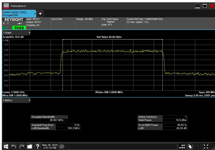
100MHz_30kHz_3500MHz_CP-OFDM 256QAM_RB273@0
