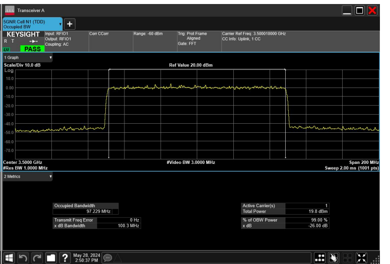
100MHz_30kHz_3500MHz_CP-OFDM 64QAM_RB273@0
