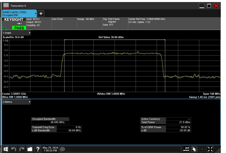
70MHz_30kHz_3500MHz_DFT-s-OFDM256QAM_RB180@0
