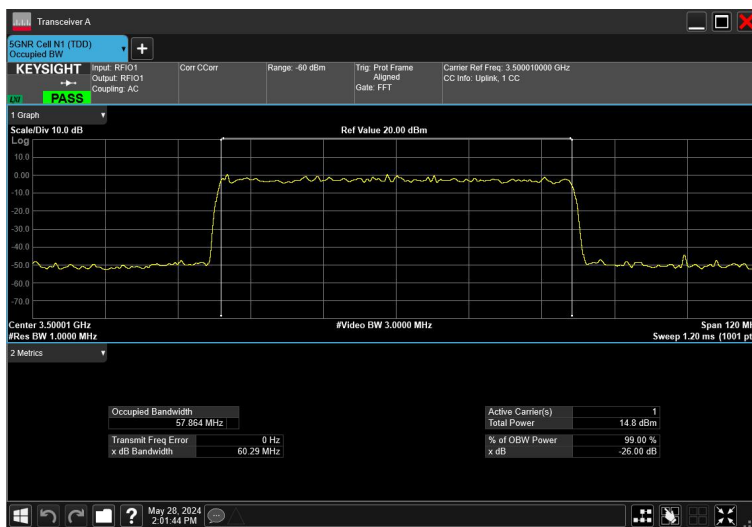
60MHz_30kHz_3500MHz_CP-OFDM 256QAM_RB162@0
