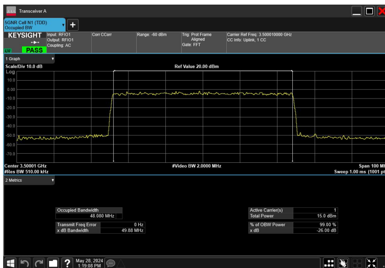
50MHz_15kHz_3500MHz_CP-OFDM 256QAM_RB270@0
