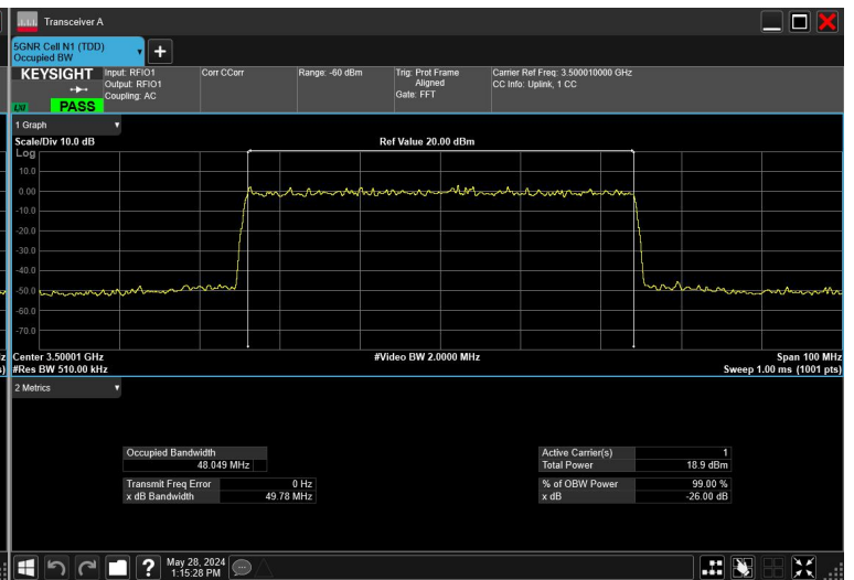
50MHz_15kHz_3500MHz_DFT-s-OFDM64QAM_RB270@0
