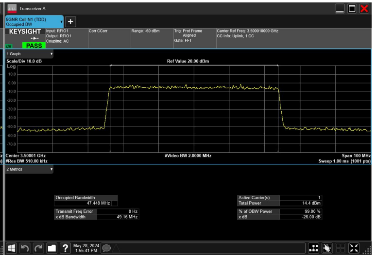
50MHz_30kHz_3500MHz_CP-OFDM256QAM_RB133@0
