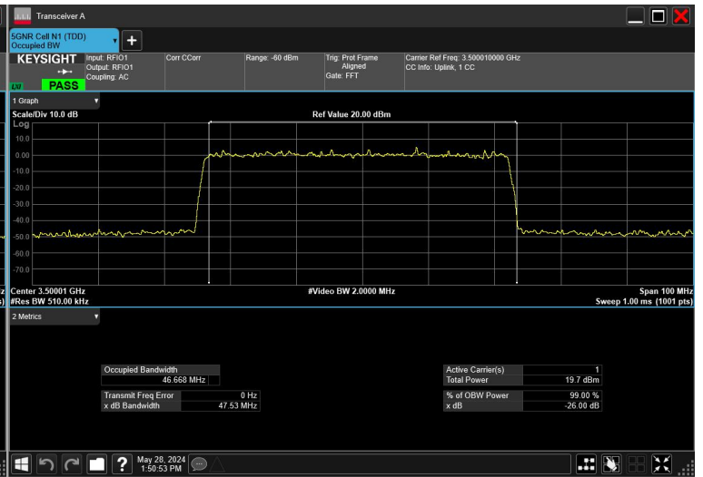
50MHz_30kHz_3500MHz_DFT-s-OFDM QPSK_RB128@0
