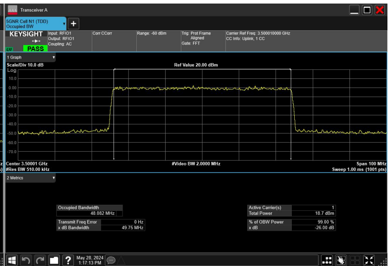
50MHz_15kHz_3500MHz_CP-OFDM 16QAM_RB270@0
