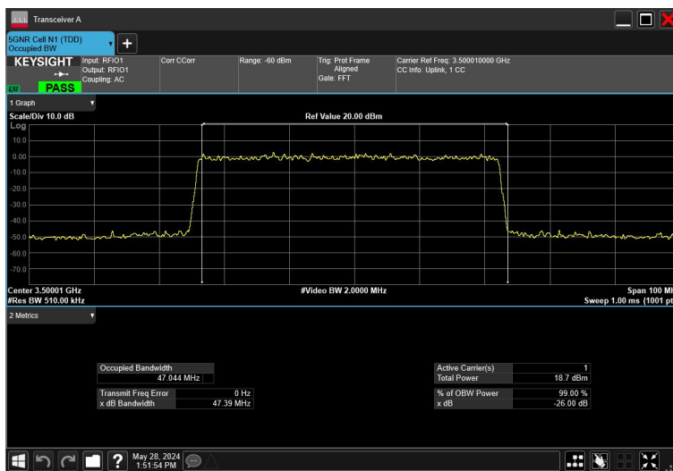
50MHz_30kHz_3500MHz_DFT-s-OFDM16QAM_RB128@0
