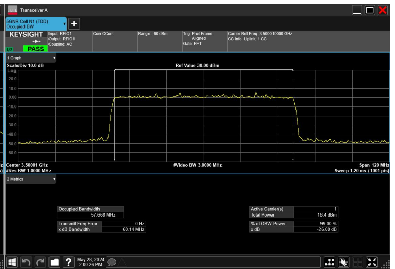
60MHz_30kHz_3500MHz_CP-OFDM 16QAM_RB162@0
