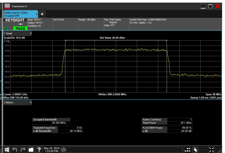
40MHz_15kHz_3500MHz_DFT-s-OFDM π/2 BPSK_RB216@0
