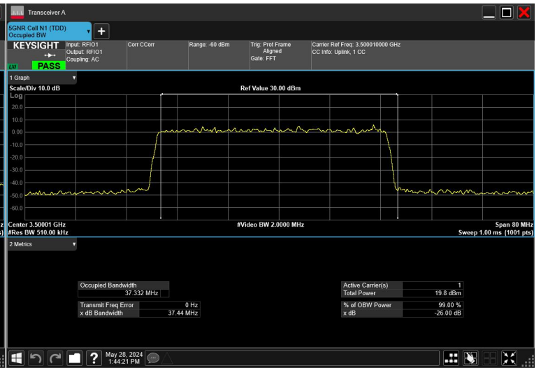
40MHz_30kHz_3500MHz_DFT-s-OFDM QPSK_RB100@0
