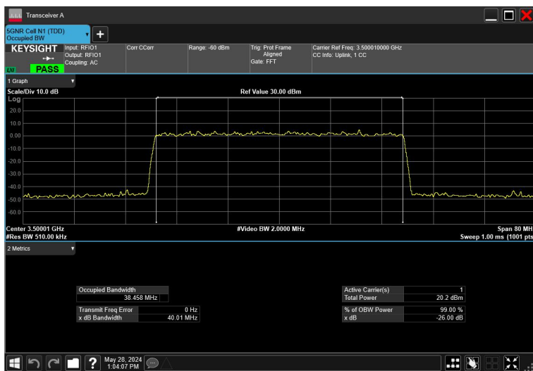
40MHz_15kHz_3500MHz_DFT-s-OFDM QPSK_RB216@0
