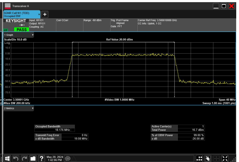
20MHz_30kHz_3500MHz_CP-OFDM 64QAM_RB51@0
