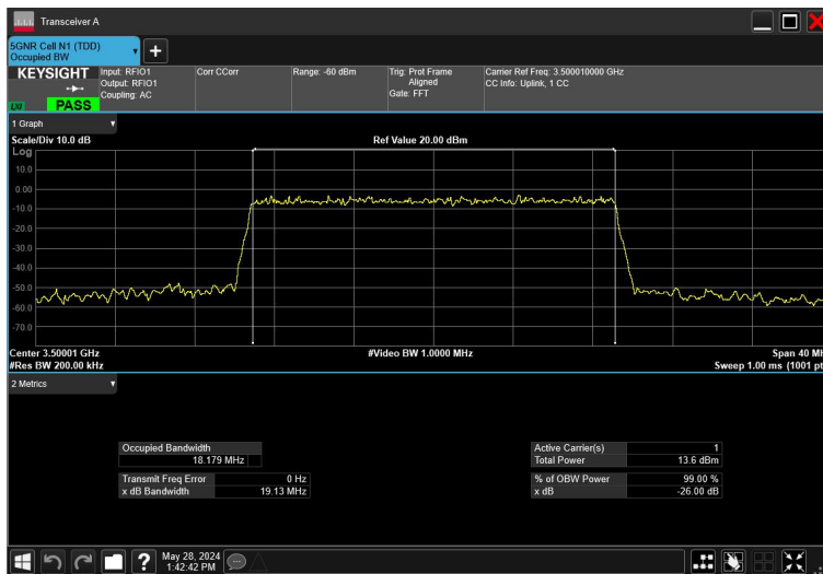
20MHz_30kHz_3500MHz_CP-OFDM 256QAM_RB51@0
