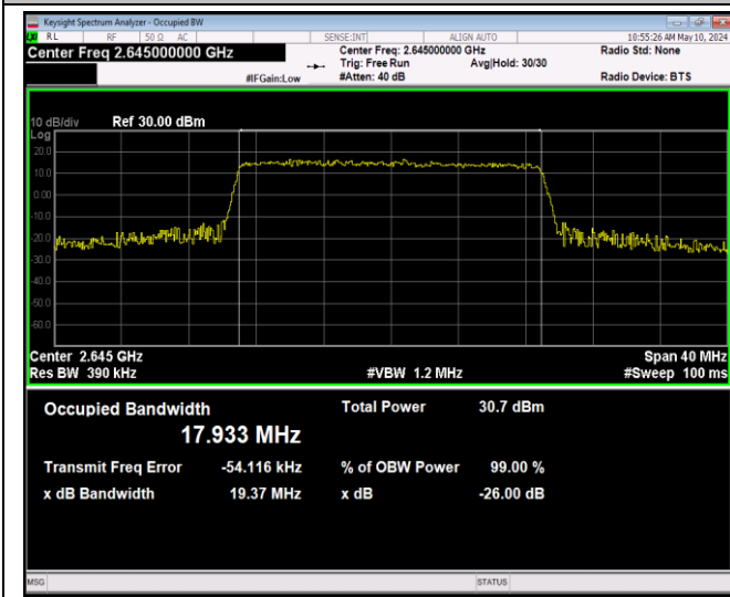
41(2535-2655)-20MHz-16QAM-41140-100RB#0-PASS
