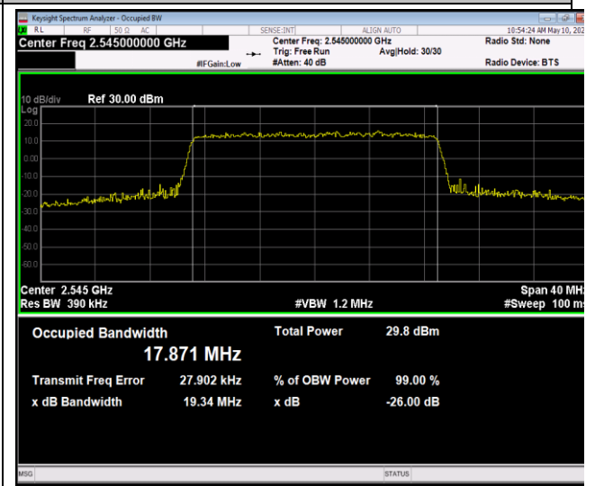
41(2535-2655)-20MHz-64QAM-40140-100RB#0-PASS
