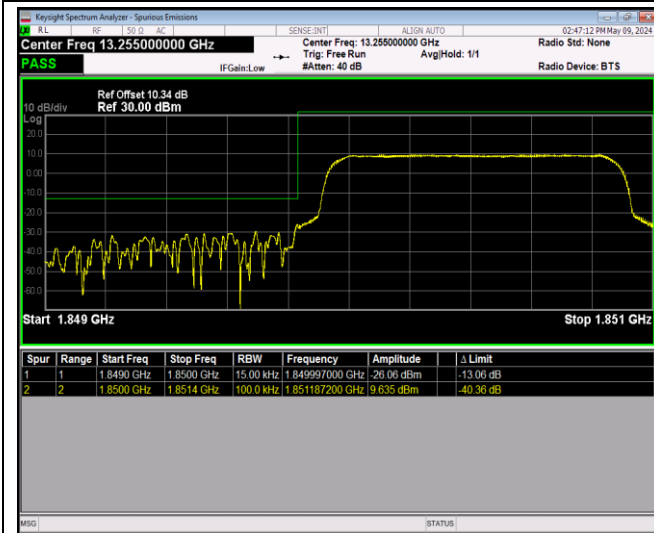
Band2_1.4MHz_QPSK_18607_6RB#0
