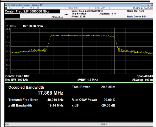
41(2535-2655)-20MHz-64QAM-41140-100RB#0-PASS
