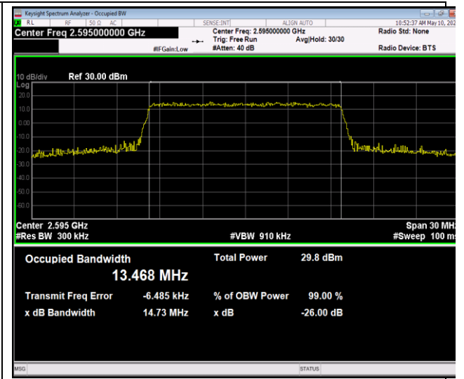
41(2535-2655)-15MHz-64QAM-40640-75RB#0-PASS
