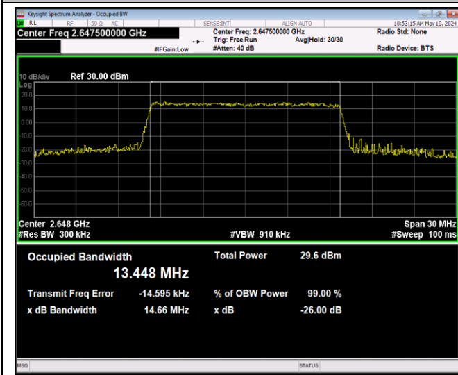
41(2535-2655)-15MHz-64QAM-41165-75RB#0-PASS
