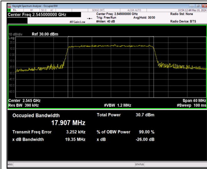
41(2535-2655)-20MHz-16QAM-40140-100RB#0-PASS
