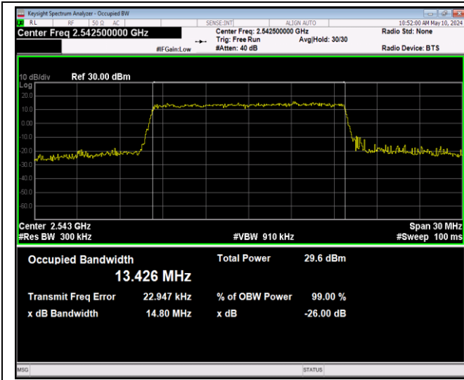
41(2535-2655)-15MHz-64QAM-40115-75RB#0-PASS
