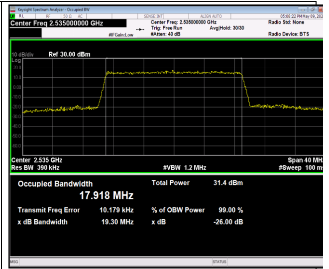
Band7-20MHz-16QAM-21100-100RB#0-PASS
