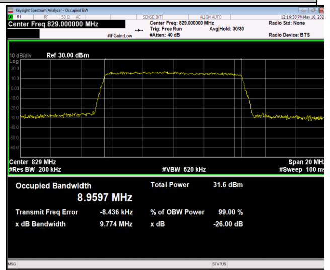
Band5-10MHz-QPSK-20450-50RB#0-PASS
