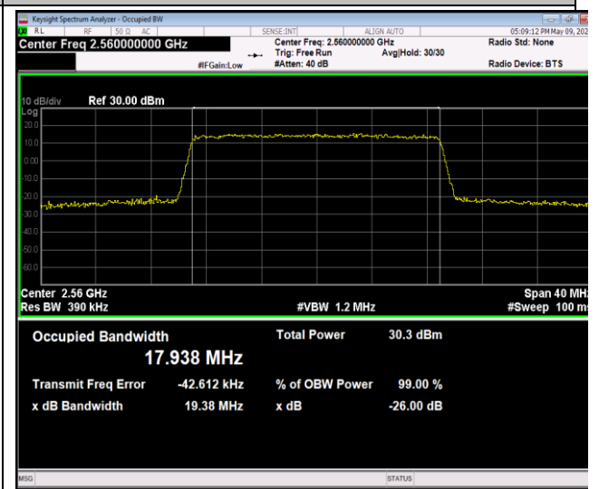
Band7-20MHz-64QAM-21350-100RB#0-PASS
