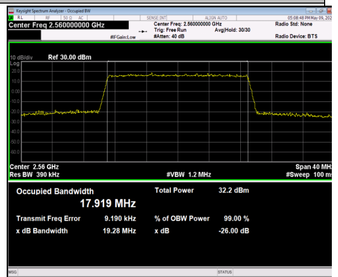
Band7-20MHz-QPSK-21350-100RB#0-PASS
