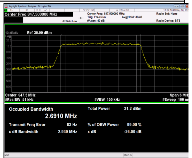
Band5-3MHz-QPSK-20635-15RB#0-PASS
