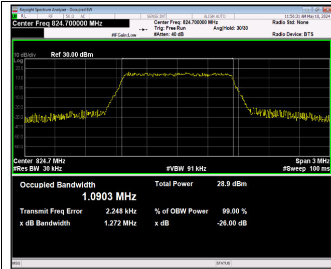
Band5-1.4MHz-64QAM-20407-6RB#0-PASS
