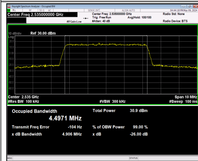
Band7-5MHz-16QAM-21100-25RB#0-PASS
