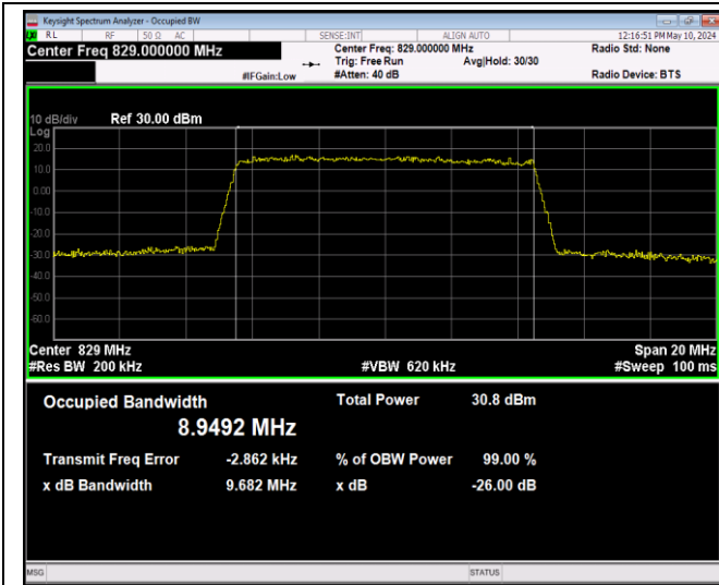
Band5-10MHz-16QAM-20450-50RB#0-PASS
