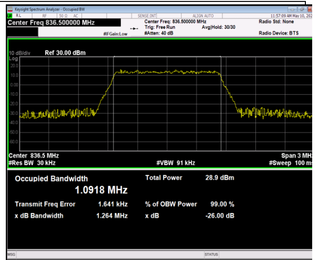
Band5-1.4MHz-64QAM-20525-6RB#0-PASS
