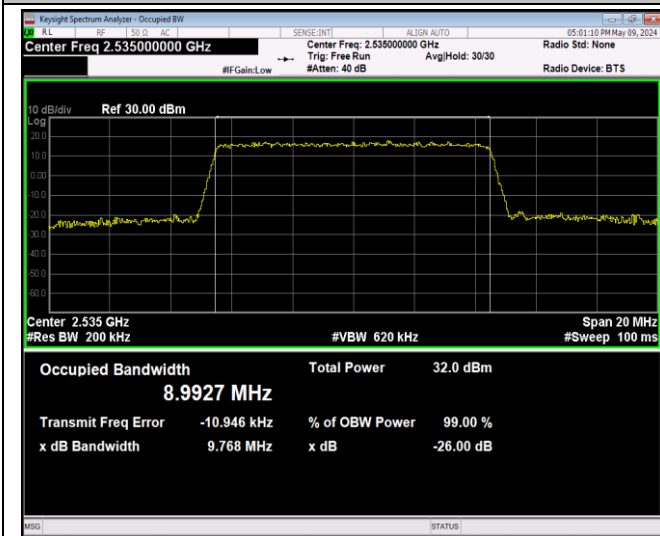
Band7-10MHz-QPSK-21100-50RB#0-PASS
