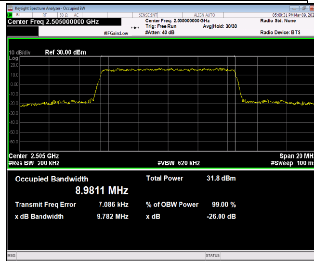
Band7-10MHz-QPSK-20800-50RB#0-PASS
