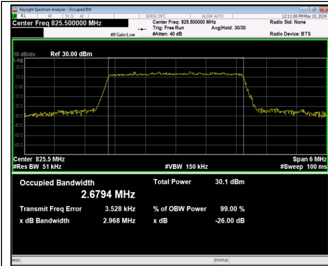
Band5-3MHz-16QAM-20415-15RB#0-PASS
