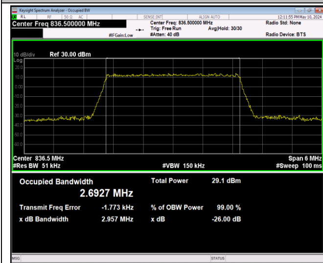
Band5-3MHz-64QAM-20525-15RB#0-PASS
