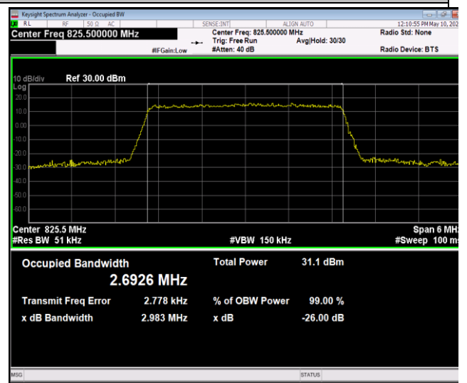
Band5-3MHz-QPSK-20415-15RB#0-PASS
