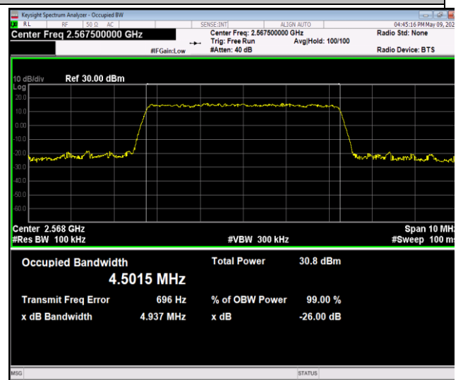
Band7-5MHz-16QAM-21425-25RB#0-PASS
