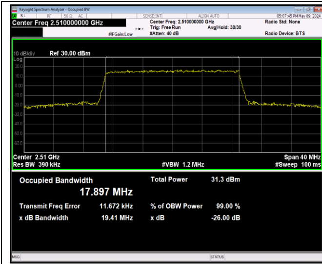
Band7-20MHz-16QAM-20850-100RB#0-PASS
