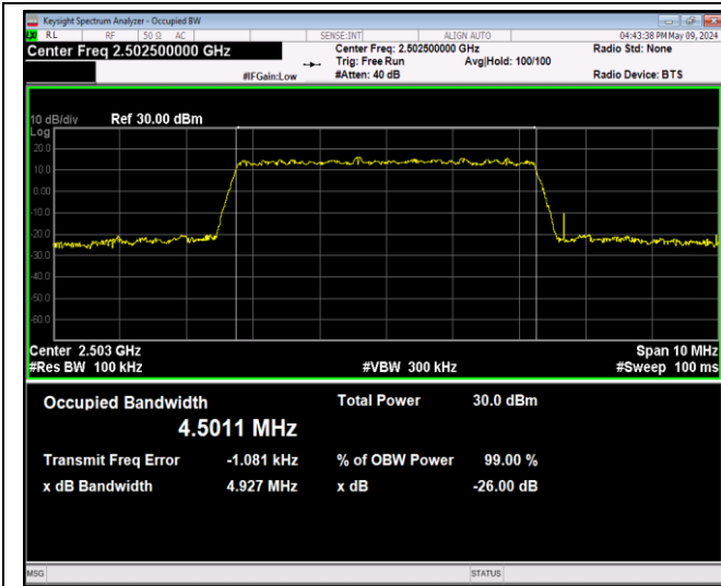
Band7-5MHz-64QAM-20775-25RB#0-PASS
