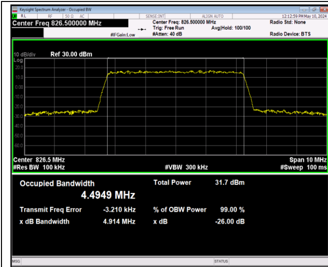
Band5-5MHz-QPSK-20425-25RB#0-PASS
