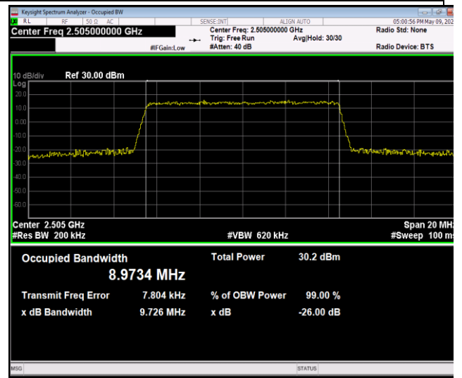
Band7-10MHz-64QAM-20800-50RB#0-PASS
