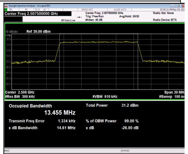
Band7-15MHz-16QAM-20825-75RB#0-PASS
