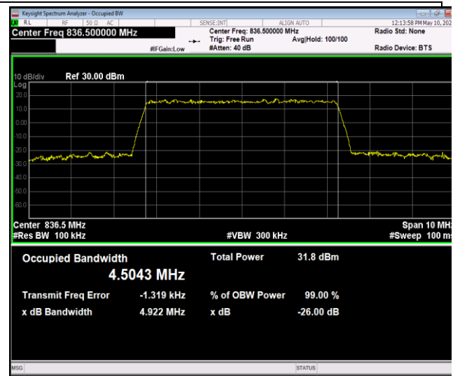
Band5-5MHz-QPSK-20525-25RB#0-PASS
