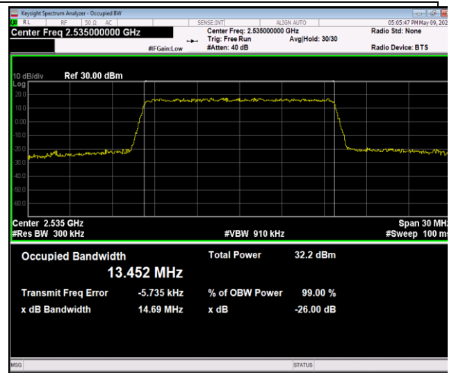
Band7-15MHz-QPSK-21100-75RB#0-PASS
