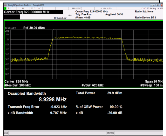
Band5-10MHz-64QAM-20450-50RB#0-PASS
