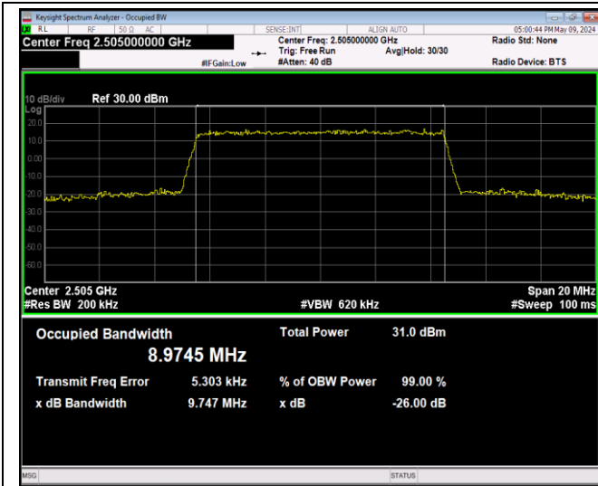
Band7-10MHz-16QAM-20800-50RB#0-PASS
