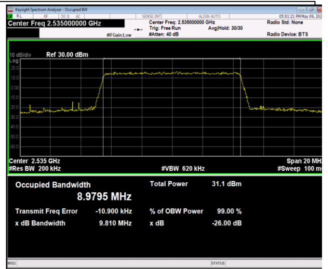
Band7-10MHz-16QAM-21100-50RB#0-PASS
