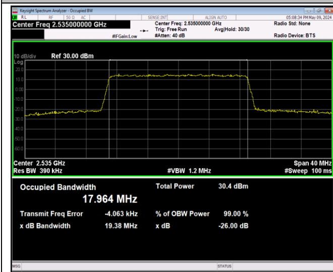
Band7-20MHz-64QAM-21100-100RB#0-PASS
