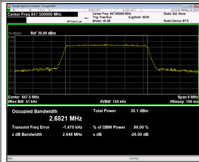
Band5-3MHz-16QAM-20635-15RB#0-PASS
