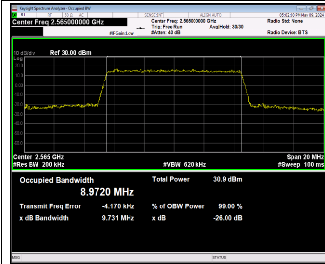
Band7-10MHz-16QAM-21400-50RB#0-PASS
