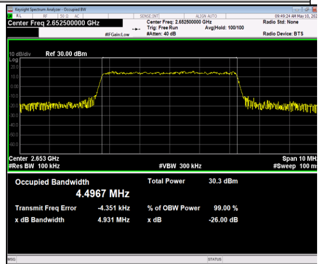
41(2535-2655)-5MHz-16QAM-41215-25RB#0-PASS
