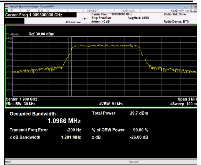
Band2-1.4MHz-16QAM-18607-6RB#0-PASS
