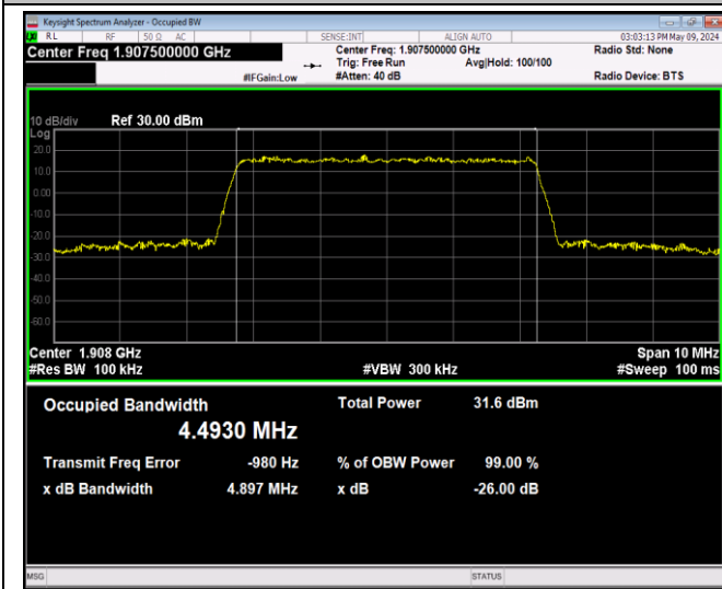
Band2-5MHz-QPSK-19175-25RB#0-PASS
