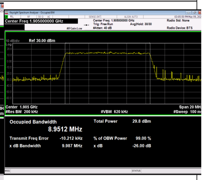
Band2-10MHz-64QAM-19150-50RB#0-PASS
