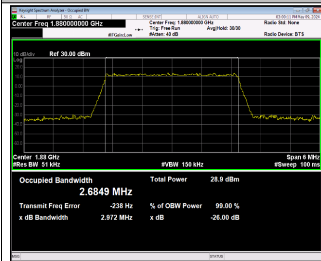
Band2-3MHz-64QAM-18900-15RB#0-PASS
