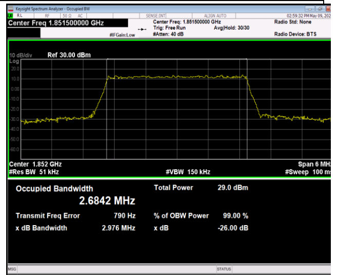
Band2-3MHz-64QAM-18615-15RB#0-PASS
