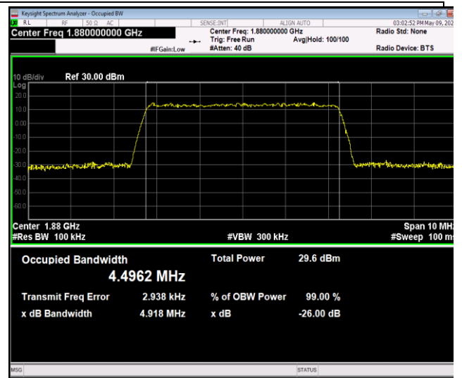
Band2-5MHz-64QAM-18900-25RB#0-PASS
