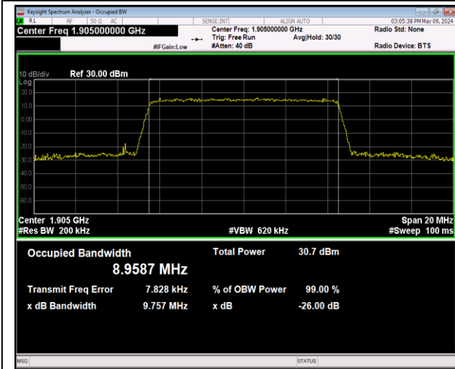
Band2-10MHz-16QAM-19150-50RB#0-PASS
