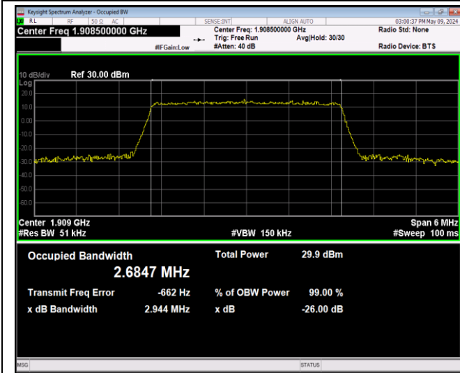
Band2-3MHz-16QAM-19185-15RB#0-PASS
