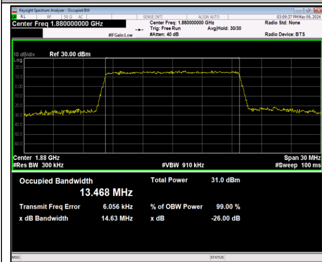
Band2-15MHz-16QAM-18900-75RB#0-PASS
