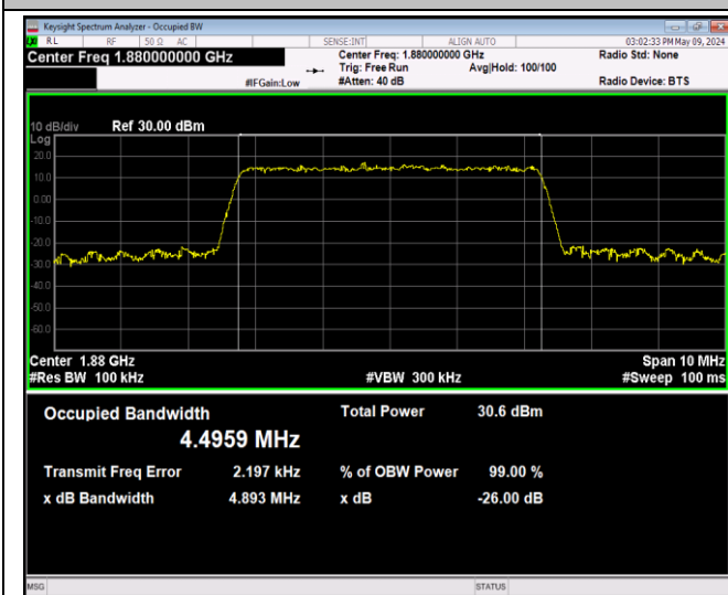
Band2-5MHz-16QAM-18900-25RB#0-PASS
