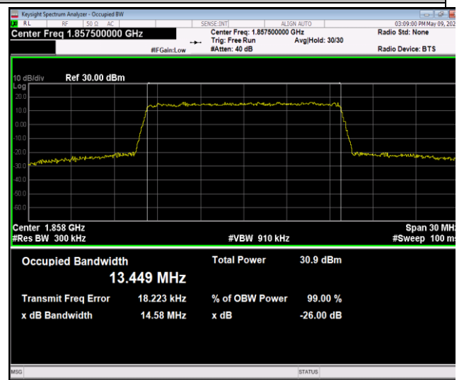
Band2-15MHz-16QAM-18675-75RB#0-PASS
