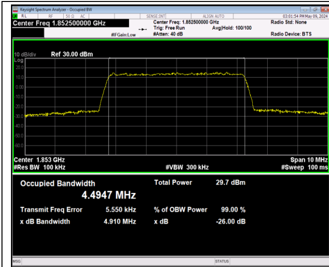
Band2-5MHz-64QAM-18625-25RB#0-PASS
