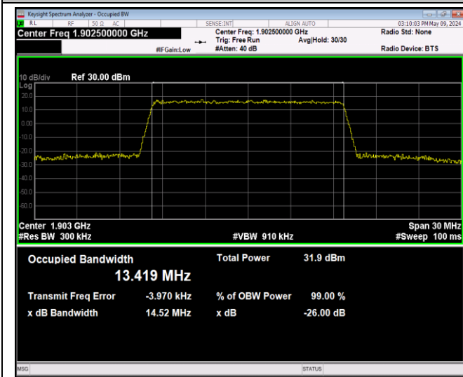
Band2-15MHz-QPSK-19125-75RB#0-PASS
