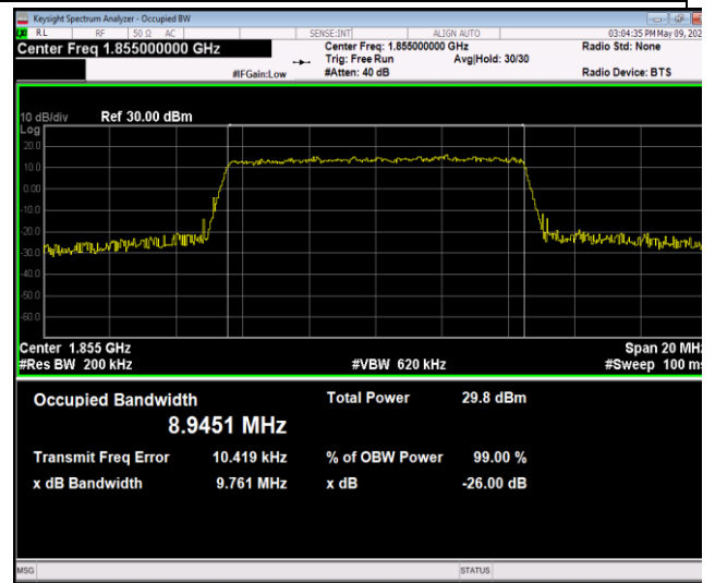
Band2-10MHz-64QAM-18650-50RB#0-PASS
