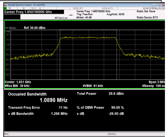
Band2-1.4MHz-16QAM-18607-6RB#0-PASS
