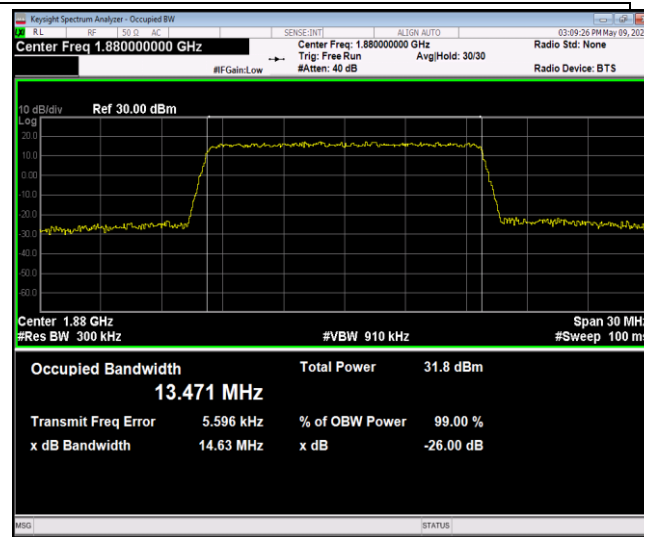
Band2-15MHz-QPSK-18900-75RB#0-PASS
