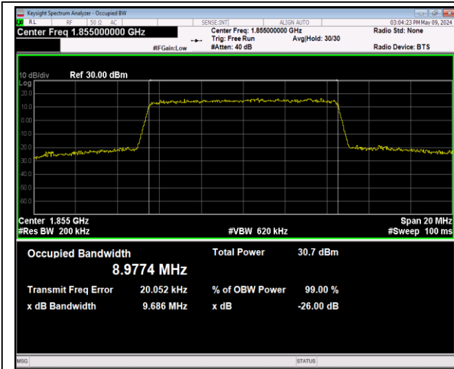
Band2-10MHz-16QAM-18650-50RB#0-PASS
