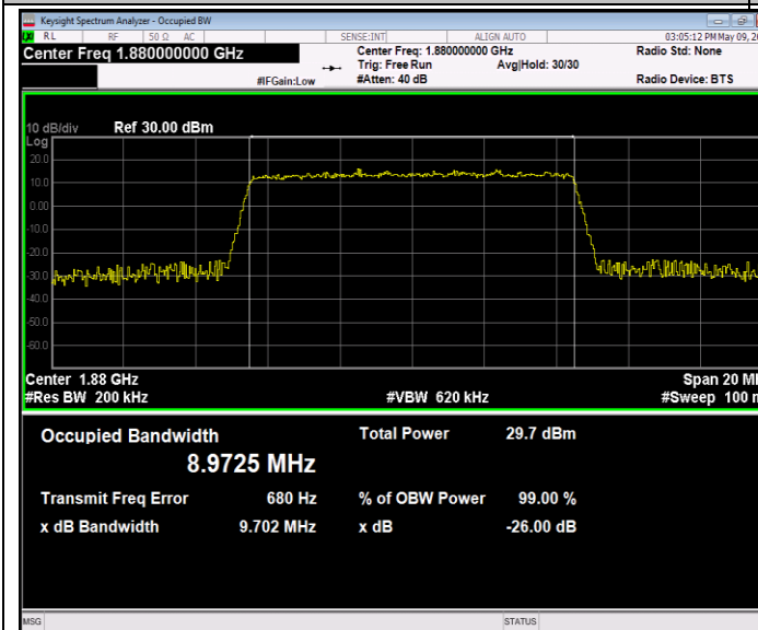
Band2-10MHz-64QAM-18900-50RB#0-PASS
