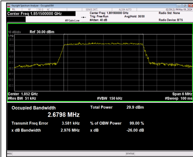
Band2-3MHz-16QAM-18615-15RB#0-PASS
