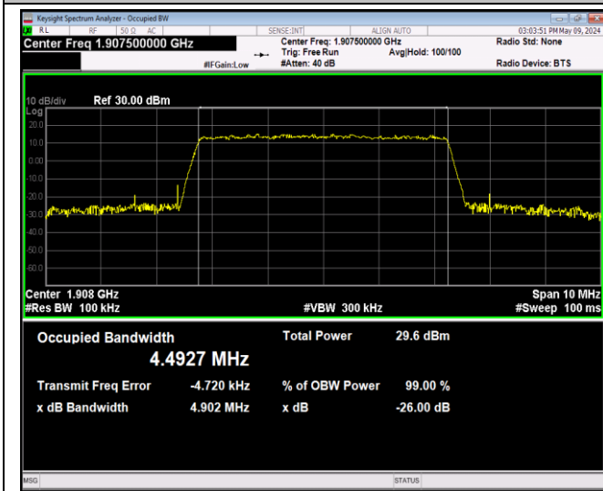
Band2-5MHz-64QAM-19175-25RB#0-PASS
