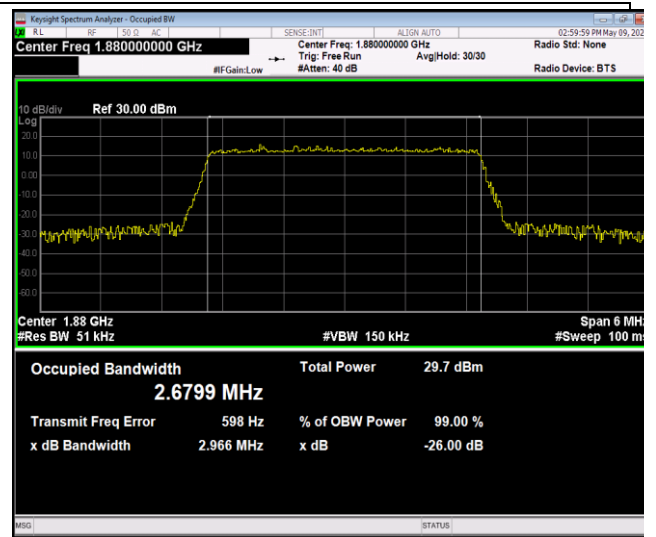
Band2-3MHz-16QAM-18900-15RB#0-PASS
