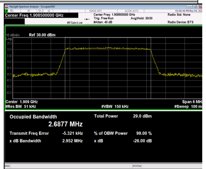
Band2-3MHz-64QAM-19185-15RB#0-PASS
