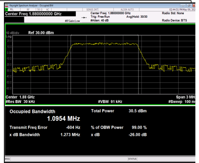
Band2-1.4MHz-QPSK-18900-6RB#0-PASS
