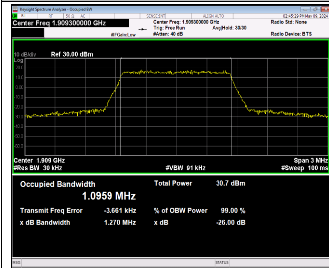
Band2-1.4MHz-QPSK-19193-6RB#0-PASS
