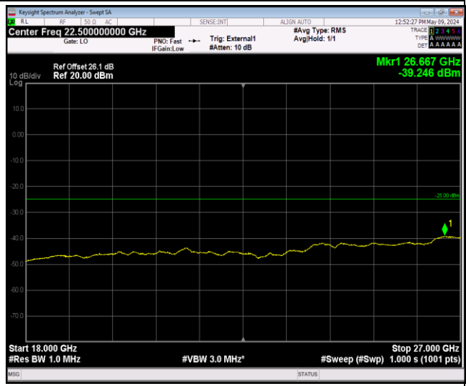
Band41_20MHz_QPSK_41140_1RB#0_18000~27000_18000~27000
