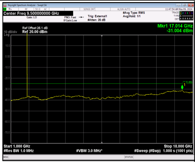
Band41_5MHz_64QAM_40065_1RB#0_1000~18000_100 0~18000
