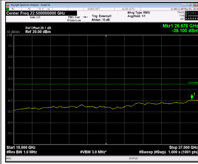
Band41_5MHz_64QAM_40065_1RB#0_18000~27000_18
