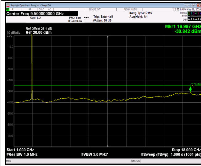
Band41_20MHz_QPSK_41140_1RB#0_1000~18000_1000~18000
