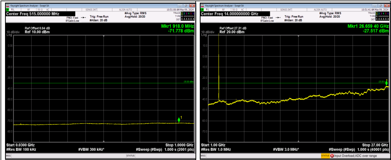
Band7_20MHz_QPSK_21100_1RB#0_1000~27000_1000~27000
