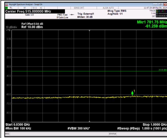
Band41_5MHz_64QAM_40065_1RB#0_30~1000_30~100 0
