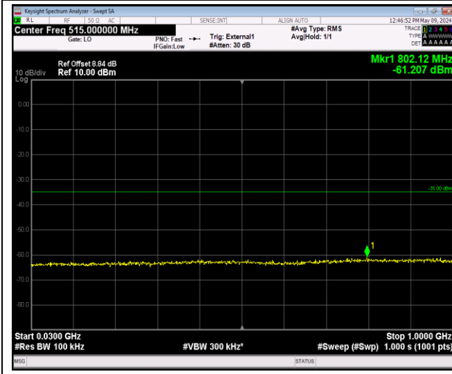
Band41_20MHz_16QAM_40140_1RB#0_30~1000_30~1000
