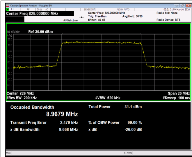
Band5-10MHz-16QAM-20450-50RB#0-PASS
