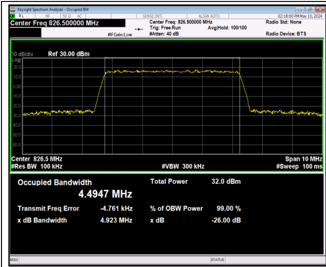
Band5-5MHz-QPSK-20425-25RB#0-PASS
