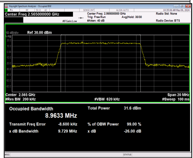
Band7-10MHz-QPSK-21400-50RB#0-PASS
