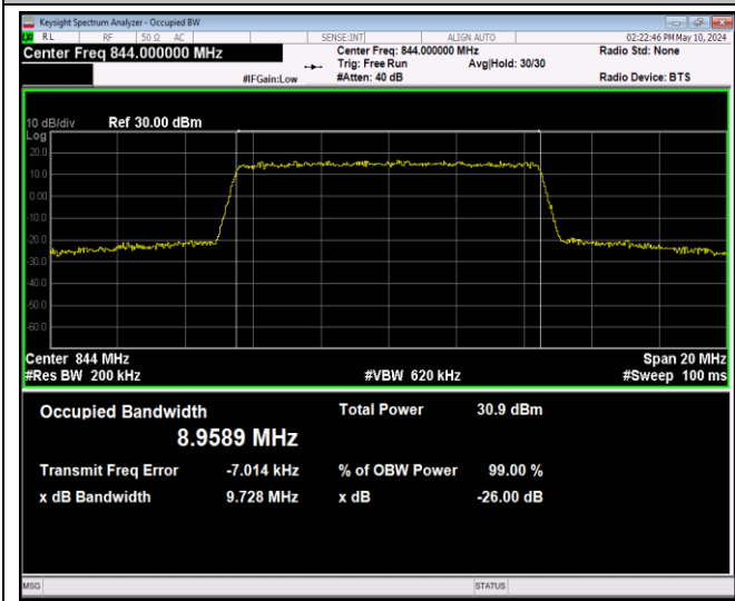
Band5-10MHz-16QAM-20600-50RB#0-PASS
