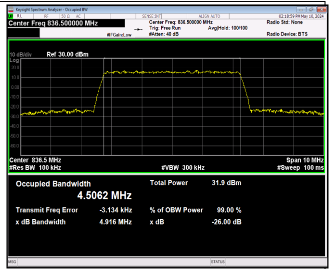
Band5-5MHz-QPSK-20525-25RB#0-PASS
