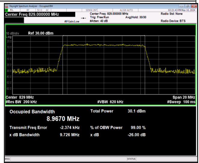
Band5-10MHz-64QAM-20450-50RB#0-PASS
