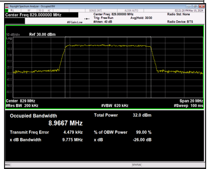
Band5-10MHz-QPSK-20450-50RB#0-PASS
