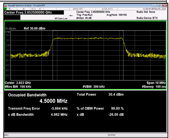
41(2535-2655)-5MHz-16QAM-41215-25RB#0-PASS
