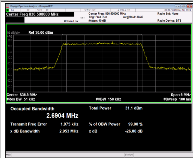
Band5-3MHz-QPSK-20525-15RB#0-PASS
