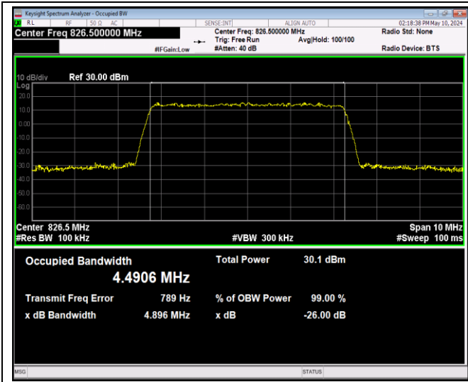
Band5-5MHz-64QAM-20425-25RB#0-PASS
