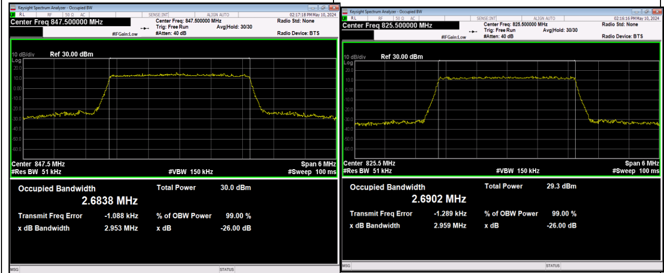
Band5-3MHz-16QAM-20635-15RB#0-PASS
