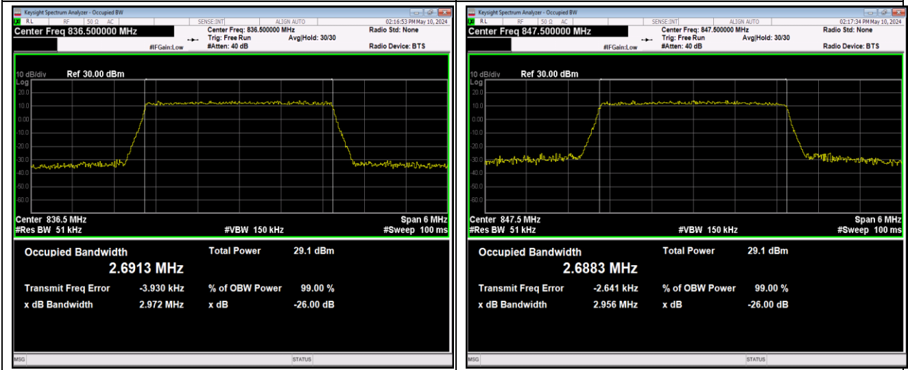
Band5-3MHz-64QAM-20525-15RB#0-PASS
