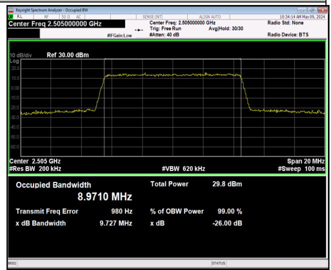
Band7-10MHz-64QAM-20800-50RB#0-PASS
