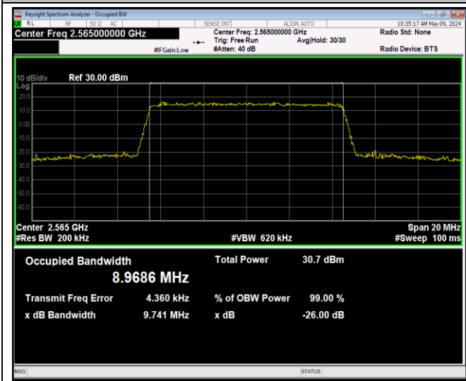
Band7-10MHz-16QAM-21400-50RB#0-PASS
