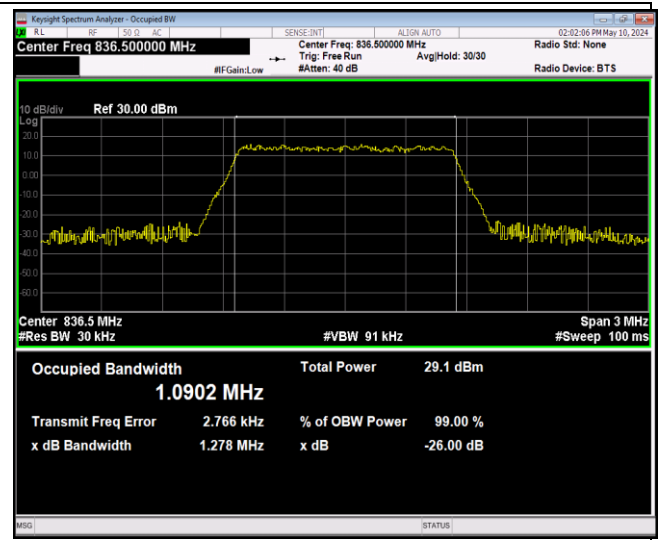
Band5-1.4MHz-64QAM-20525-6RB#0-PASS
