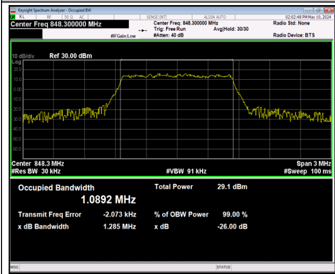
Band5-1.4MHz-64QAM-20643-6RB#0-PASS
