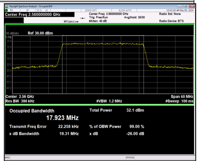
Band7-20MHz-QPSK-21350-100RB#0-PASS
