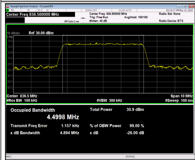
Band5-5MHz-16QAM-20525-25RB#0-PASS
