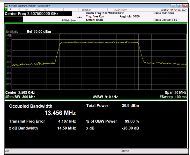
Band7-15MHz-16QAM-20825-75RB#0-PASS
