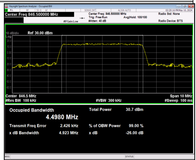
Band5-5MHz-16QAM-20625-25RB#0-PASS
