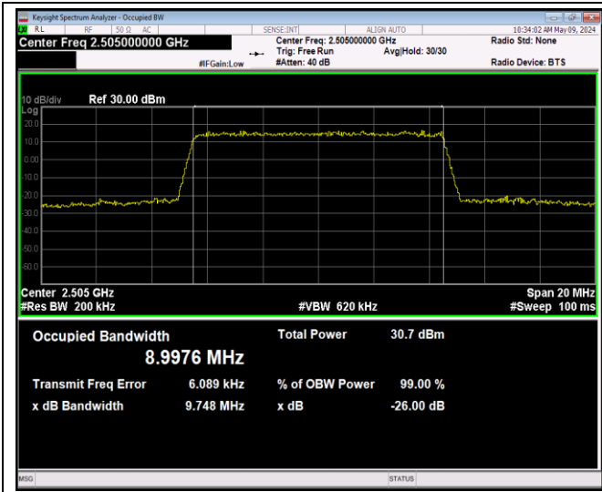
Band7-10MHz-16QAM-20800-50RB#0-PASS
