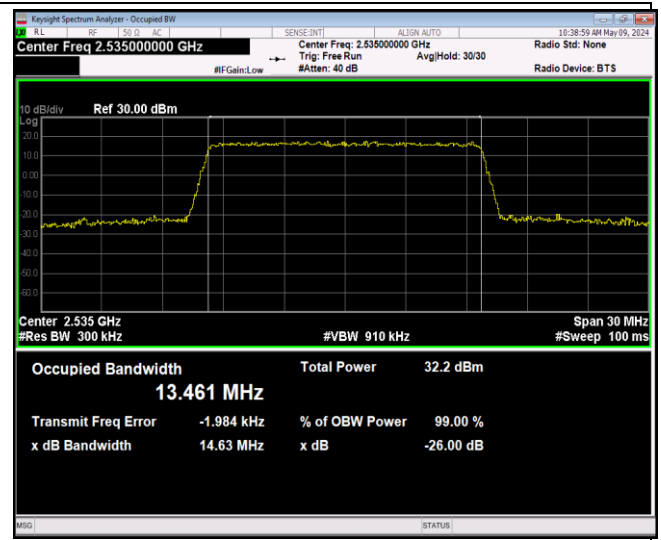
Band7-15MHz-QPSK-21100-75RB#0-PASS
