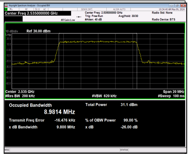
Band7-10MHz-16QAM-21100-50RB#0-PASS
