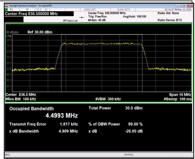
Band5-5MHz-64QAM-20525-25RB#0-PASS
