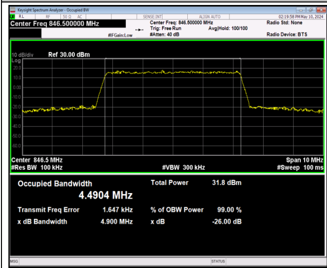
Band5-5MHz-QPSK-20625-25RB#0-PASS
