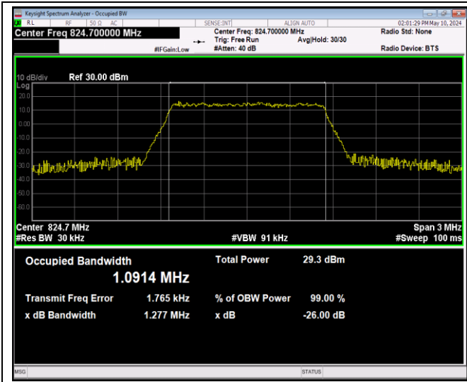
Band5-1.4MHz-64QAM-20407-6RB#0-PASS
