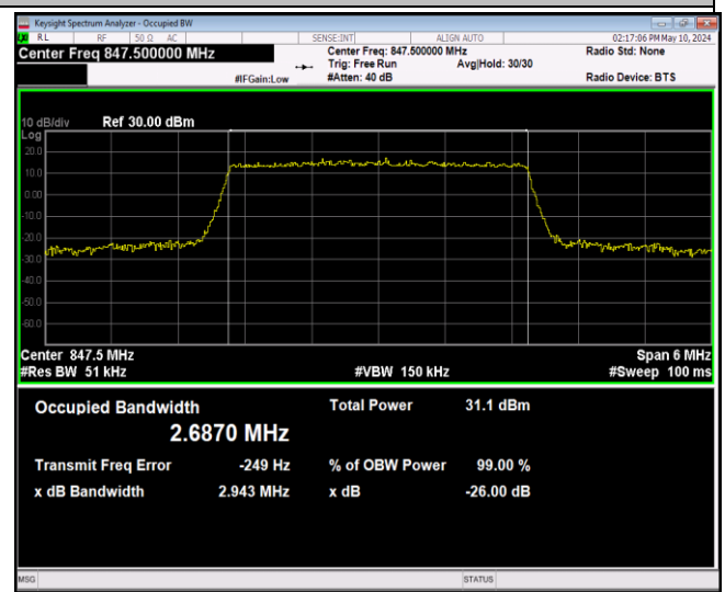
Band5-3MHz-QPSK-20635-15RB#0-PASS
