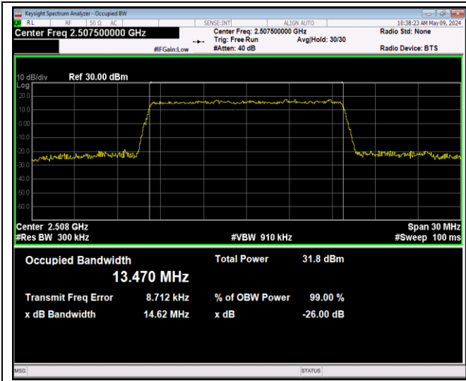
Band7-15MHz-QPSK-20825-75RB#0-PASS
