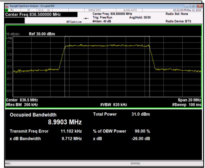
Band5-10MHz-16QAM-20525-50RB#0-PASS
