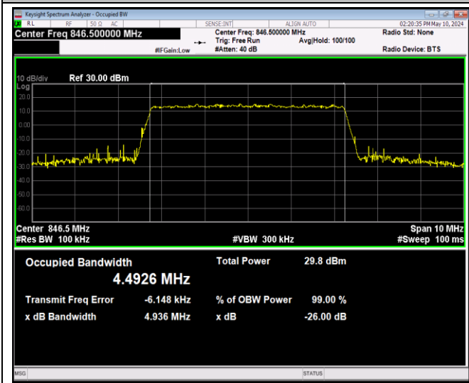
Band5-5MHz-64QAM-20625-25RB#0-PASS
