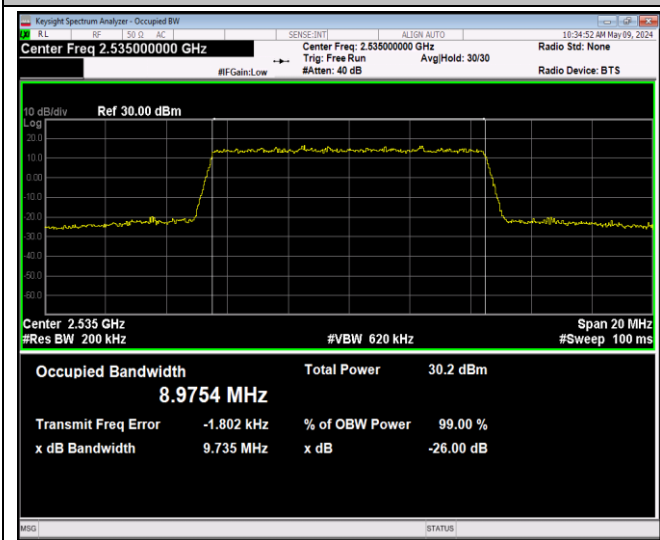
Band7-10MHz-64QAM-21100-50RB#0-PASS
