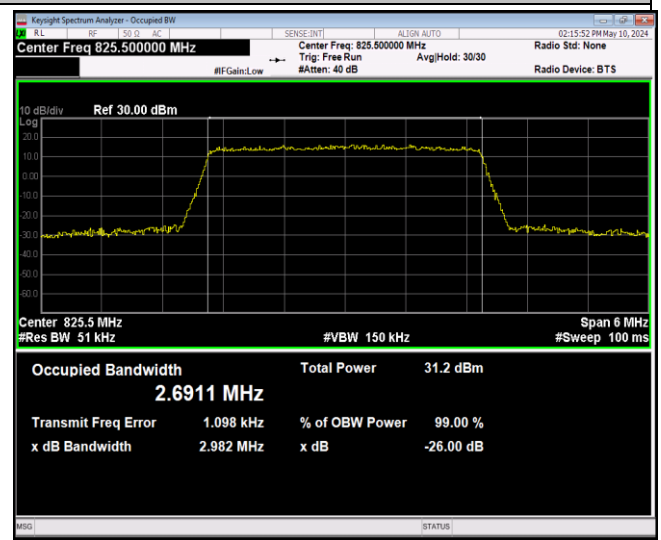
Band5-3MHz-QPSK-20415-15RB#0-PASS
