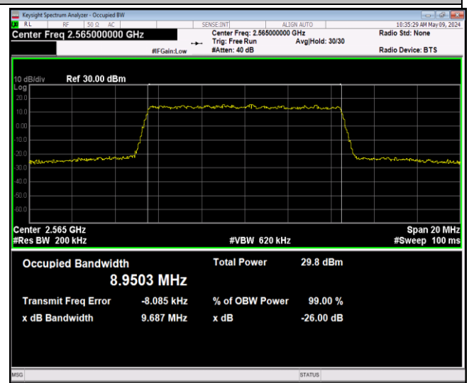
Band7-10MHz-64QAM-21400-50RB#0-PASS
