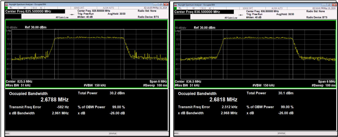
Band5-3MHz-16QAM-20415-15RB#0-PASS
