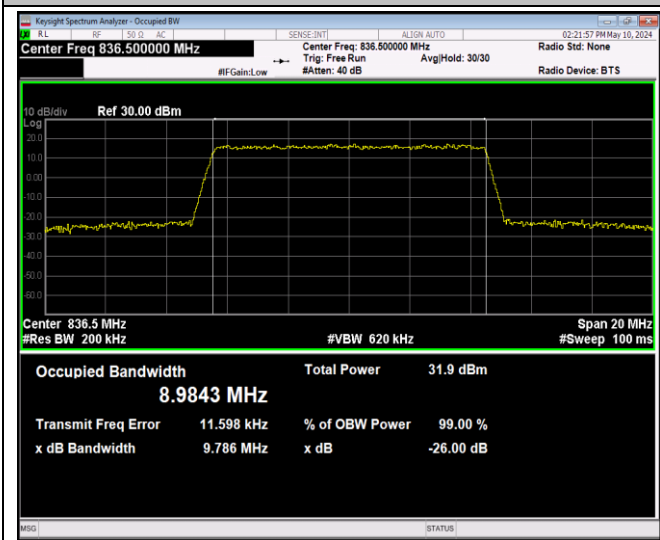
Band5-10MHz-QPSK-20525-50RB#0-PASS
