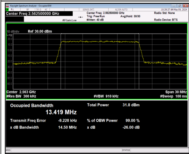
Band7-15MHz-QPSK-21375-75RB#0-PASS
