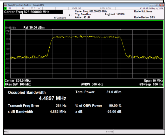
Band5-5MHz-16QAM-20425-25RB#0-PASS
