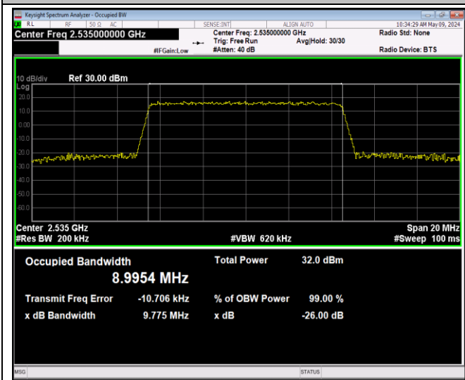
Band7-10MHz-QPSK-21100-50RB#0-PASS
