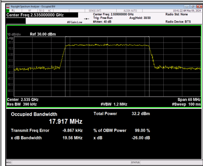
Band7-20MHz-QPSK-21100-100RB#0-PASS
