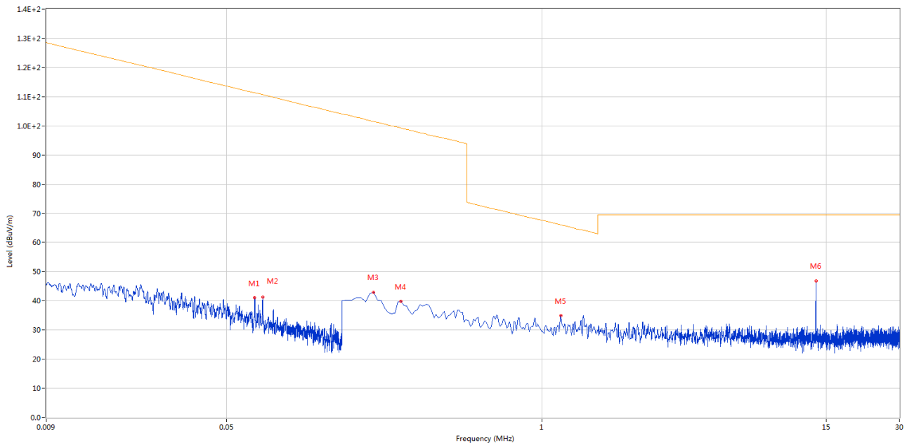
Below 30 MHz, Test Antenna LOOP, EUT X axis
