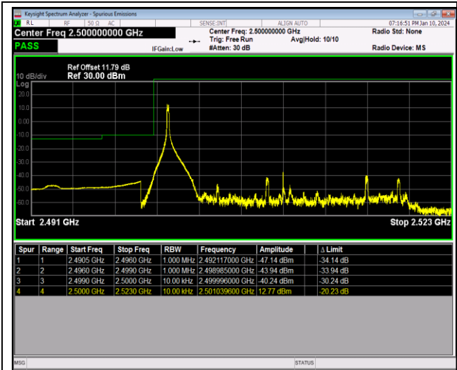
Band7-20MHz-QPSK-20850-100RB#0
