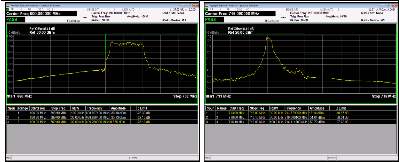
Band12-1.4MHz-64QAM-23173-1RB#5
