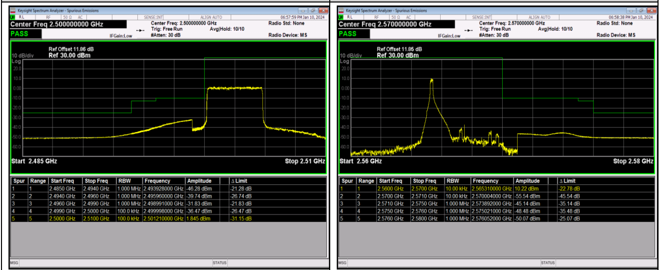
Band7-5MHz-64QAM-21425-1RB#24
