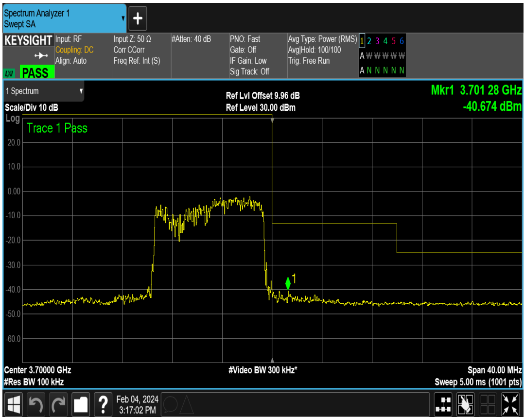
n77(3550-3700) SCS=30kHz DFT_QPSK BW=10MHz Channel=646332 RB=1@23
